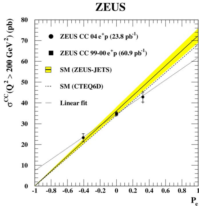
Fig. 3. The total cross section for e^+p CC DIS with Q^2 > 200 \text{ GeV}^2 as a function of the longitudinal polarisation of the positron beam. The full (dashed) line shows the prediction of the SM evaluated using the ZEUS-JETS (CTEQ6D) PDFs and the shaded band indicates the uncertainty on the cross section from the ZEUS-JETS fit. The dotted line shows the result of the linear fit to the data described in the text. Horizontal error bars representing the uncertainty on the measured polarisation are included but are too small to be visible.
