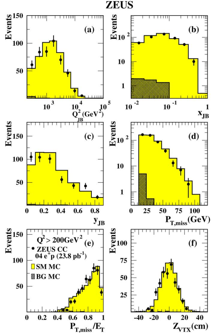
Fig. 1. Comparison of the final e^+p CC data sample (solid points) with the sum of the signal and background MC simulations (light shaded histograms). The simulated background events are shown as the dark shaded histograms. The distributions of (a) Q_{\text{JB}}^2 , (b) x_{\text{JB}} , (c) y_{\text{JB}} , (d) P_{\text{T,miss}} , (e) P_{\text{T,miss}}/E_T and (f) Z_{\text{VTX}} , are shown.
