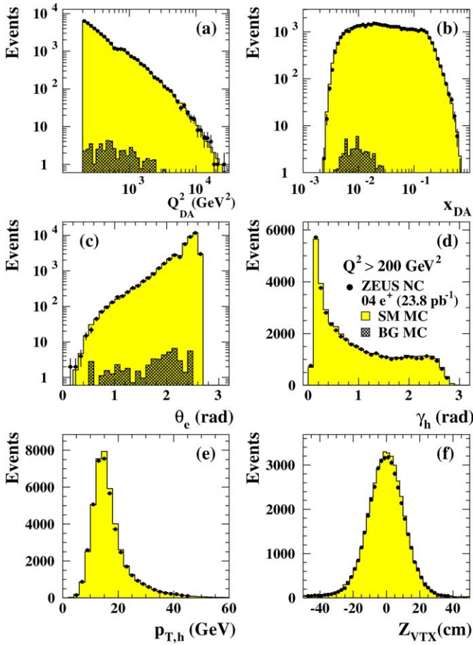
Fig. 2. Comparison of the final e^+p NC data sample (solid points) with the sum of the signal and background MC simulations (light shaded histograms). The simulated background events are shown as the dark shaded histograms. The distributions of (a) Q^2_{DA} , (b) x_{DA} , (c) \theta_e , (d) \gamma_h , (e) p_{T,h} , and (f) Z_{VTX} , are shown.
