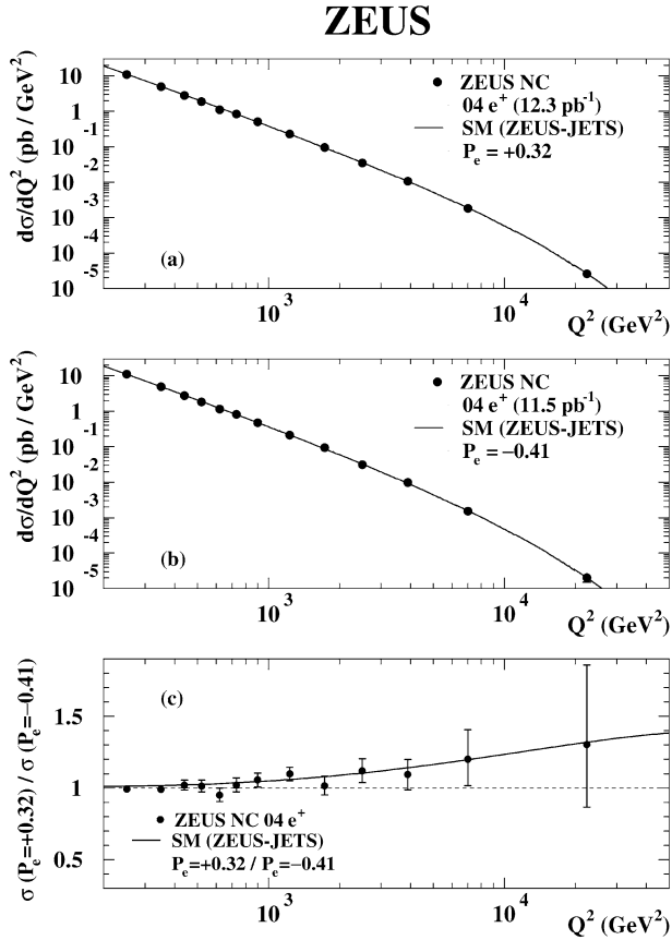
Fig. 5. The e^+p NC DIS cross section d\sigma/dQ^2 for (a) positive polarisation data, (b) negative polarisation data and (c) the ratio of the two. The full lines show the predictions of the SM evaluated using the ZEUS-JETS PDFs and the dashed line the prediction with no dependence on the longitudinal polarisation of the positron beam.
