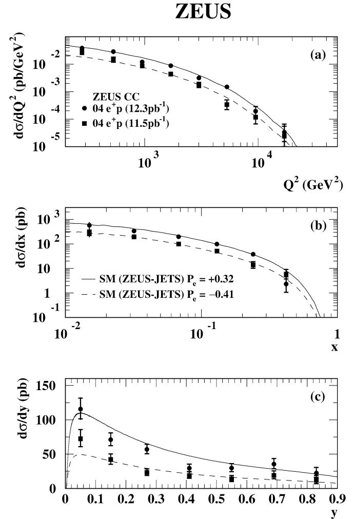
Fig. 4. The e^+p CC DIS cross-sections (a) d\sigma/dQ^2 , (b) d\sigma/dx and (c) d\sigma/dy . The circles (squares) represent data points for the positive (negative) polarisation measurements and the curves show the predictions of the SM evaluated using the ZEUS-JETS PDFs.
