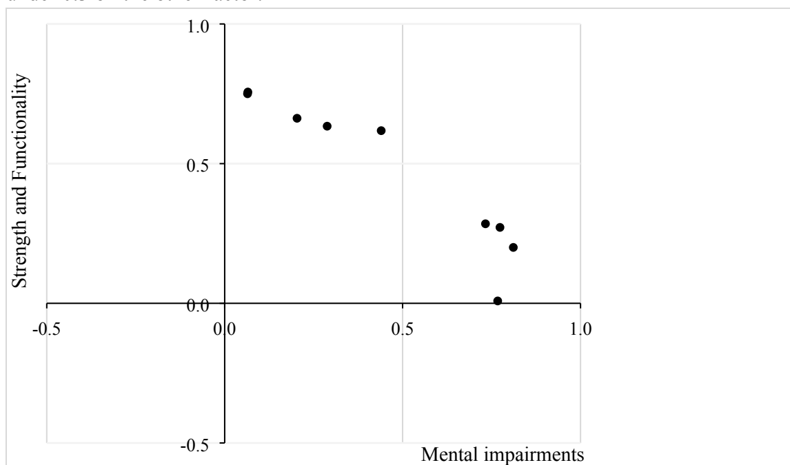
Figure 5. Factor loadings of the nine impairment items on the Mental impairments factor and Strength and Functionality factor
