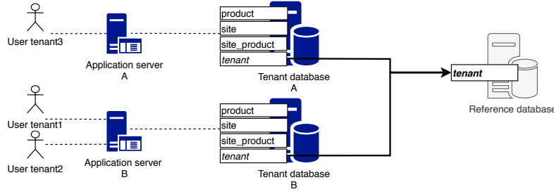
Fig. 3. Multi-tenant stock management application: table placement.
