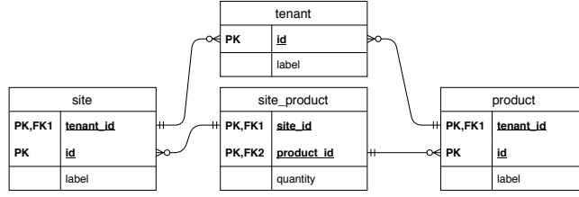
Fig. 1. Multi-tenant stock management application: Entity-Relation schema.
