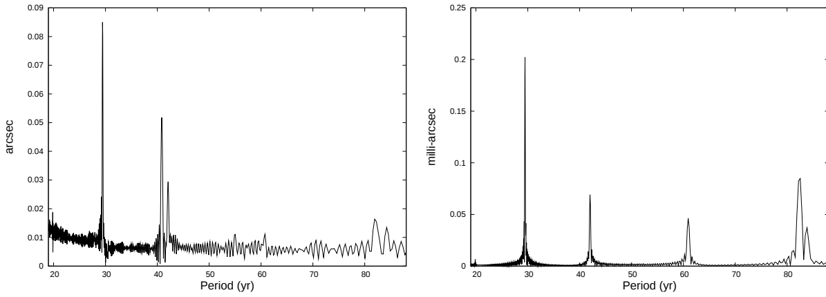
Figure 4.6: Fourier spectra of the residuals of the frequency analysis, for the longitudinal librations (left), and for the latitudinal librations, both in the Model 2 (i.e. 10000-term ephemerides). Here, only the contributions with periods between 18 and 90 years is plotted. The Fourier spectra for Models 1/1b do not give significant information in this range.
