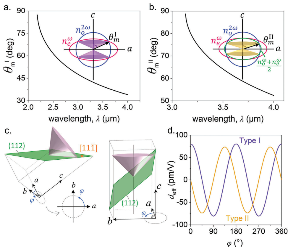
Figure 5. a) Type I and b) Type II phase-matching angles of \text{MgSiP}_2 at various fundamental wavelengths. c) Definition of the phase matching angle \theta_m and azimuthal angle \varphi . d) d_{\text{eff}} for Type I and Type II phase-matching conditions of \text{MgSiP}_2 versus the azimuthal angle \varphi .
