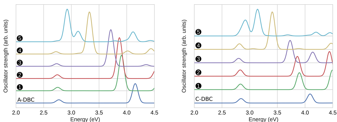
Figure 5. Computed absorption spectra for the angular (left) and compact (right) DBCs with substituents at R3 and R4 positions: the angular and compact DBCs are at the bottom in blue, next from bottom to top, the modified DBCs with groups from 1 to 5 (Figure 1d) are plotted.
