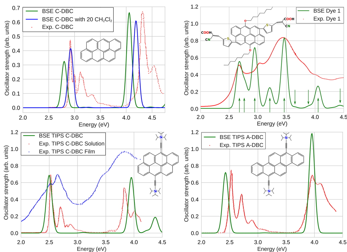
Figure 2. Comparison between experimental (red) and computed (green) absorption spectra for the C-DBC (upper left), Dye 1 (upper right), TIPS-C-DBC (lower left, C-R1R2-8), and TIPS-A-DBC (lower right, A-R1R2-8). The experimental spectra are from refs 40, 19, 12, and 17, respectively. In the upper left graph, the absorption spectrum for C-DBC with a first solvation shell of \text{CH}_2\text{Cl}_2 is plotted in blue. In the lower left graph, the absorption spectrum of a thin film TIPS-C-DBC is plotted in blue. In the upper right graph, the nine theoretical absorption peaks (1–9 from left to right) are indicated with green arrows.
