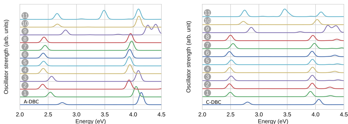
Figure 4. Computed absorption spectra for the angular (left) and compact (right) DBCs with substituents at R1 and R2 positions: the angular and compact DBCs are at the bottom in blue, next from bottom to top, the modified compact DBCs with groups from 1 to 11 (Figure 1c) are plotted.
