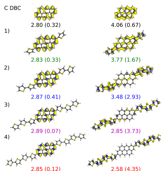
Figure 9. Hole-averaged electronic (in yellow) and electron-averaged hole (in wireframed blue) densities of the excitonic states for the molecules illustrated in Figure 8. Left column: exciton localized on the backbone DBC. Right column: exciton localized on the thiophenyl groups. For each exciton, its energy level and, between parentheses, its oscillator strength (in arb. units) are reported below the corresponding densities.
