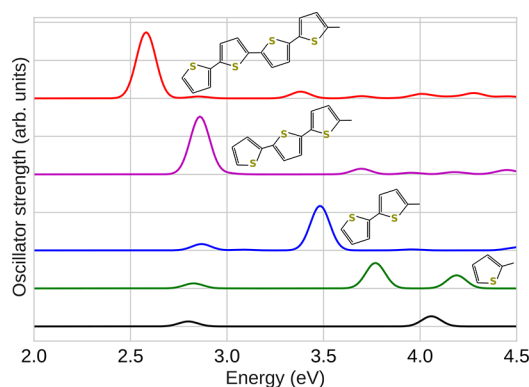
Figure 8. Computed absorption spectra for compact DBC (black curve) and for functionalized compact DBCs with 1 (green), 2 (blue), 3 (violet), and 4 (red) thiophenyl groups attached at R3 and R4 positions.
