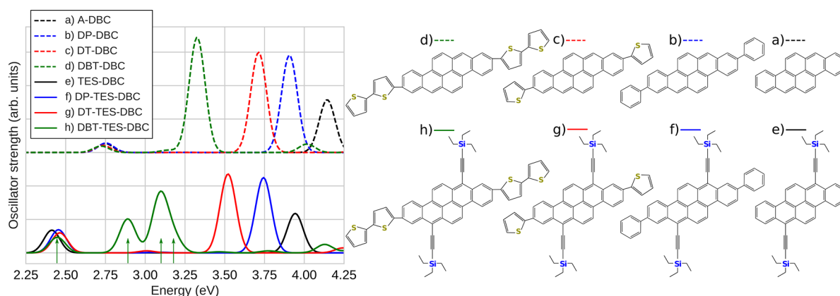
Figure 6. Computed absorption spectra for different angular DBC molecules. For the DBT-TES-DBC, the four absorption peaks (1–4 from left to right) are indicated with green arrows.
