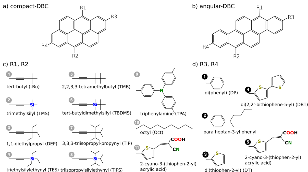
Figure 1. Illustration of the compact (a) and angular (b) dibenzochrysenes. Various functional groups with their nomenclature attached at R1 and R2 positions (c) and at R3 and R4 positions (d).
