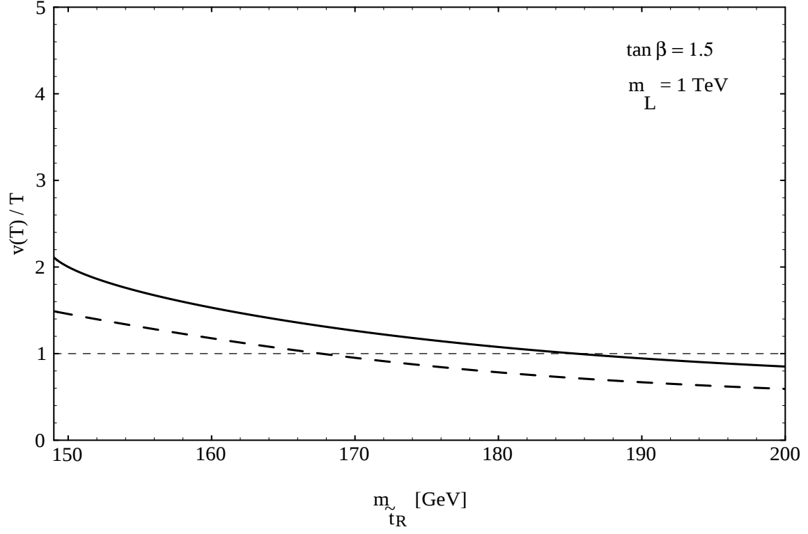
Figure 1: Dependence of the ratios v(T_0)/T_0 (solid line) and v(T_1)/T_1 (bold-dashed line) on the right-handed stop mass m_{\tilde{t}_R} for the particular values of \tan \beta = 1.5 , m_L = 1 TeV and m_t = 174 GeV.
