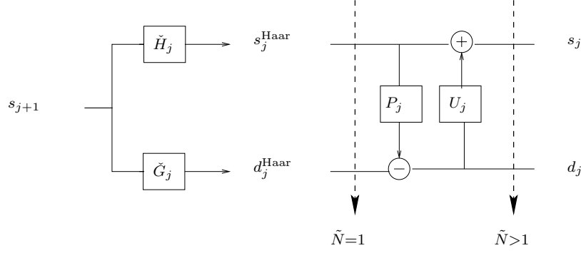
Figure 3: Filter bank diagram for our analysing wavelet transform. A Haar transform is performed first, producing detail and scaling coefficients corresponding to the initialisation wavelet basis of order \tilde{N} = 1 . This basis is further improved by two lifting steps: the predict operator P_j produces detail coefficients with better approximation properties, the update operator U_j stabilizes the transform.
