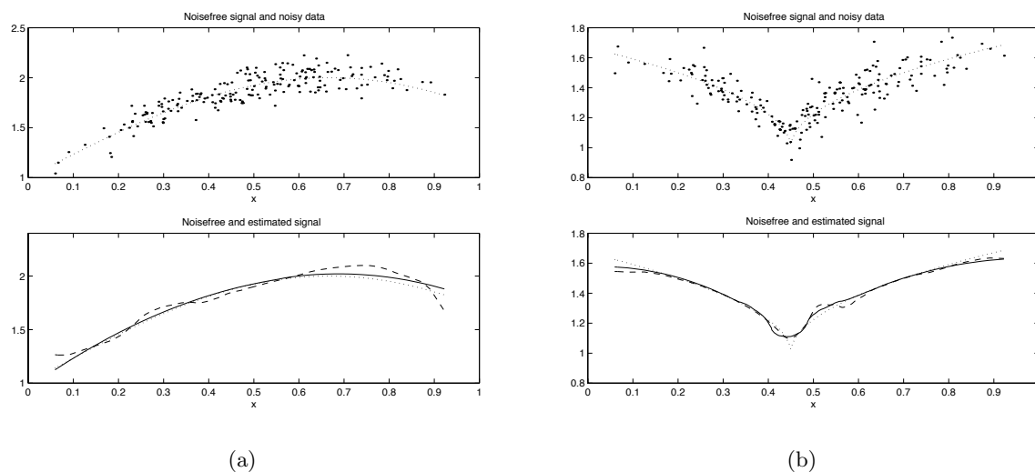
Figure 5: Estimation of the Sine (a) and Cusp (b) functions with the one-step algorithm. Data are represented by dots and the underlying signal by a dotted line. The WAI estimator with update is represented as a plain line, the estimator from interpolation as a dashed line. The RMSE values for the WAI and interpolation methods, respectively, are equal to 0.94% and 2.92% in (a), and 1.83% and 2.00% in (b).
