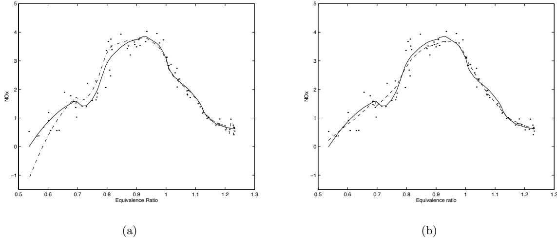
Figure 8: The ethanol data set is represented in dots. In (a) the WAI estimator with (plain line) and without (interrupted dashed line) update resulting from the three-step procedure is shown. In (b) the WAI estimator with update (plain line) is represented together with the k -nearest neighbour linear least squares, using cross-validation for a local choice of k (dashed line).
