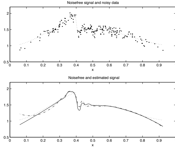
Figure 6: Estimation of the Jump function with the three-step algorithm in case of correlated errors. The dotted line represents the underlying signal. The WAI estimators with and without update are plotted in continuous and in dashed line, respectively. The RMSE equals 3.39% for the estimator with update and 4.19% without update.
