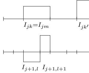
Figure 1: Coarsening procedure when n is not a power of two. At the level j = 4 , we combine the 14 intervals two by two to produce 7 intervals at level j = 3 . The first 6 intervals are further combined to produce the first three intervals at the coarser level, the last interval being passed unchanged to the level j = 2 .
