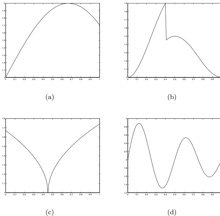
Figure 4: Test functions: (a) Sine (b) Jump (c) Cusp (d) Damped Sine
