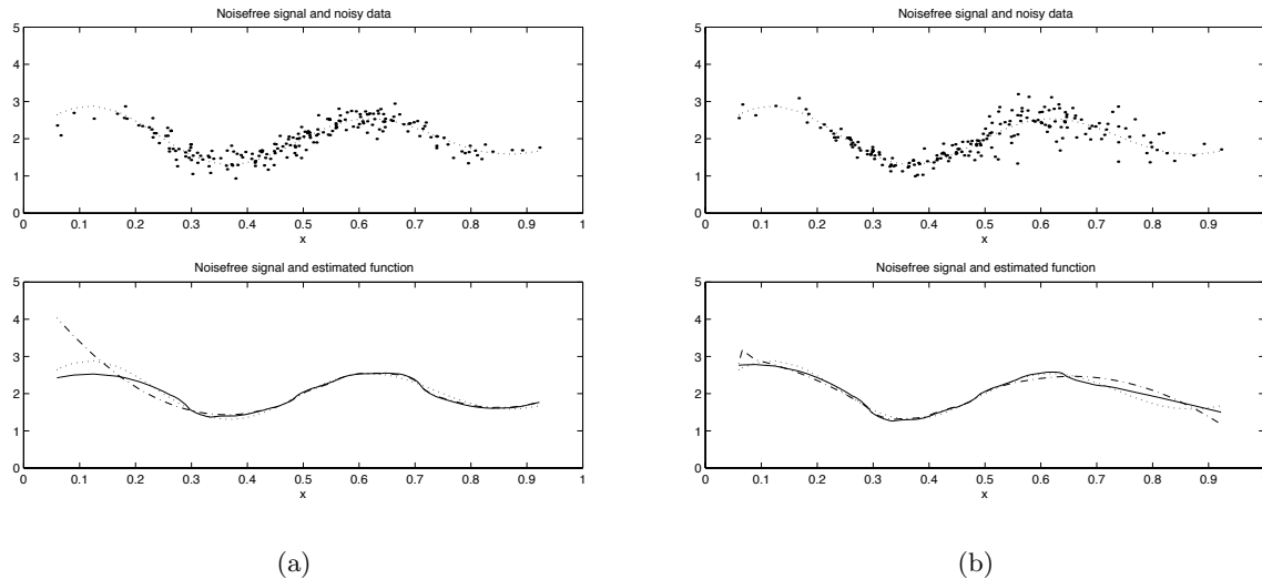
Figure 7: Estimation of the Damped Sine function in case of (a) i.i.d. errors (b) heteroscedasticity. The dotted line represents the underlying signal. The WAI estimators with and without update are plotted in continuous and in dashed line, respectively. The RMSE equals 3.84% in (a), 4.11% in (b) for the estimator with update, and 7.32% in (a), 6.70% in (b) without update.
