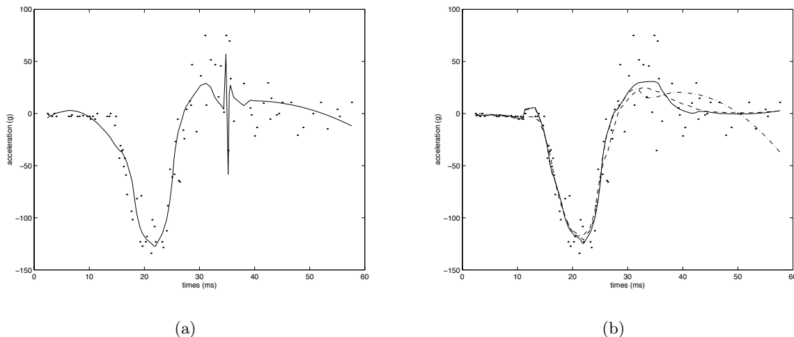
Figure 9: Motorcycle acceleration data are represented in dots. In (a) the WAI estimator with update using the three-step procedure is shown. In (b) we first removed all details at level J - 1 , then applied the iterative algorithm with update (plain line) and without update (interrupted dashed line). The k -nearest neighbour estimate is in dashed line. Both wavelet estimators seem to indicate a change point in the first derivative around 23 ms.
