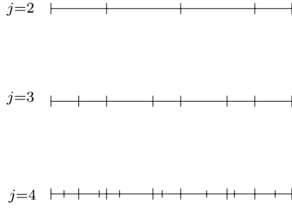
Figure 1: Coarsening procedure when n is not a power of two. At the level j = 4 , we combine the 14 intervals two by two to produce 7 intervals at level j = 3 . The first 6 intervals are further combined to produce the first three intervals at the coarser level, the last interval being passed unchanged to the level j = 2 .
