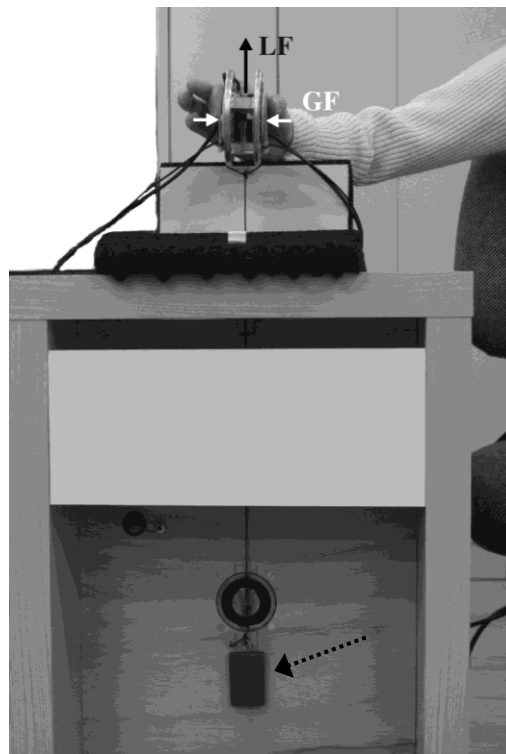
Figure II.1. Handheld object used to measure the different forces during the task. Grip force (GF) normal to the contact surfaces is indicated by white arrows, tangential load force (LF) by a black arrow and the steel mass by a dotted arrow.
