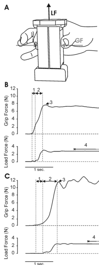
Figure III.2. (A) Diagram of the manipulandum held between the thumb and index fingers. Light grey arrows indicates the grip force (GF) while the black arrow indicates the load force (LF) exerted on the contact surfaces. (B) Typical trace of a grip-lift trial realized with the dominant hand of a healthy subject. (C) Paretic hand, of a chronic stroke subject, grip-lift trial typical trace. Both traces (B-C) indicate the preloading phase (1), the loading phase (2), the GF peak (3), and part of the stable phase (4).
