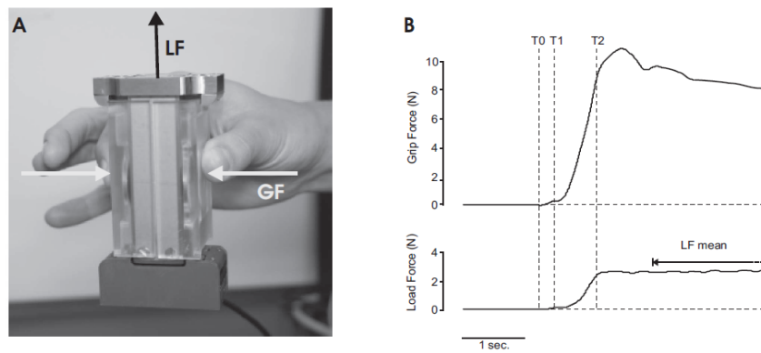
Figure IV.1.2 (A) The manipulandum and vectors illustrating the forces: grip force (GF) in grey and load force (LF) in black. (B) Typical recordings of LF and mean GF exerted by the two fingers. The vertical dotted lines indicate the temporal parameters: T0-T1=preloading phase; T1-T2=loading phase.
