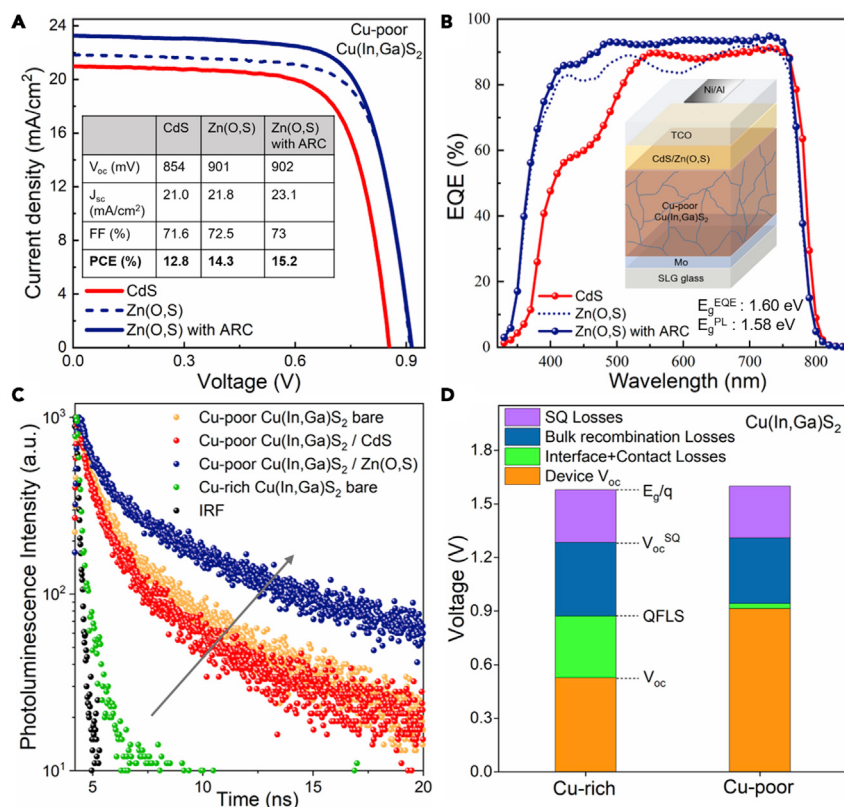
Figure 5. High-efficiency solar cell from Cu-poor Cu(In,Ga)S 2
