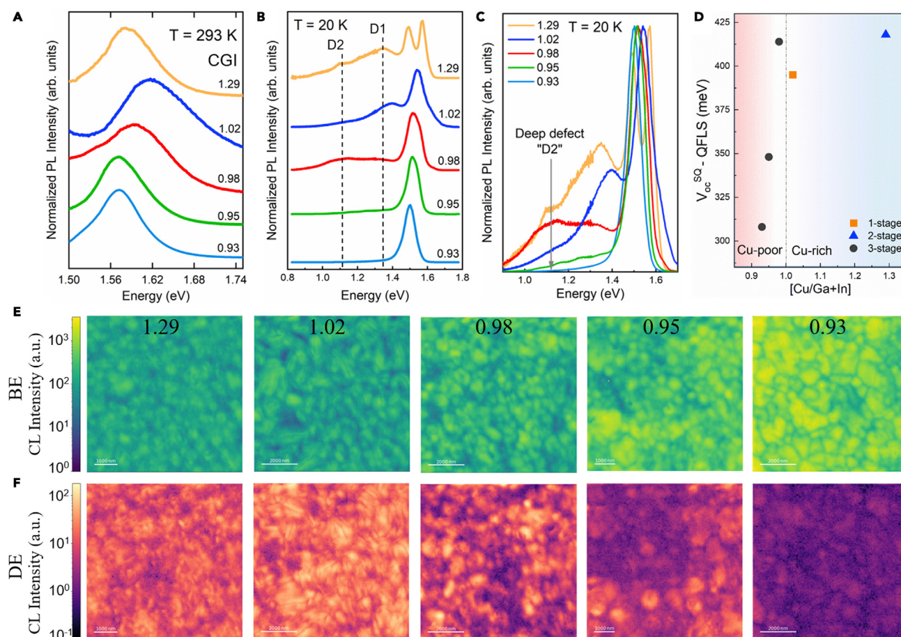
Figure 2. QFLS deficit and defect analysis from photoluminescence and cathodoluminescence measurements
