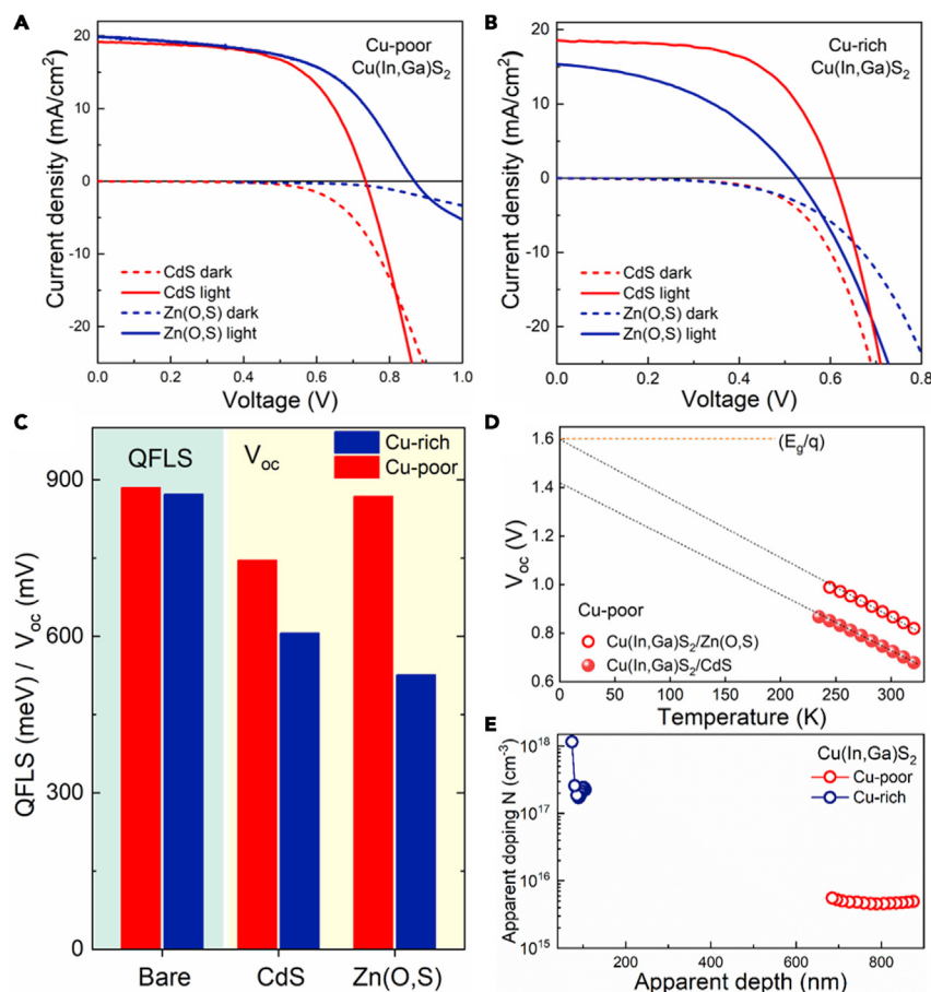
Figure 4. Optoelectronic comparison between Cu-poor and Cu-rich Cu(In,Ga)S 2 solar cells
