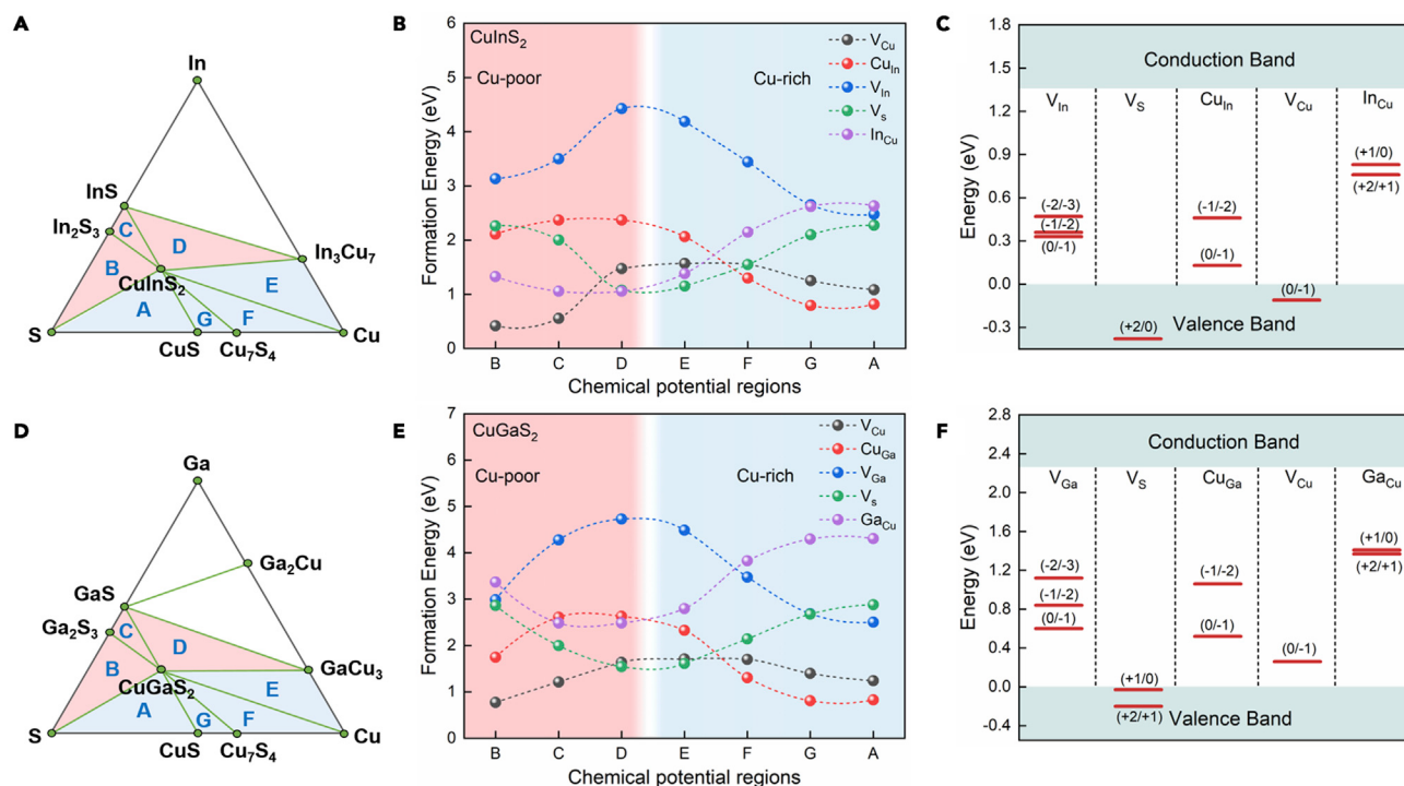
Figure 3. Theoretical analysis of the defect formation energies and their energetic position in CuInS 2 and CuGaS 2
