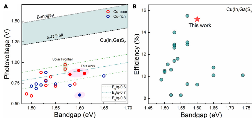
Figure 6. Summary of the photovoltage and efficiency in context to literature
