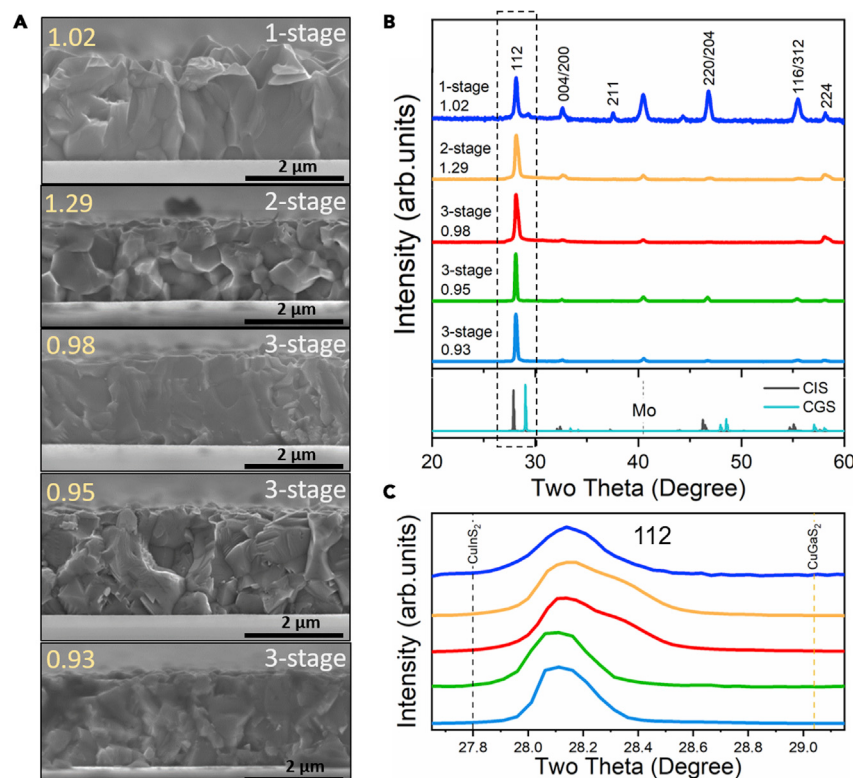
Figure 1. Structural characterization of Cu(In,Ga)S 2 thin films with varying CGI ratios
