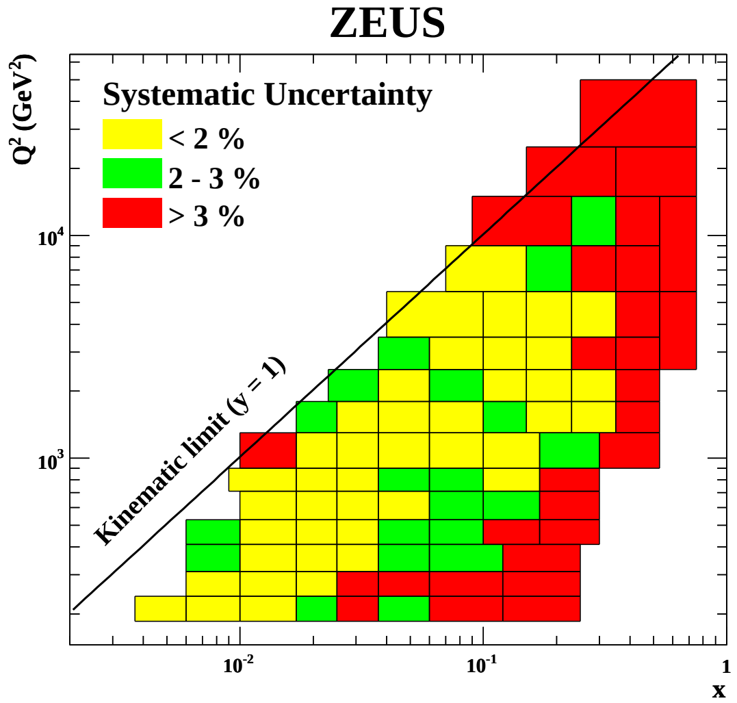
Figure 2: The total systematic uncertainty for the bins used in the reduced cross section measurements.
