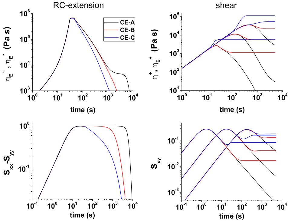
FIG. 4. Left: (upper) \eta_E^+, \eta_E^- vs time for all three constitutive equations at \dot{\epsilon} = 0.1\text{s}^{-1} . The flow is ceased at t \simeq 45\text{s} ( \epsilon_0 = 4.5 ). (Bottom) the corresponding orientation alignment. Right: (upper) \eta^+ vs time. (Bottom) the corresponding shear component of the orientation tensor. In all panels, the black, red, and blue lines refer to CE-A, CE-B, and CE-C, respectively. In all cases, ES is quenched.
