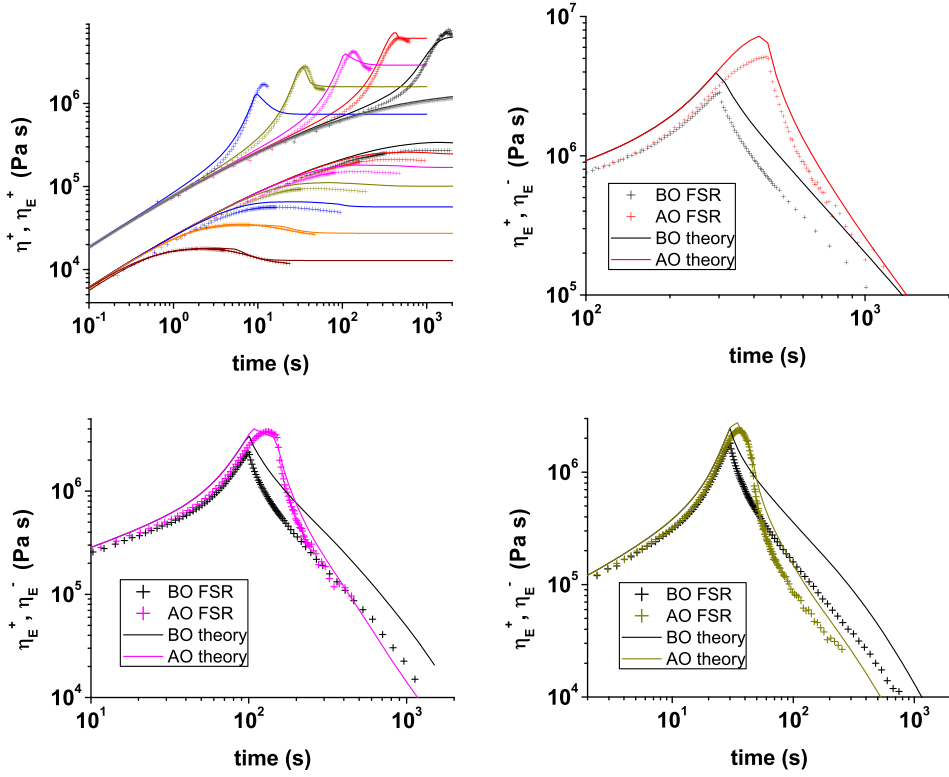
FIG. 8. Comparison of the minimal model (lines) with the FSR data (symbols) for extension and shear data [Hassell et al. (2008)], for the DOW 150 R sample, using the parameterization shown in Table III. NC for shear and extension (upper, left). RC following the extensional flow: \dot{\epsilon} = 0.01 \text{ s}^{-1} (upper right), \dot{\epsilon} = 0.03 \text{ s}^{-1} (bottom left), and \dot{\epsilon} = 0.1 \text{ s}^{-1} (bottom right). For each rate, the flow has been stopped at \epsilon_0 = 3 and \epsilon_0 = 4.5 for the BO and AO case, respectively. The color code for the rates is the same as in Fig. 7 and is explained in Table IV.
