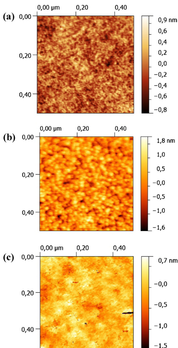
Fig. 2. AFM 2D images of the surface of (a) template-free \text{TiO}_2 , (b) TiB and (c) TiP films.
