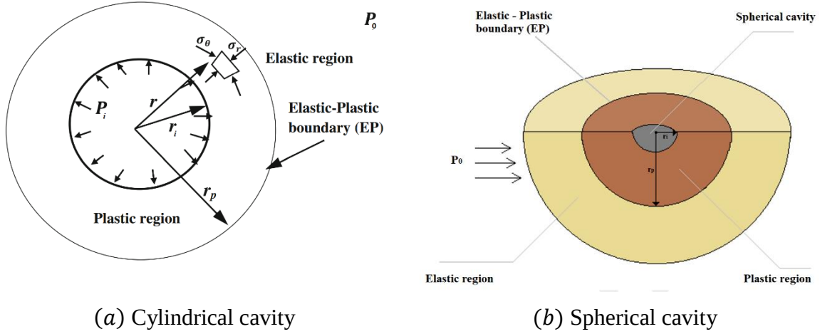
Figure 1: Geometry of the problem and boundary conditions
