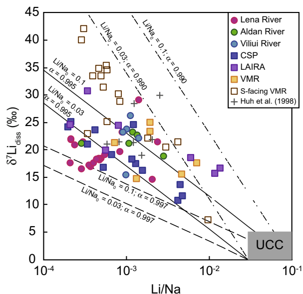
Fig. 5. Relationship between measured \delta^7\text{Li}_{\text{diss}} and Li/Na molar ratios for the Lena River. Shown for comparison are Lena River data from Huh et al. (1998a). The lines represent the evolution of \delta^7\text{Li} and Li/Na following a Rayleigh distillation model, in which Li is supplied to waters by dissolution of primary silicate minerals, followed by the progressive removal of Li into secondary minerals. Curves are shown for different starting values and different fractionation factors for Li removal. The grey field represents the range of values that are generally expected for dissolution of silicate rocks, with Li/Na molar ratios between the highest measured in the Lena River watershed and the composition of upper continental crust (UCC), and \delta^7\text{Li} values for UCC and typical shales (Taylor and McLennan, 1995; Teng et al., 2004; Dellinger et al., 2014; Sauzéat et al., 2015). CSP = Central Siberian Plateau; LAIRA = Lena-Amginsky inter-river area; VMR = Verkhoyansk Mountain Range. Open symbols represent VMR rivers draining south-facing catchments.
