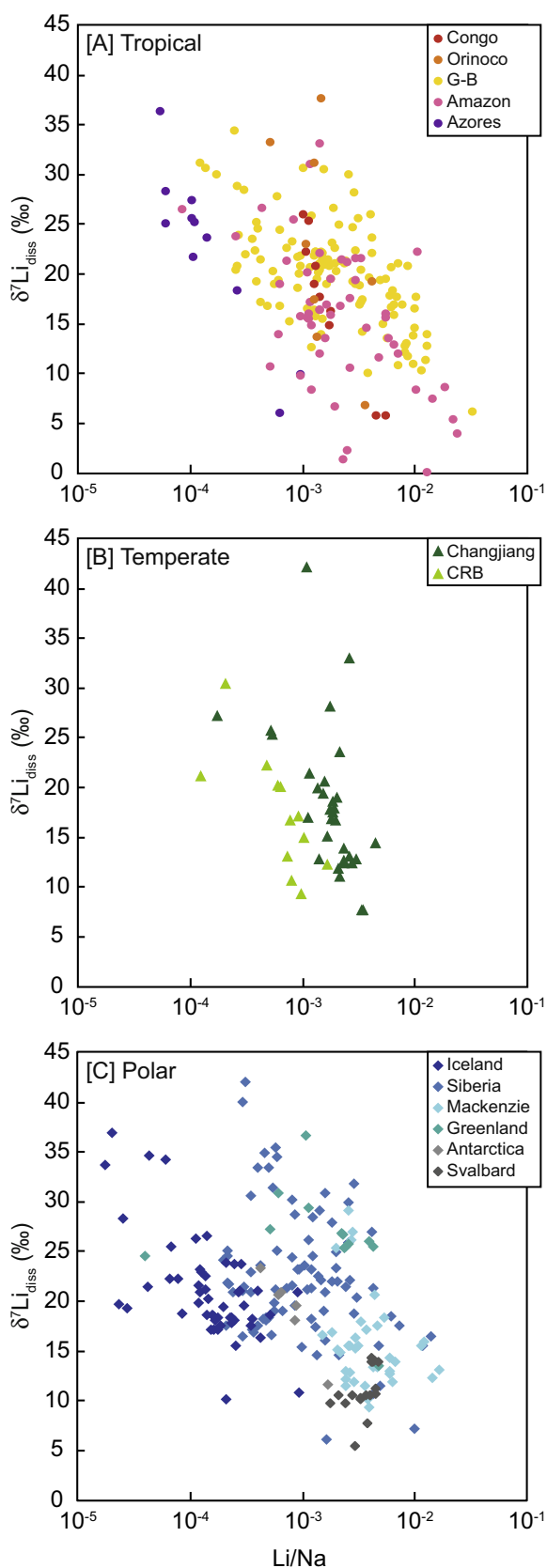
Fig. 6. A compilation of dissolved Li isotope values versus molar \text{Li}/\text{Na} for rivers in [A] tropical, [B] temperate and [C] polar regions. Despite vastly different climatic and weathering regimes, the same range of riverine \delta^7\text{Li} values globally suggests that cryogenic weathering features typical of permafrost-dominated regions and climate (temperature and runoff), are not a dominant control on \delta^7\text{Li} fractionation. Data include the Lena River and other Siberian rivers (this study; Huh et al., 1998a); the Mackenzie River (Millot et al., 2003; Millot et al., 2010); Antarctic rivers (Witherow et al., 2010); Greenland (Wimpenny et al., 2010b); Svalbard (Hindshaw et al., 2016; Hindshaw et al., 2018); the High Himalayas (Huh et al., 1998a; Kısakürek et al., 2005); the Ganges-Brahmaputra (Huh et al., 1998a; Kısakürek et al., 2005; Bagard et al., 2015; Frings et al., 2015; Manaka et al., 2017; Pogge von Strandmann et al., 2017); the Amazon (Huh et al., 1998a; Dellinger et al., 2015); the Orinoco (Stallard et al., 1995, 1996; Huh et al., 1998a); the Congo (Henchiri et al., 2016); Changjiang (Yangtze) River (Huh et al., 1998a; Liu et al., 2011; Wang et al., 2015); and basalts from Iceland, the Azores and the Columbia River Basalts (Pogge von Strandmann et al., 2006; Vigier et al., 2009; Pogge von Strandmann et al., 2010; Liu et al., 2015).
