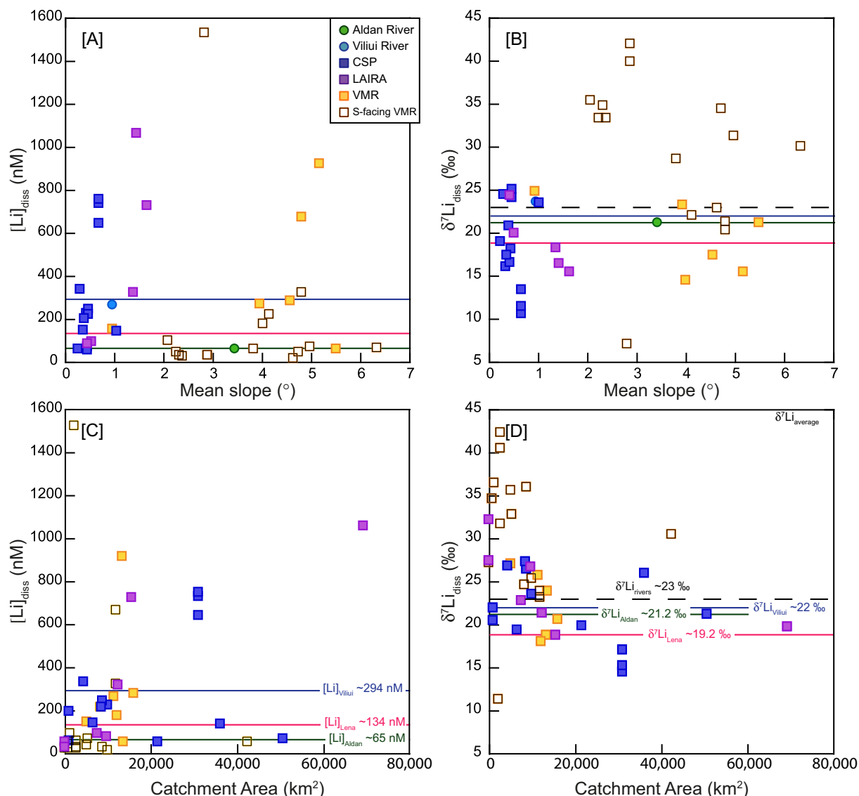
Fig. 3. Dissolved Li concentrations and \delta^7\text{Li} compositions compared with watershed gradient [A, B] and catchment area [C, D] for tributaries draining the Central Siberian Plateau (CSP), Lena-Amginsky inter-river area (LAIRA) and Verkhoyansk Mountain Range (VMR) regions. The lack of trends with watershed gradient may in part be a result of the unique cryogenic physical erosion processes associated with the presence of continuous permafrost, which obscure relationships observed in rivers draining high topography in non-permafrost rivers. The greatest variation in \delta^7\text{Li}_{\text{diss}} compositions is seen in smaller ( <10,000 \text{ km}^2 ) catchment areas, particularly in rivers draining the south-facing catchments of the VMR (open symbols). Tributaries draining larger catchment areas tend to have \delta^7\text{Li}_{\text{diss}} values closer to the global mean riverine value of 23\text{‰} (shown as dashed line, after Huh et al. 1998a) as well as the average \delta^7\text{Li}_{\text{diss}} compositions of the Lena, Aldan and Viliui Rivers (shown as solid lines in pink, green and blue respectively).
