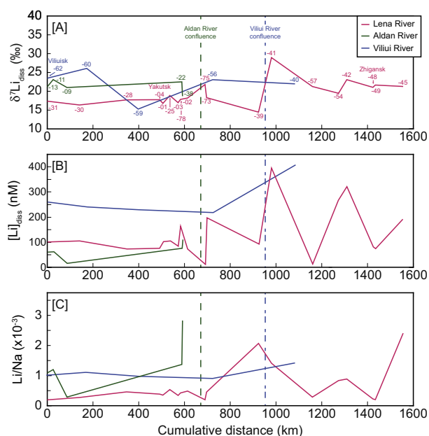
Fig. 4. Downstream variations in \delta^7\text{Li}_{\text{diss}} , [\text{Li}] and \text{Li}/\text{Na} in the Lena River main channel, and major tributaries of the Aldan and Viliui Rivers that converge into the main channel. River sample numbers are shown adjacent to curves, and arrows indicate the downstream river location of major towns. Confluences of the Aldan and Viliui Rivers into the Lena River main channel are shown as dashed lines. See Fig. 1 for more information. No systematic trends can be observed in [\text{Li}] , or \text{Li}/\text{Na} . A gradual \sim 5\% increase can be seen along the Lena River main channel, see text for further details.
