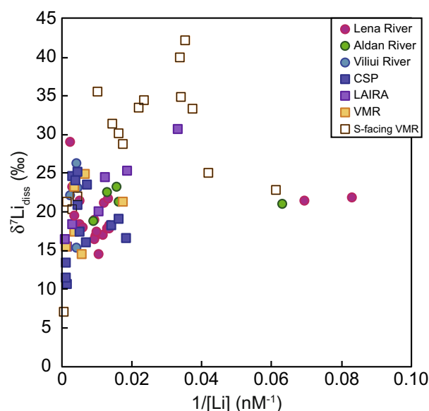
Fig. 2. \delta^7\text{Li}_{\text{diss}} compositions versus the inverse of dissolved Li concentrations for rivers in the Lena River watershed. Previous values from the Lena River watershed are shown for comparison (not shown is one anomalous sample UL436 that drains the evaporitic marine carbonates within the Siberian Platform with high [Li] of 3350 nM and \delta^7\text{Li}_{\text{diss}} = 21.2\text{‰} (Huh et al., 1998a)). The range of values do not define clear, straight line mixing trajectories, thus are unlikely to be explained by simple mixing between two riverine end-members, and reflect the complex behaviour of Li in this watershed. Uncertainties on \delta^7\text{Li} smaller than the symbols. CSP = Central Siberian Plateau; LAIRA = Lena-Anginsky inter-river area; VMR = Verkhoyansk Mountain Range. Open symbols represent VMR rivers draining south-facing catchments, which show the greatest variation in both [Li] and \delta^7\text{Li}_{\text{diss}} .
