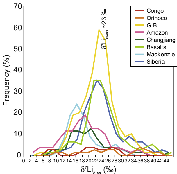
Fig. 7. A two point moving average frequency histogram (2 permil bin width) summarising dissolved \delta^7\text{Li} compositions from large global rivers, and rivers draining basaltic terrains. A large peak can be seen clustering around the global median value of 23\text{‰} (Huh et al., 1998b), with a smaller peak around \sim 14 to 16\text{‰} . Data from same sources as Fig. 6.
