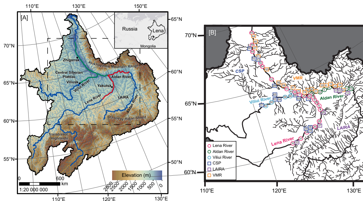
Fig. 1. Map showing [A] the Lena River catchment and its sub-catchment regions with the July 2012 sampling route shown in red and June 2013 in green. Sampling locations are shown [B] with samples within the Lena River main channel or the Viliui and Aldan Rivers, which are major tributaries, denoted by circles. Smaller tributaries of the Central Siberian Plateau (CSP), Lena-Amginsky inter-river area (LAIRA) and Verkhoyansk Mountain Range (VMR) are denoted by squares (maps modified after Hirst et al. 2017 ).
