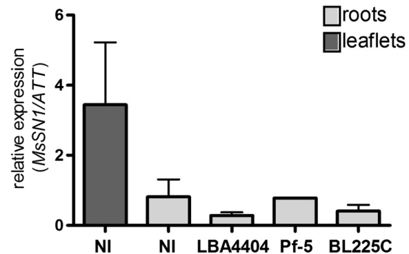
Figure 4 Quantitative analysis of the expression of the MsSN1 gene in wild type alfalfa plants under microbe stress conditions. Real-time RT-PCR studies for MsSN1 expression in non-inoculated leaves and roots (NI) or in roots exposed to Agrobacterium tumefaciens LBA4404, Pseudomonas fluorescens Pf-5 and Sinorhizobium meliloti BL225C for 24 hs.
