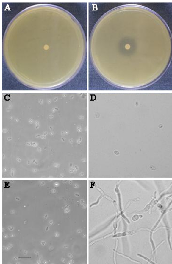
Figure 3 Analysis of the in vitro antimicrobial activity of MsSN1 . Agrobacterium growth (A-B) and Phoma spore germination ( 1 \times 10^5 spores/ml) (C-F) inhibition assays using MsSN1 -free (A, C and D) or MsSN1 extracts (B, E and F). Spore germination was examined immediately (C and E) and after 16 h (D and F) of incubation with the extracts. Bar = 50 µm.
