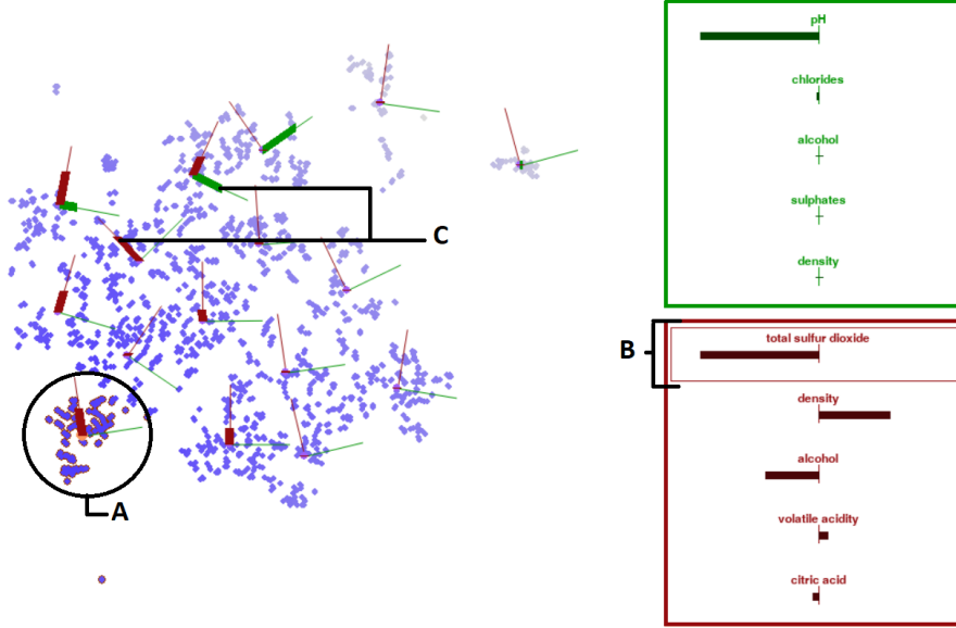
Figure 1: Interface for the proposed globally local and fast explanation framework.
