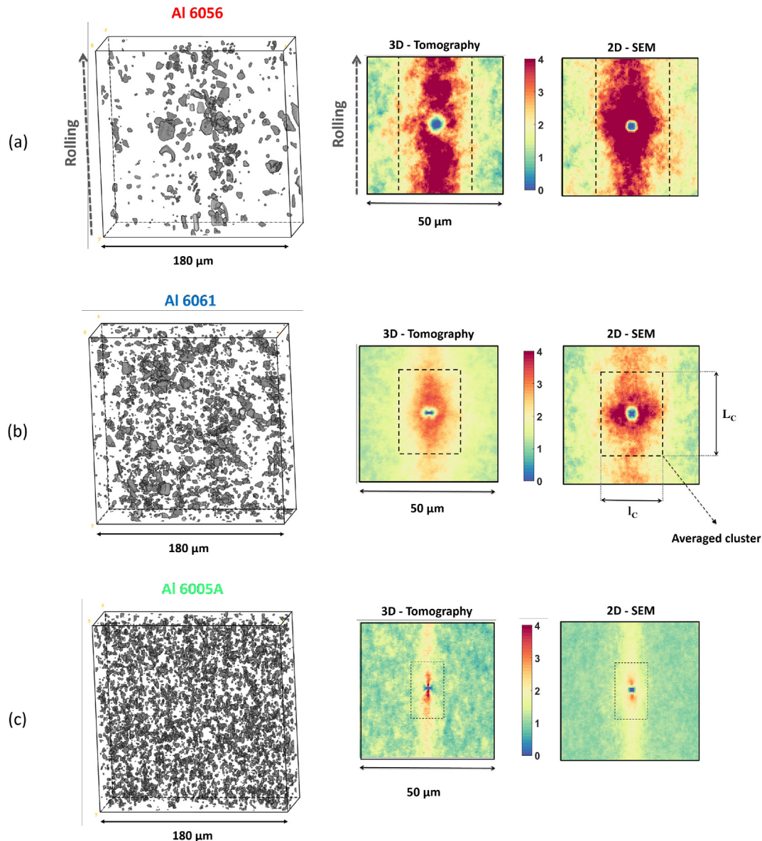
Fig. 3. (Left) 3D microtomography perspective of particles distribution in the aluminium alloys (a) 6056, (b) 6061 and (c) 6005A and (Right) corresponding pair correlation functions (PCFs) for the RD-TD plane through the center of the sub-volume. A PCF value smaller or larger than one corresponds respectively to a smaller or larger probability to find a neighbor in the vicinity of a particle compared to a perfectly homogenous distribution.
