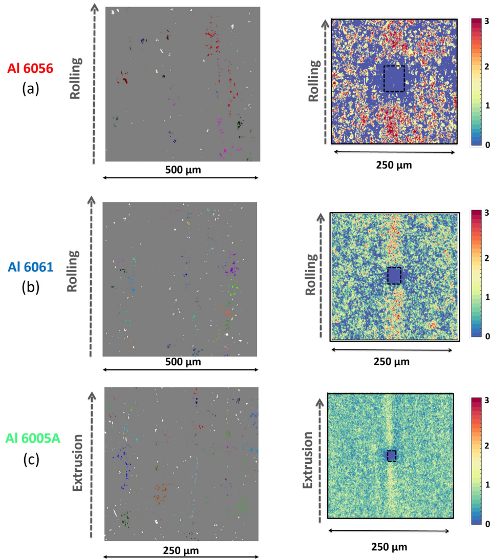
Fig. 4. (Left) Visualisation of a few clusters from particle distribution shown in the SEM images of Fig. 2. (Right) PCF analysis performed on clusters from SEM images for the alloys (a) Al 6056, (b) Al 6061 and (c) Al 6005A.
