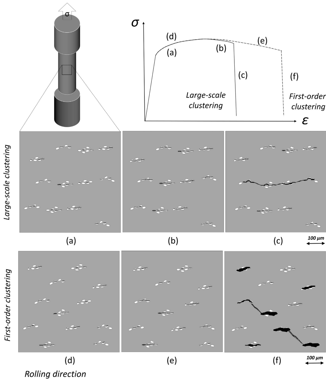
Fig. 8. Schematics of the damage sequence in the alloy Al 6056 ((a), (b) and (c)), and in the alloys Al 6061 and 6005A ((d), (e) and (f)).
