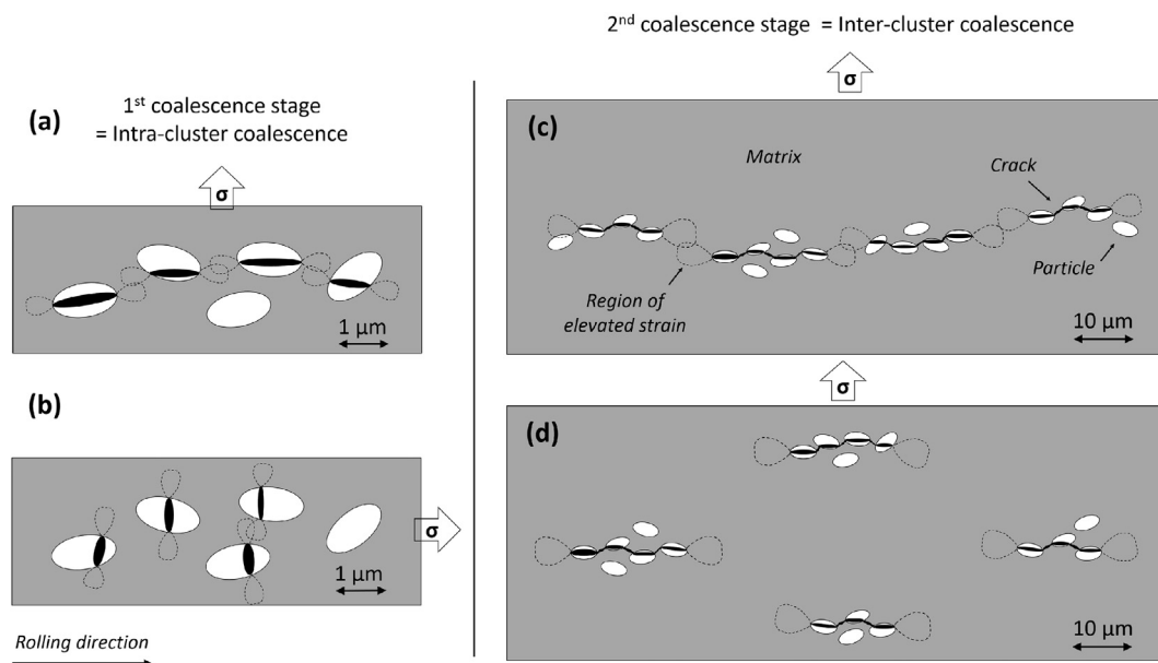
Fig. 7. Schematic of the effect of microstructural anisotropy on the damage percolation process. The effect of the stringer orientation on the first coalescence stage (i.e. intra-cluster) is shown in (a) and (b). The effect of the clusters distribution on the second coalescence stage (i.e. inter-cluster) is shown in (c) and (d). In the case of discontinuous stringer (d), a second void growth process based on the early coalesced voids sets in until second coalescence.
