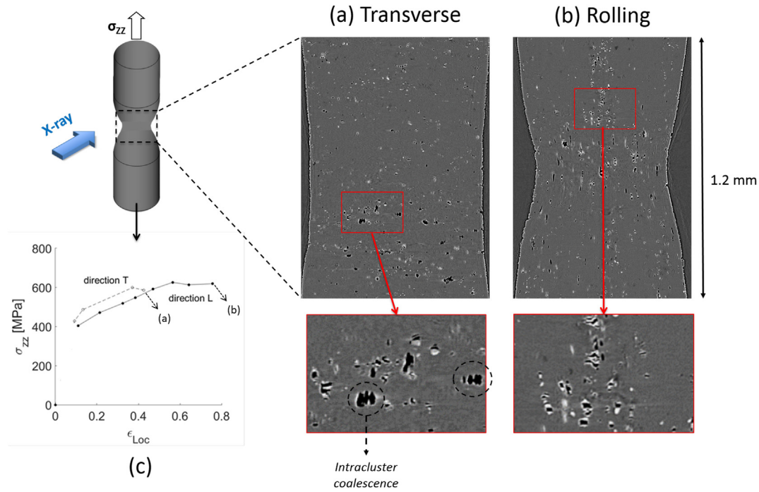
Fig. 5. X-ray microtomography reconstructed images just before fracture of the tensile test performed on the alloy Al 6056-T4 loaded in (a) the transverse direction and (b) the rolling direction. Voids appear in black in the grey matrix and IM particles appear in white. The tensile curves in (c) correspond to the in situ tensile tests shown in (a) and (b).
