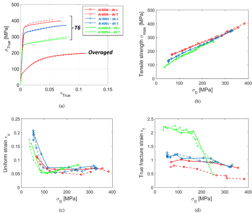
Fig. 1. (a) True stress-true strain curves until necking for the three alloys in the T6 state and loaded along the rolling (plain line) and transverse direction (dashed line). Variation of the different parameters extracted from the uniaxial tensile tests on the three alloys, as a function of the yield stress corresponding to the different heat treatments: (b) tensile strength of the three Al alloys; (c) true strain at the onset of necking; (d) true fracture strain.
