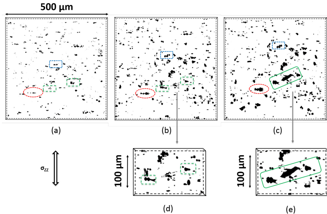
Fig. 6. Void distribution observed during in-situ microtomography in the alloy Al 6056 loaded in the transverse direction at a local strain of (a) \epsilon_{Loc} = 0.1 , (b) \epsilon_{Loc} = 0.35 and (c) \epsilon_{Loc} = 0.43 . (d) Zoom of figure (b), showing the formation of a second population of voids between two clusters of voids. (e) Zoom of figure (c), showing the intercluster coalescence with the formation of micro shear band.
