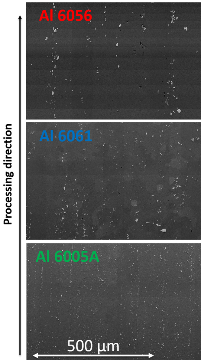
Fig. 2. SEM micrographs taken in the processing-transverse plane showing the distribution of intermetallic particles (in white) in the alloys Al 6056, Al 6061 and Al 6005A.
