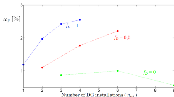
Figure 7 - Negative sequence voltage unbalance factor at the last node of the radial 10 nodes feeder, in function of the amount of connected DG units
