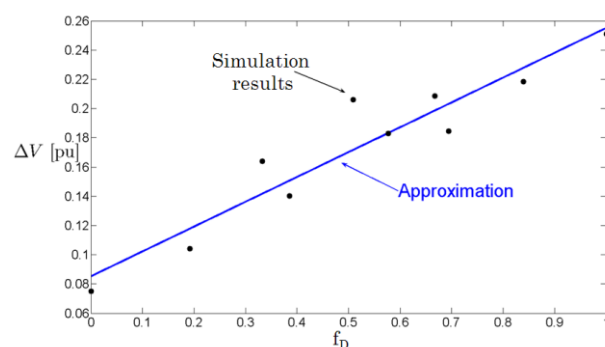
Figure 9 - Maximum overvoltage in function of the distribution factor (30 nodes feeder)
