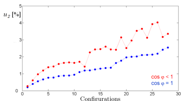
Figure 11 – Increase of the voltage unbalance due to reactive power consumption for various configurations
