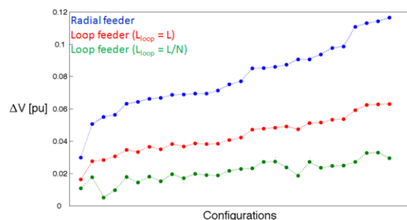
Figure 13 – Overvoltage reduction by looping the feeder
