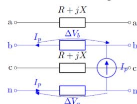
Figure 1 – Simplified case of a feeder with a single-phase PV installation connected at the end
