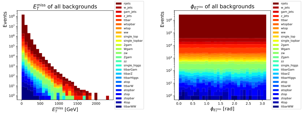
Figure 5: Missing transverse energy E_T^{\text{miss}} in GeV and azimuthal angle \phi_{E_T^{\text{miss}}} for all backgrounds.
