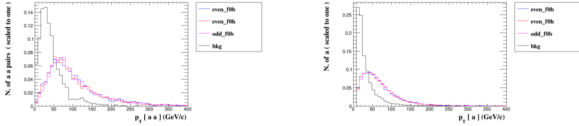
Figure 3: Left-hand side: Normalised distribution of the diphoton system transverse momentum, p_{T,\gamma\gamma} (in GeV). Right-hand side: Normalised distribution of the photon system transverse momentum, p_{T_\gamma} (in GeV). We consider a scalar mass m_\phi = 20 GeV. The signal and SM background (black) are superimposed over each other. A typical scale value f_B = f_W = 1 TeV, f_H = 1 TeV and \tilde{f}_B = \tilde{f}_W = 1 TeV is used respectively in the case CP-even _1/f_V (blue), CP-even _1/f_H (red) and CP-odd _1/\tilde{f}_V (purple).
