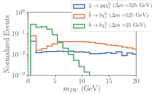
Figure 3: The invariant mass distribution for candidate displaced vertices. The blue histogram shows the distribution for a gluino simplified model with a large mass gap: (m_{\tilde{g}}, m_{\tilde{\chi}_1^0}) = (625 \text{ GeV}, 100 \text{ GeV}) . The orange histogram shows the distribution for the model considered here with masses (m_{\tilde{b}}, m_{\chi}) = (625 \text{ GeV}, 100 \text{ GeV}) , while the green histogram shows the same distribution but for the compressed scenario: (m_{\tilde{b}}, m_{\chi}) = (625 \text{ GeV}, 600 \text{ GeV}) .
