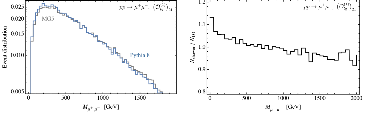
Figure 1: Left: Invariant mass distribution of dimuon signal events; the gray line is generated with MG5_AMC, the blue line includes PYTHIA8 parton showering. Right: relative correction due to parton showering as function of dimuon invariant mass.
