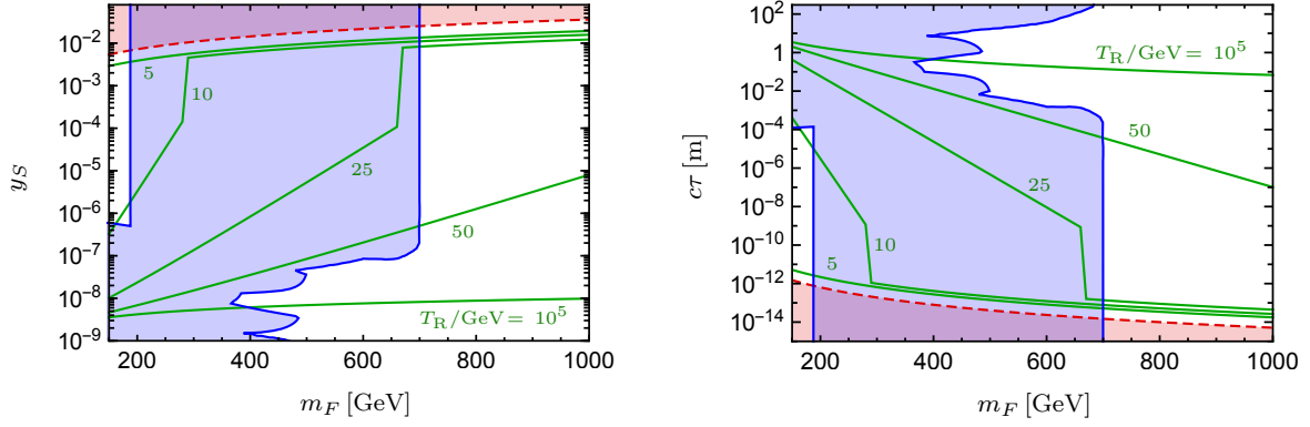
Figure 5: Summary of the results obtained in this work in the (m_f, y_s) (left panel) and (m_f, c\tau) (right panel) planes, assuming a dark matter mass m_s = 12 keV: Contours along which the cosmic DM abundance as measured by Planck can be explained through freeze-in of s (green lines) along with global constraints from searches for prompt dileptons plus MET, displaced leptons plus MET, disappearing tracks and Heavy Stable Charged Particles (blue shaded region) and parameter space region disfavoured by \mu \rightarrow e\gamma (red shaded region).
