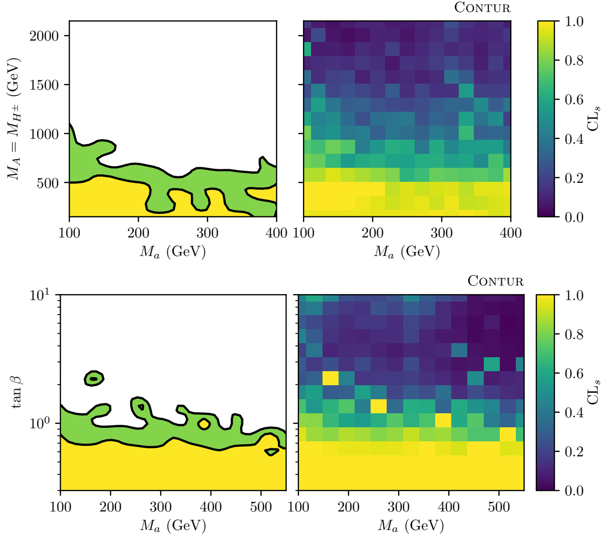
Figure 2: CONTUR scans over the parameter planes shown in Fig. 1 in the M_a – M_A (top) and M_a – \tan \beta plane (bottom). Left: 95% (68%) excluded contours in yellow (green). Right: Underlying heatmap of exclusion at each investigated parameter space point.
