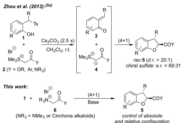
Scheme 1. Zhou and co-workers' recently developed sulfur ylide ( 4 ) addition to o -quinone methides 3 and targeted use of (chiral) ammonium salts 6 to control the absolute and relative configurations of 2,3-dihydrobenzofurans 5 .
