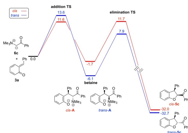
Figure 1. Computed free-energy profiles [ \text{kcal mol}^{-1} ] for the formation of cis - and trans -2,3-dihydrobenzofurans 5c from ammonium ylide 6c .
