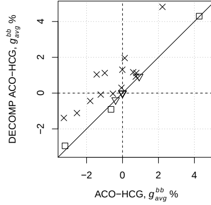
Figure A.1: Comparison of DECOMP ACO-HCG and ACO-HCG. Each point gives the average relative deviation from the bb-best solution over 10 independent runs. The symbols denote whether there is statistically significant difference (X) or not (□), or all the runs obtained the same cost (▽).
