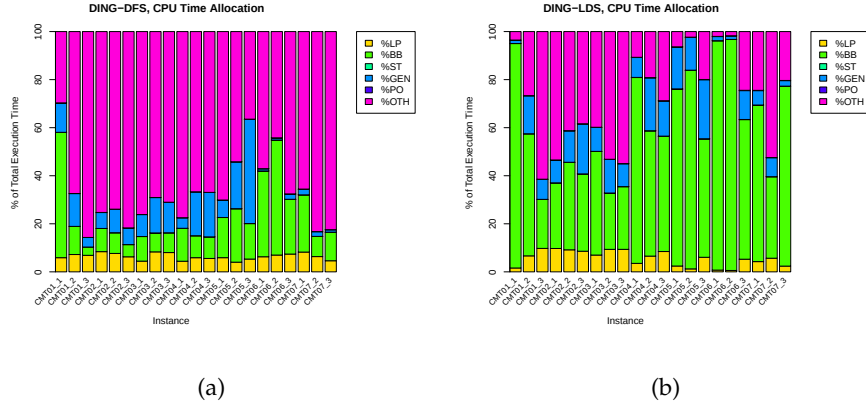
Figure 13.6: DING: CPU Time Allocation
