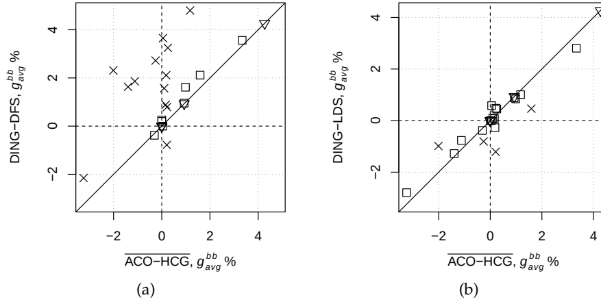
Figure A.2: Comparison of DING and \overline{\text{ACO-HCG}} , ACO-HCG in the manual configuration. Each point gives the average relative deviation from the bb\text{-best} solution over 10 independent runs. The symbols denote whether there is statistically significant difference (X) or not ( \square ), or all the runs obtained the same cost ( \nabla ).
