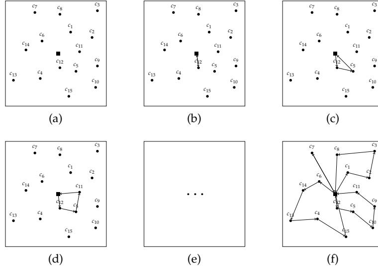
Figure 2.3: Execution of the Mole and Jameson Heuristic on a CVRP.
