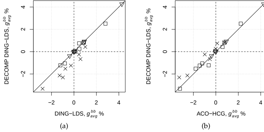
Figure A.3: Comparison of DECOMP DING-LDS with DING-LDS and with ACO-HCG. Each point gives the average relative deviation from the bb -best solution over 10 independent runs. The symbols denote whether there is statistically significant difference (X) or not (□), or all the runs obtained the same cost (▽).
