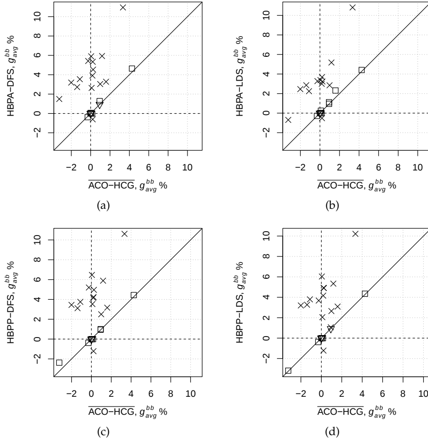
Figure A.4: Comparison of HBP and \overline{\text{ACO-HCG}} , the manual configuration of ACO-HCG. Each point gives the average relative deviation from the bb -best solution over 10 independent runs. The symbols denote whether there is statistically significant difference (X) or not ( \square ), or all the runs obtained the same cost ( \nabla ).
