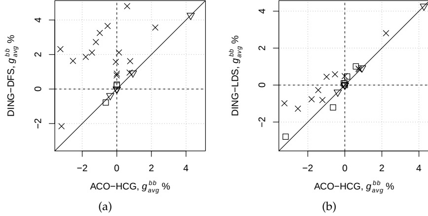
Figure 12.5: Comparison of DING and ACO-HCG. Each point gives the average relative deviation from the bb -best solution over 10 independent runs. The symbols denote whether there is statistically significant difference (X) or not (□), or all the runs obtained the same cost (▽).
