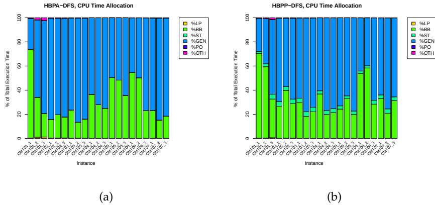
Figure 13.9: HBP: CPU Time Allocation
