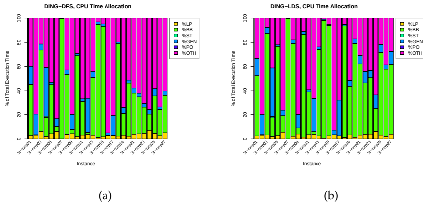
Figure 12.6: DING: CPU Time Allocation
