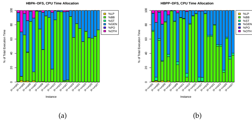
Figure 12.9: HBP: CPU Time Allocation
