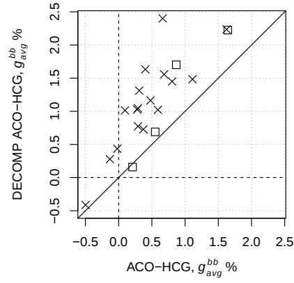
Figure B.1: Comparison of DECOMP ACO-HCG and ACO-HCG. Each point gives the average relative deviation from the bb -best solution over 10 independent runs. The symbols denote whether there is statistically significant difference (X) or not ( \square ), or all the runs obtained the same cost ( \nabla ).
