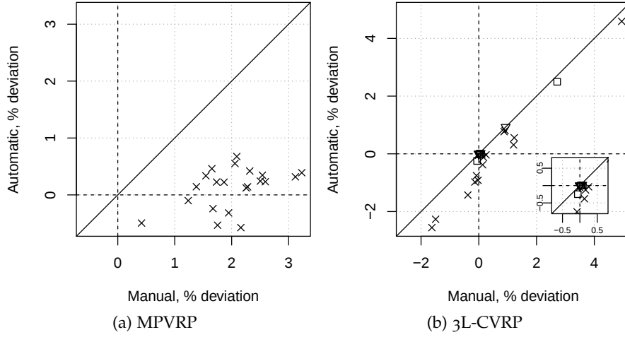
Figure 11.1: Comparison between manual and automatic configuration. Each point gives the mean %-deviation from the best-bb solution over 20 runs with different random seed on the same test instance. The symbols denote whether there is a statistically significant difference (X) or not ( \square ), or all the runs obtained the same cost ( \nabla ).
