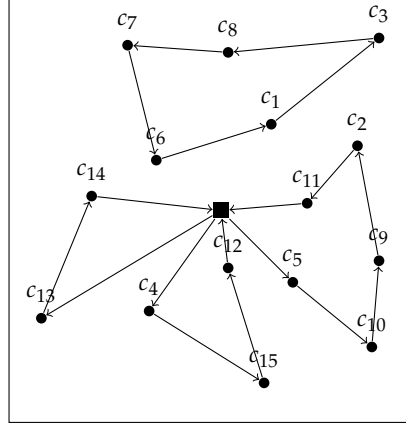
Figure 2.7: A subtour visiting customers c_1, c_3, c_8, c_7 and c_6 A subtour is a cycle in the problem graph not containing the depot vertex.
