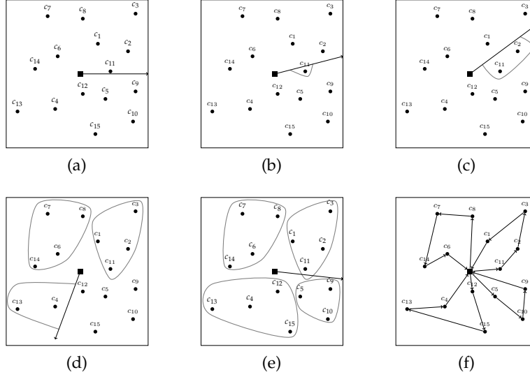
Figure 2.4: Intermediate steps in the execution of the Sweep Heuristic on a CVRP. Note that the Sweep heuristic is designed for instances where the customers are distributed in clusters.
