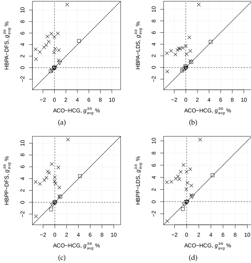
Figure 12.8: Comparison of HBP and ACO-HCG. Each point gives the average relative deviation from the bb -best solution over 10 independent runs. The symbols denote whether there is statistically significant difference (X) or not (□), or all the runs obtained the same cost (▽).
