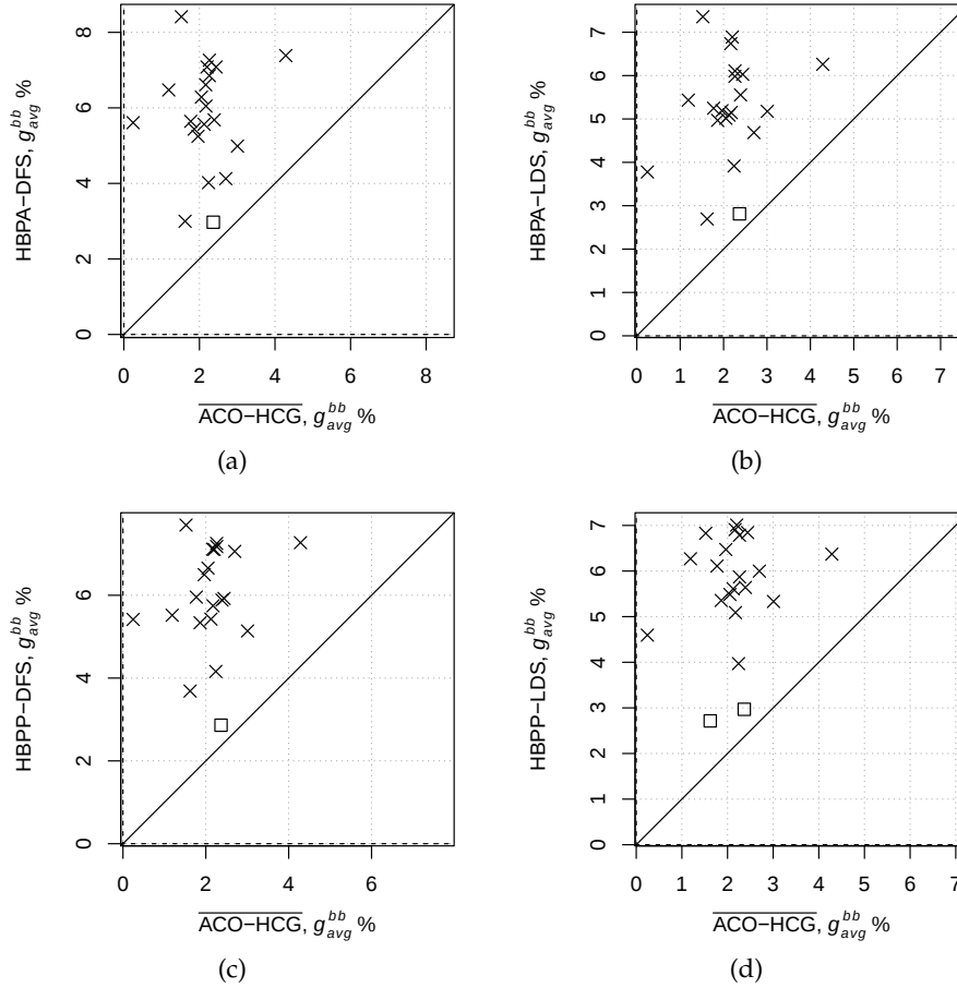
Figure B.4: Comparison of HBP and \overline{\text{ACO-HCG}} , the manual configuration of ACO-HCG. Each point gives the average relative deviation from the bb -best solution over 10 independent runs. The symbols denote whether there is statistically significant difference (X) or not ( \square ), or all the runs obtained the same cost ( \nabla ).
