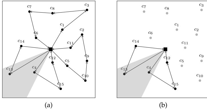
Figure 9.1: A wedge selected in a CVRPBB solution (a). The routes (and their customers) extracted using this wedge are shown in (b).
