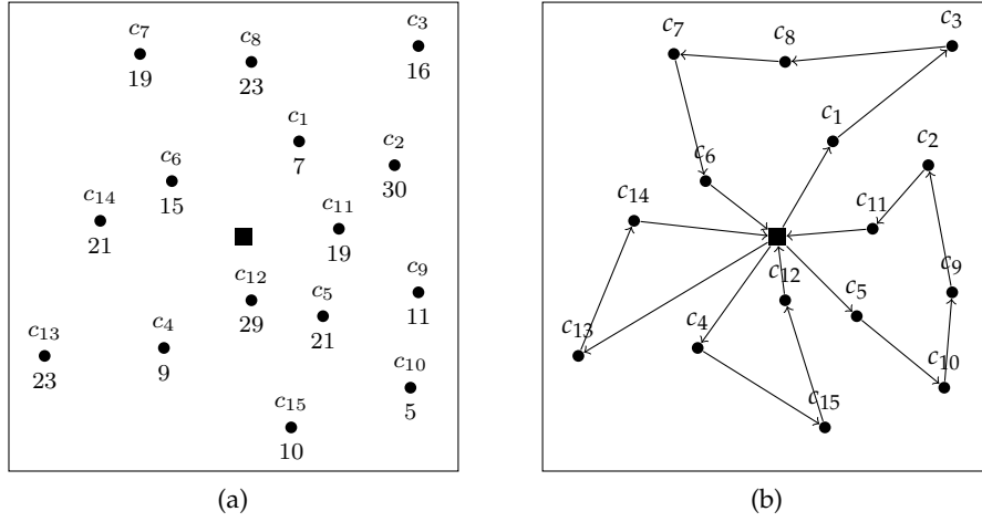
Figure 2.1: A CVRP instance with |K| = 4 and Q = 90 (a) and one of its feasible solutions (b). The customer demands are indicated below each customer vertex in the instance. In order to improve visibility the customer demands are not indicated in the solution.
