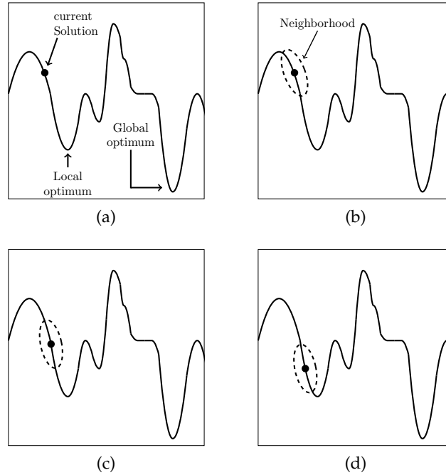
Figure 2.5: Local Search moving through the solution space towards a local optimum.
