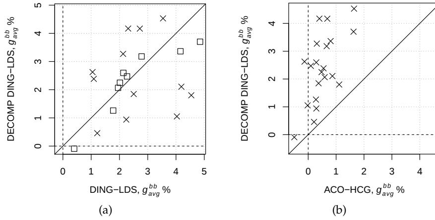
Figure B.3: Comparison of DECOMP DING-LDS with DING-LDS and with ACO-HCG. Each point gives the average relative deviation from the bb -best solution over 10 independent runs. The symbols denote whether there is statistically significant difference (X) or not (□), or all the runs obtained the same cost (▽).
