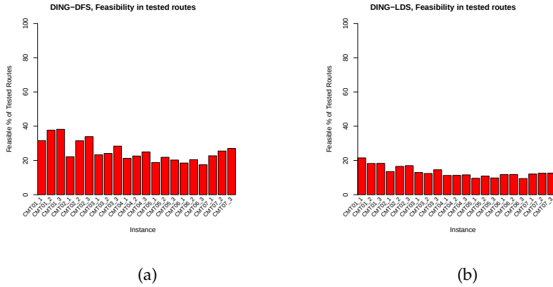
Figure 13.7: DING: % of tested routes that were bb -feasible
