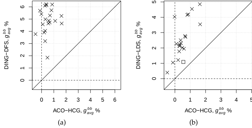
Figure 13.5: Comparison of DING and ACO-HCG. Each point gives the mean %-deviation from the bb -best solution over 10 independent runs. The symbols denote whether there is statistically significant difference (X) or not ( \square ), or all the runs obtained the same cost ( \nabla ).
