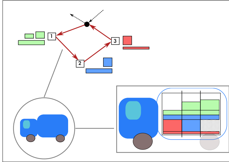
Figure 13.2: Feasible loading for a MP-VRP route
