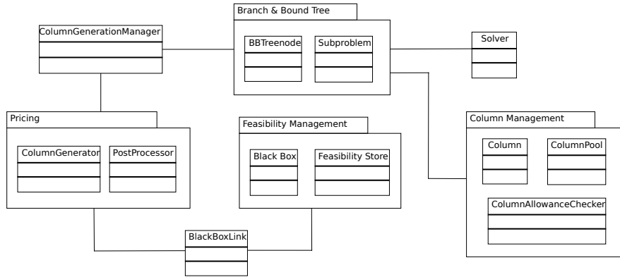
Figure 10.1: Visualization of the most important classes and their responsibilities. Links indicate communication streams.
