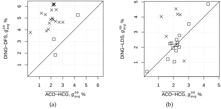
Figure B.2: Comparison of DING and \overline{\text{ACO-HCG}} , ACO-HCG in the manual configuration. Each point gives the average relative deviation from the bb -best solution over 10 independent runs. The symbols denote whether there is statistically significant difference (X) or not (□), or all the runs obtained the same cost (∇).
