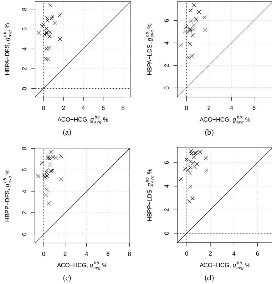
Figure 13.8: Comparison of HBP and ACO-HCG. Each point gives the mean %-deviation from the bb-best solution over 10 independent runs. The symbols denote whether there is statistically significant difference (X) or not (□), or all the runs obtained the same cost (▽).
