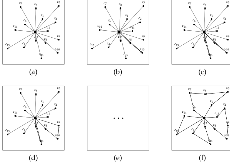
Figure 2.2: Execution of the savings heuristic on a CVRP.
