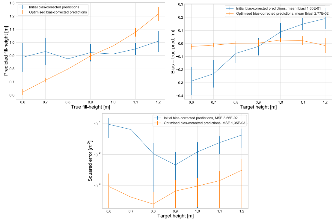
Figure 16. Performance of the optimised detector after stage 1 compared to the initial detector (both shown after the de-biasing process). Heights shown include the space below the passive volume.
