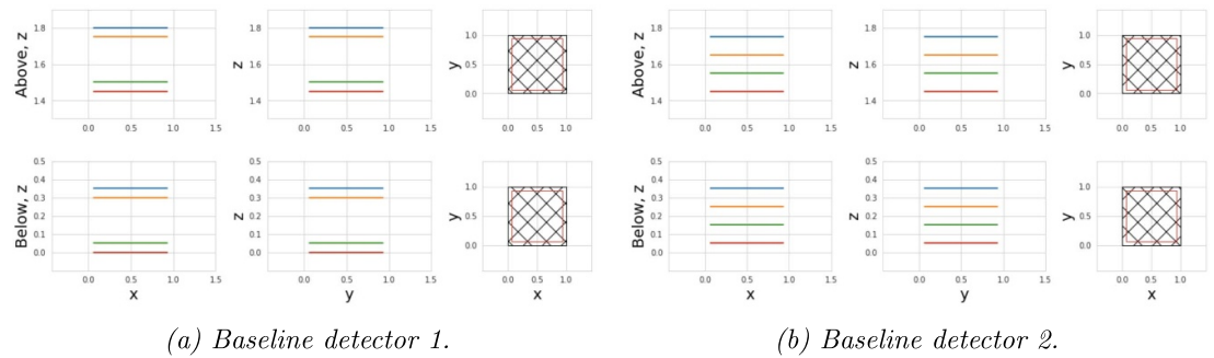
Figure 19. Configurations for the human-designed baseline detectors. The coloured lines/squares indicate the positions and sizes of the panels, and the hatched area indicates the position and size of the passive volume. The top rows indicate panels above the passive volumes, and the bottom rows indicate panels below the passive volume.
