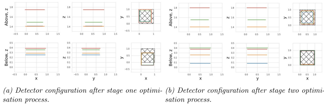
Figure 17. Comparison of detector configurations after stage one (left) and stage two (right) of the optimisation process.
