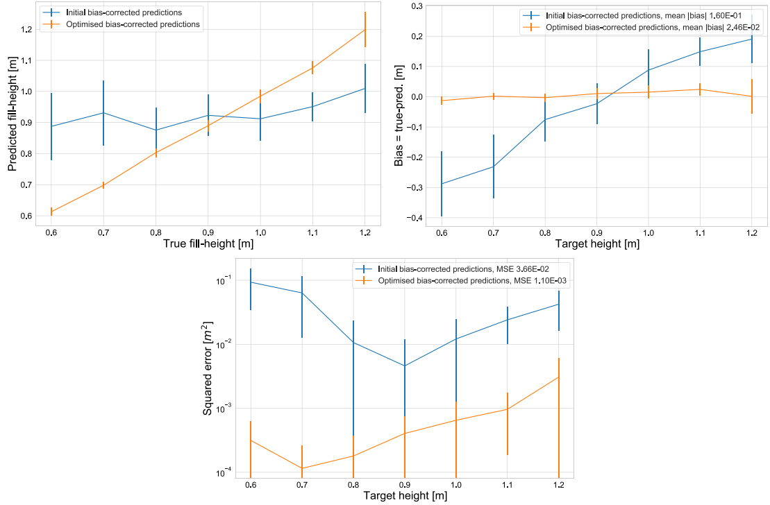
Figure 18. Performance of the optimised detector after stage 2 compared to the initial detector (both shown after the de-biasing process). Heights shown include the space below the passive volume.
