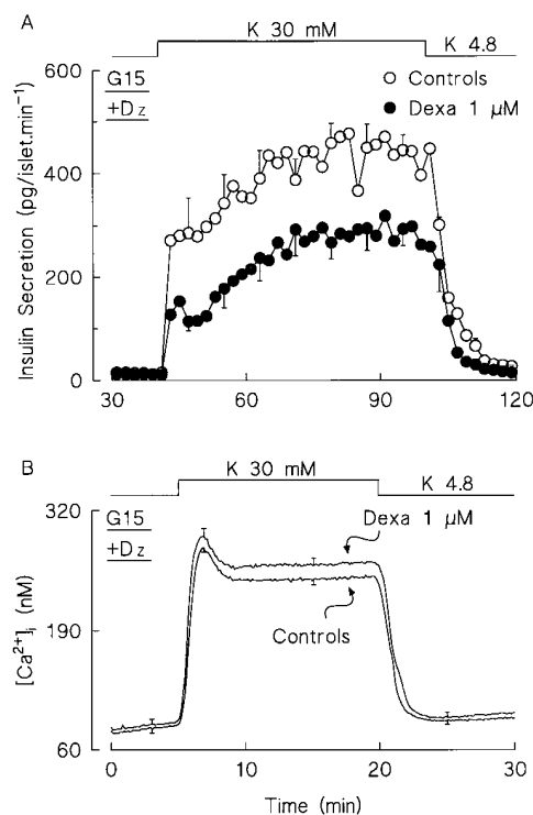
Figure 8. K^+ -induced insulin secretion and [Ca^{2+}]_i changes in islets cultured for 18 h without or with 1 \mu M dexamethasone. (A) Insulin secretion from batches of 20 control or test islets stimulated by high K^+ . The perfusion medium contained 15 mM glucose (G) and 250 \mu M diazoxide (Dz) throughout whereas the concentration of K^+ was raised from 4.8 to 30 mM between 40 and 100 min. Values are means \pm SEM for six experiments. (B) Increase in [Ca^{2+}]_i in islets stimulated by a rise in K^+ concentration from 4.8 to 30 mM between 5 and 20 min. Values are means \pm SEM for 18 islets from three separate cultures.
