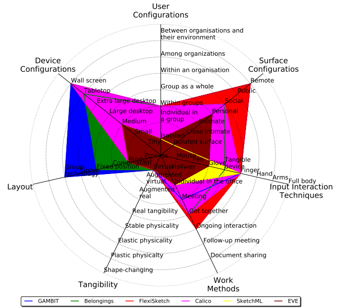
Fig. 13. CROSSIDE instantiations for BELONGINGS, FLEXISKETCH, CALICO, SKETCHML, EVE and GAMBIT all combined at once.
