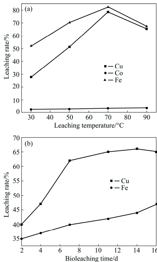
Fig. 5 Influence of temperature on leaching rate in abiotic experiment at pH 1.5, pulp density of 12% (w/v) during 2 h in the presence of 1.5 mol/L H 2 O 2 (a) and bioleaching time on leaching rate in biotic experiment at 33.3 °C, pulp density of 2% (w/v), fraction size of –75 μm, 16 d and redox potential of 350–550 mV (b)
