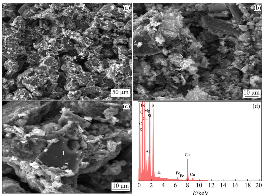
Fig. 9 SEM images (a–c) showing effective alteration of mixed chalcopyrite–chalcocite ore at 33.3 °C, fraction size of -75+53\ \mu\text{m} on day 16, and EDS spectrum of Point 1 in Fig. 9(c) (d)
