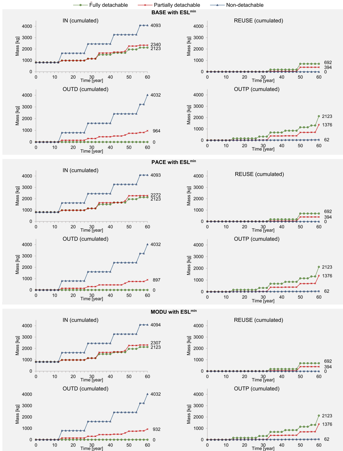
Fig. 8. Evolution of cumulated mass flows for three design options and three connection design, considering minimal Expected Service Life ( ESL_{min} ) values. Compared to ESL_{av} , material flow values increase because building parts have shorter service life values and are thus replaced more often.
