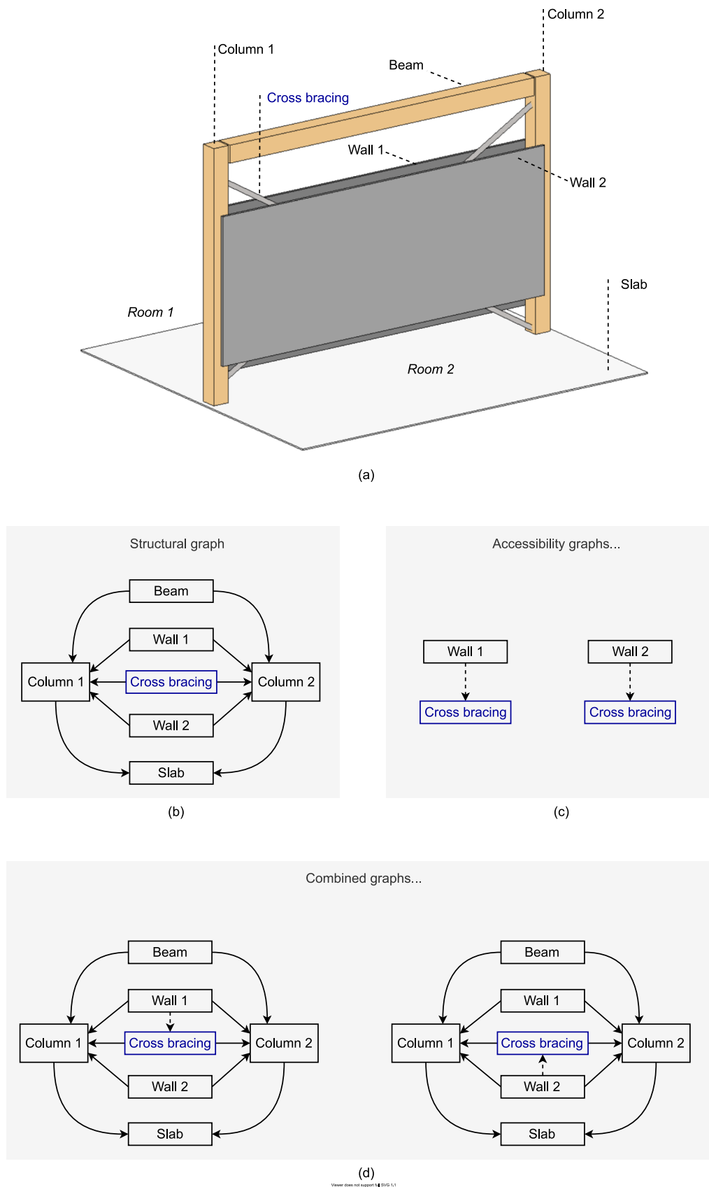
Fig. 2. Modeling interdependencies between building parts as arrows in directed network graphs. Starting from (a) a building model, (b) a structural graph indicates the parts that are attached together (plain line arrows), and (c) two accessibility graphs indicate two alternative ways to access the cross bracing (dashed line arrows). They form (d) two combined directed network graphs showing interdependencies between building parts.
