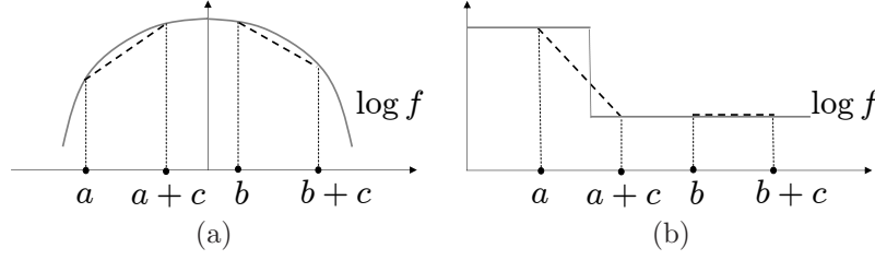
Figure 12.9: Illustration of the condition of Theorem 12.1. The function whose logarithm is presented in (a) preserves the order of opinion, as for any a \leq b and c \geq 0 , there holds \log f(a+c) - \log f(a) \geq \log f(b+c) - \log f(b) . On the other hand no piecewise constant function taking more than one value as in (b) preserves the opinion order, as there exists a \leq b and c \geq 0 such that \log f(a+c) - \log f(a) < \log f(b+c) - \log f(b) holds. In particular, f = 4\chi_{[-\frac{1}{10}, \frac{1}{10}]} + \chi_{[1,1]} used in Figure 12.8 does not preserve the order of opinions.
