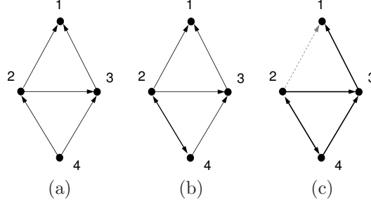
Figure 4.8: The graph represented in (a) is (minimally) persistent in \mathfrak{R}^2 , as can be seen using Theorem 4.7. The graph represented in (b), obtained by adding one additional edge (2, 4) between agents which were already connected by the edge (4, 2) in the opposite direction, is not persistent in \mathfrak{R}^2 . It contains indeed the non-rigid graph (c) as strict min D -subgraph.
