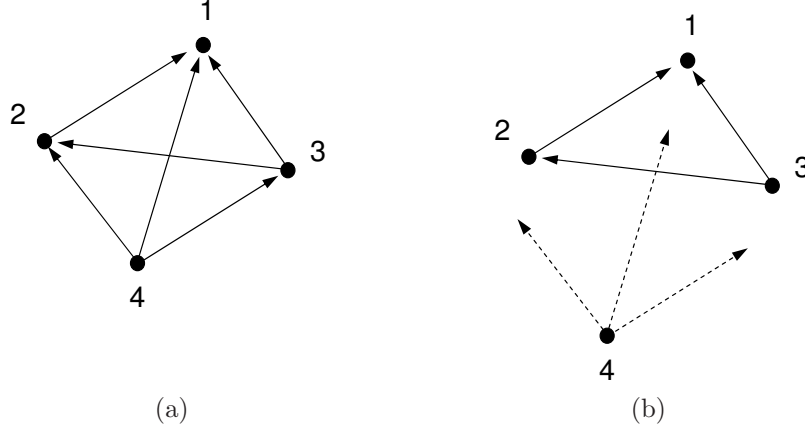
Figure 2.4: Example of 2D-formation whose shape can be maintained although one agent is responsible for three constraints (a). The three constraints of 4 are indeed made compatible by the fact that the constraints of 1, 2 and 3 are sufficient to maintain the shape the triangle (1, 2, 3). The corresponding graph is thus persistent.
