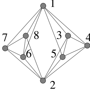
Figure 3.9: Example of a graph satisfying the necessary condition for rigidity of Theorem 3.1 with D = 3 but that is not rigid in \mathbb{R}^3 . The parts of the graphs defined by \{3, 4, 5\} and \{6, 7, 8\} can rotate around the axis defined by the positions of vertices 1 and 2.
