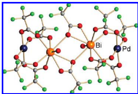
Figure 2. Molecular structure of [\text{Bi}_2\text{Pd}_2(\text{O}_2\text{CCF}_3)_{10}(\text{H}_2\text{O})_2] \cdot 2\text{Me}_2\text{CO} ( 2 ). Acetone molecules and hydrogen atoms of water are omitted for clarity.
