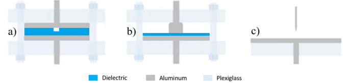
Fig. 7. Configurations of the PD sources generating: (a) internal, (b) surface, and (c) corona PDs.
