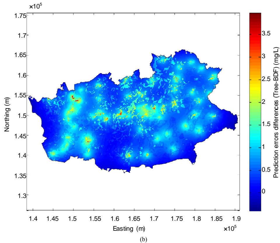
Figure 10. Differences between kriging prediction errors and BDF prediction errors (a) and between the regression tree prediction errors and BDF prediction errors (b).
