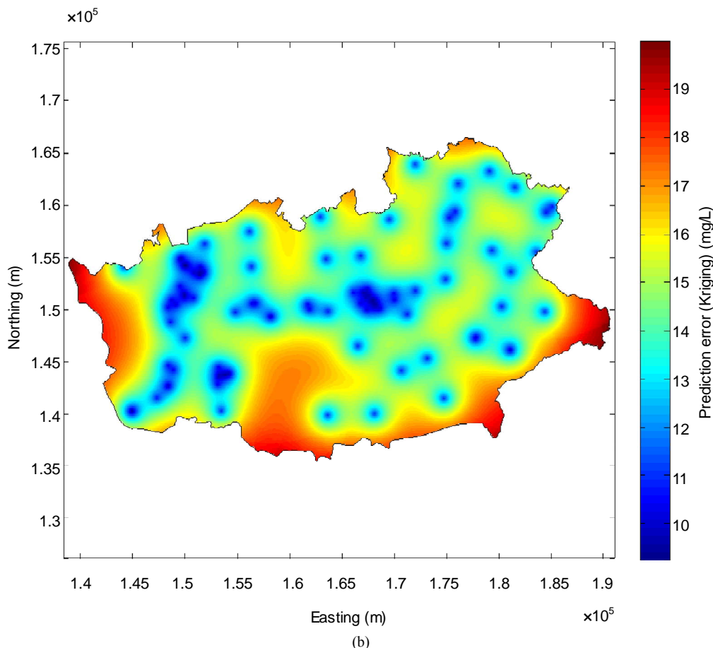
Figure 2. Map of kriged groundwater nitrate concentration (a) and associated prediction error (b). The monitoring stations are symbolized by circles on (a).
