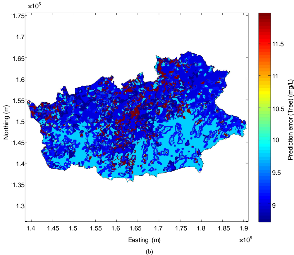
Figure 6. Map of groundwater nitrate concentration predicted by the regression tree model (a) and associated prediction error (b). The monitoring stations are symbolized by circles on (a).
