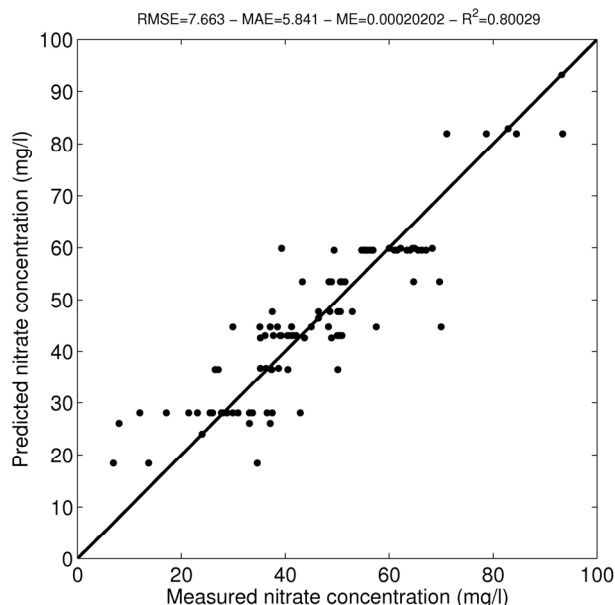
Figure 5. Comparison of the nitrate concentrations predicted with the regression tree model to the measured nitrate concentrations. The plain line represents the 1:1 line.
