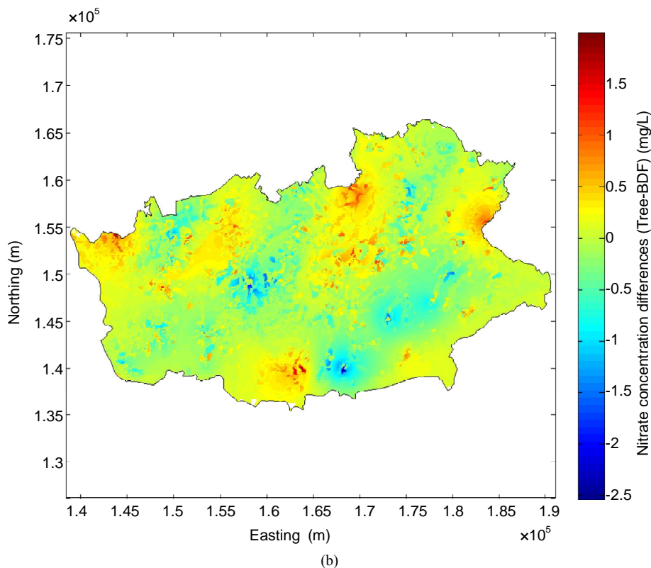
Figure 9. Differences between nitrate concentrations predicted by kriging and BDF (a) and between the regression tree model and BDF (b).
