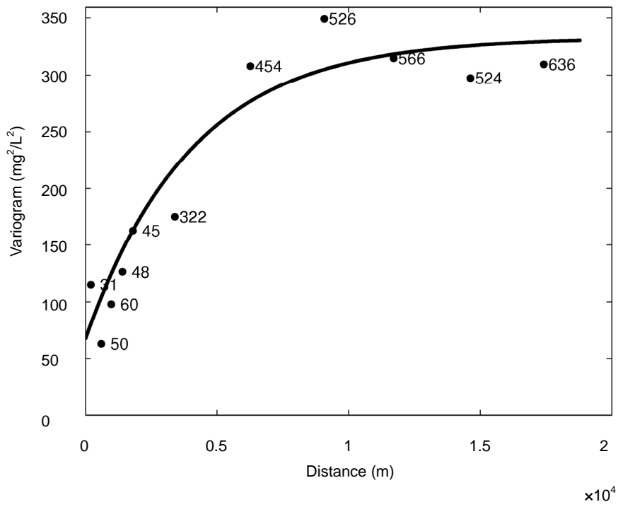
Figure 1. Semi-variogram of the nitrate concentrations in the Brusselian sands estimated on the basis of the dataset of January and February 2009. Dots represent the experimental semi-variogram (together with the number of data pairs on each lag interval), plain line represents the fitted semi-variogram.
