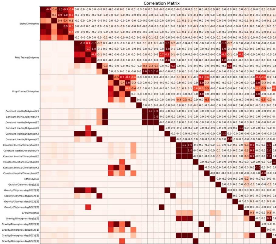
Fig. 32. Correlation matrix of the F2BP pre-impact relaxed simulation for the main parameters of interest. For clarity, some parameters in the correlation matrices are grouped: the state of Dimorphos parameters includes [X, Y, Z, DX, DY, DZ] , the F2BP propagated frame comprises [RA, DEC, W, \omega_X, \omega_Y, \omega_Z] .
