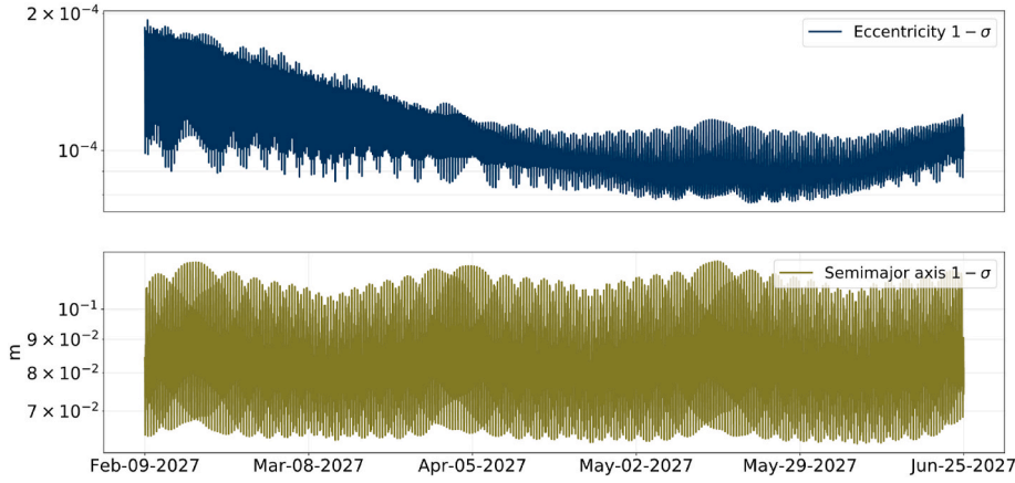
Fig. 23. Expected 1σ accuracy of Dimorphos relative orbit during the nominal mission: eccentricity (upper panel) and semimajor axis (lower panel).
