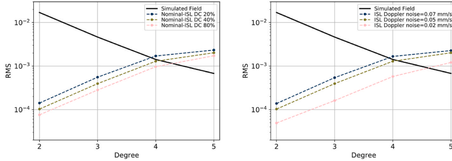
Fig. 20. Power spectra of the simulated Didymos gravity field (black) and of the recovered gravity field uncertainty at the end of the nominal mission for different ISL duty cycles (left plot) and ISL Doppler noises (right plot).
