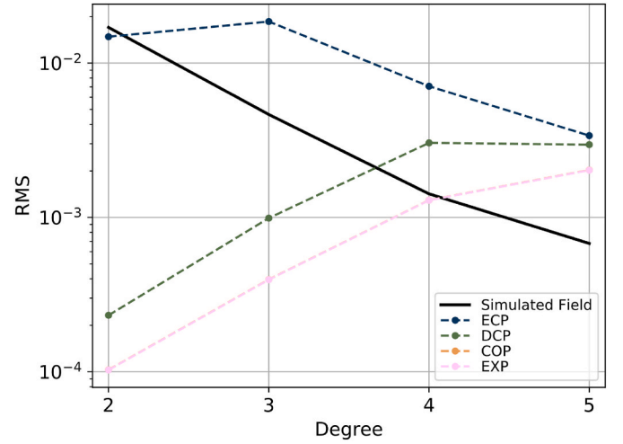
Fig. 19. Power spectra of the simulated Didymos gravity field (black) and of the recovered gravity field uncertainty at the end of each mission phase, considering Hera range-Doppler-opnav and ISL range-Doppler. Early characterization phase (blue); ECP + detailed characterization phase (green); ECP + DCP + close observation phase (orange); ECP + DCP + COP + experimental phase (pink). The EXP curve overlaps with the COP one.
