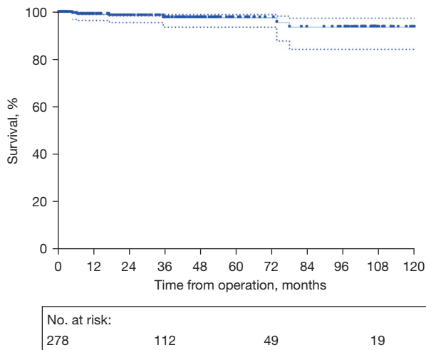
Figure 1 Overall survival.
