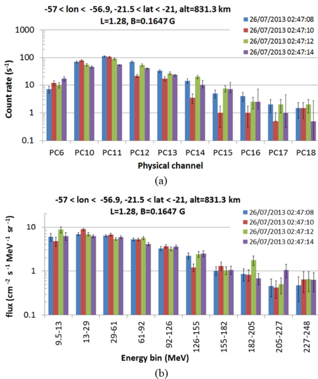
Fig. 19. (a) Counts in the EPT physical channels and corresponding (b) energy differential spectra as measured in the northern part of the SAA.
