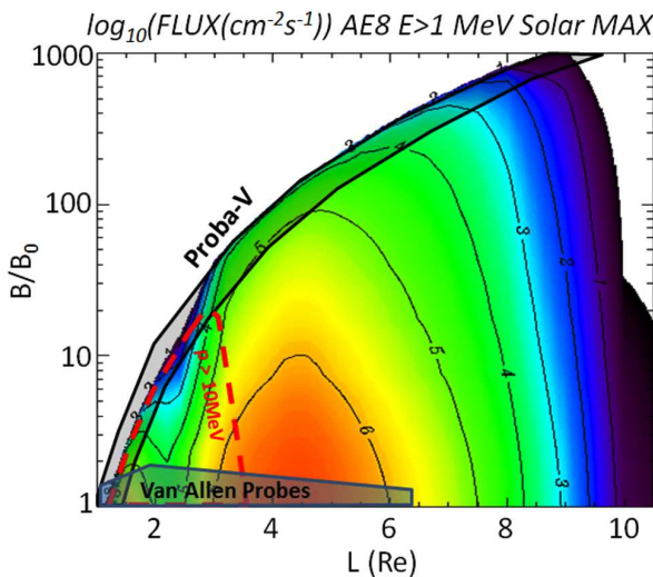
Fig. 12. Invariant coordinate map (L, B/B_0 ) of the AE-8 MAX integral electron flux >1 MeV. The position of the belt of > 10 MeV protons is indicated in red. The region covered by the PROBA-V satellite is indicated in black. For comparison the region covered by the Van Allen Probes (blue) is also shown.
