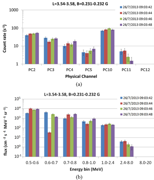
Fig. 17. Physical channel spectrum a) and energy differential spectrum (virtual channel spectra) b) as measured close to the slot region (Geographic location: latitude= -56.3°±0.2°, longitude= 12.3°±1°; altitude= 829.6km).
