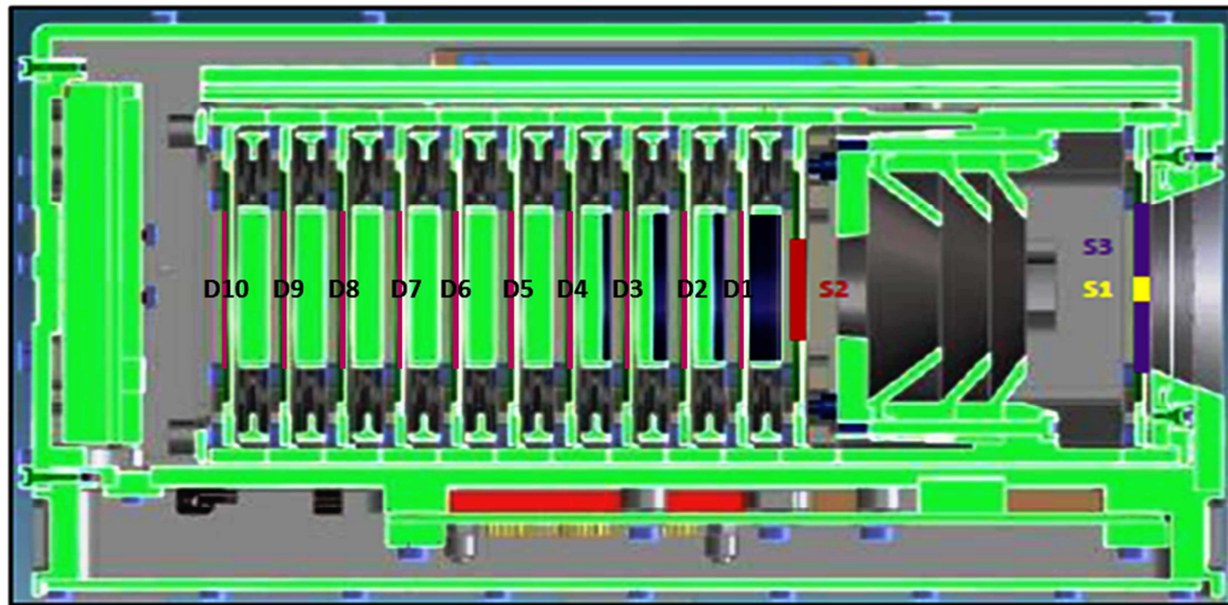
Fig. 2. Cross section view of the EPT instrument showing the collimator and the sensor layout. The S1, S2 and S3 detectors that define the 52° F.O.V angle are highlighted, as well as the 10 DAM detectors defining the High Energy Section (HES). ¶
