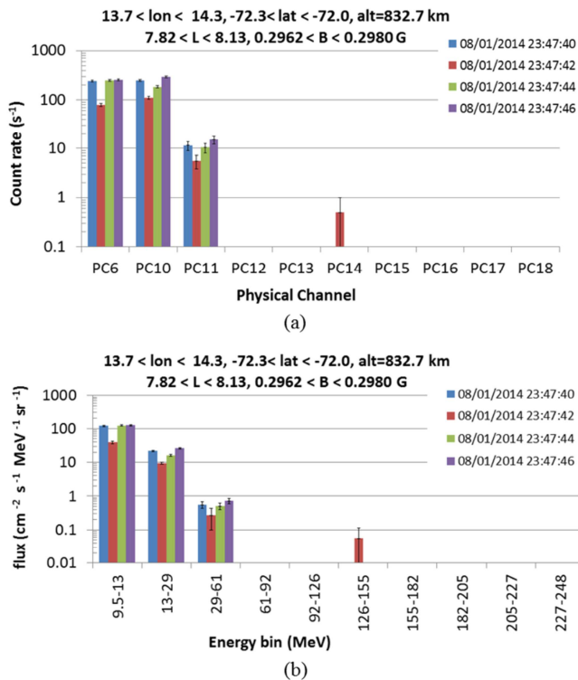
Fig. 21. Physical channel spectrum and energy differential spectrum (virtual channel spectra) as measured at high latitude during a SEP event.
