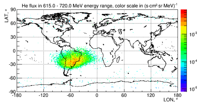
Fig. 22. World map (bin resolution 1^\circ \times 1^\circ ) of average He-ion flux in the 615-720 MeV energy range measured by the EPT from 21 May 2013 to 20 November 2013.
