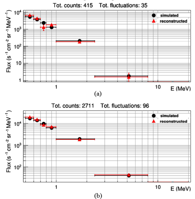
Fig. 13. Examples of comparison between original electron spectra as given by the SPENVIS tool (black dots) and reconstructed spectra (red triangles) as deduced from PC counts. The total number of counts available for spectrum reconstruction is indicated on top of each graph as well as the sum of the fluctuations of the counts in channels with regard to a poissonian distribution.
