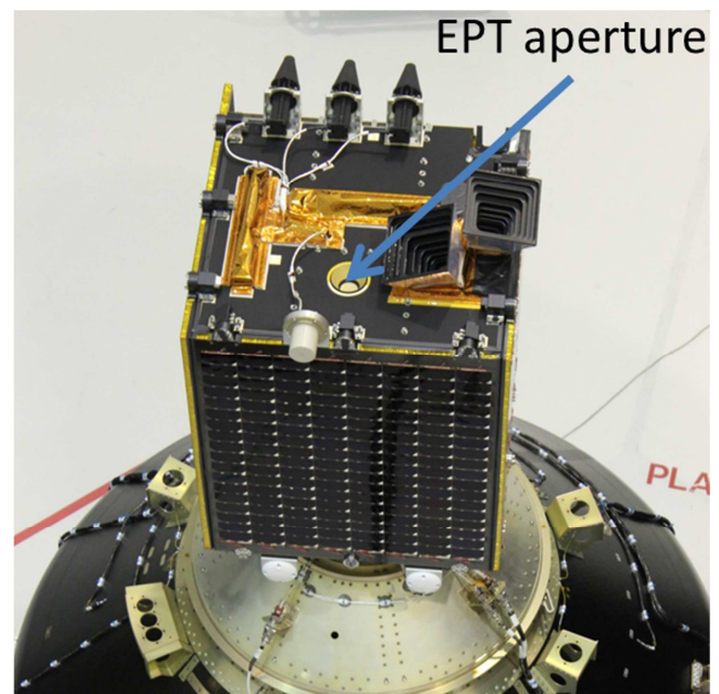
Fig. 11. View of the PROBA-V satellite mounted on the launcher with tagged EPT aperture.
