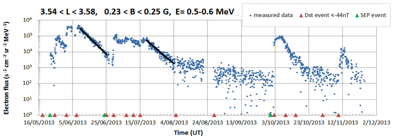
Fig. 18. Differential flux in the energy bin 0.5-0.6 MeV (blue dots) as a function of time for an indicated (L,B) bin. No averaging was done. The spread in data is mainly due to the spread of the counts in the unfolded spectra. The green triangles show the time of occurrence of a solar energetic particle event and the red triangles show the time of Dst minimum when a geomagnetic event occurred (only if Dst was below -44nT).
