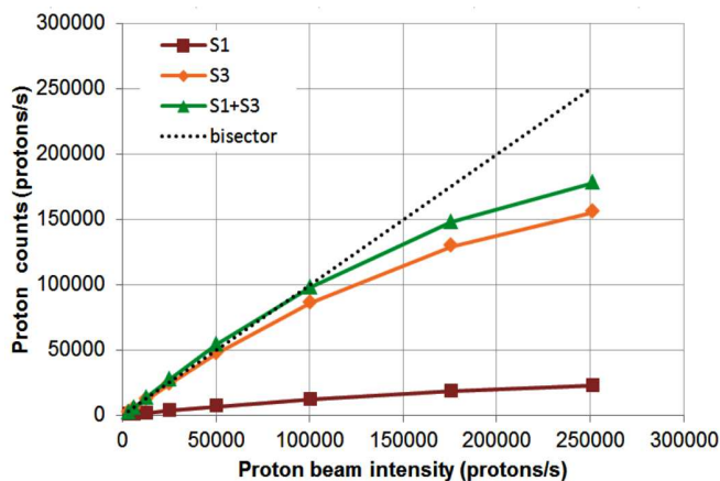
Fig. 4. EPT measured counts (50 th - percentile) as a function of 103 MeV proton beam intensity.
