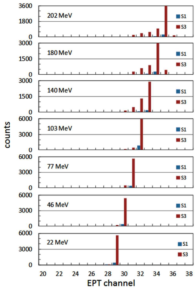
Fig. 9. Detection of protons with various incident energies in the different EPT channels.
