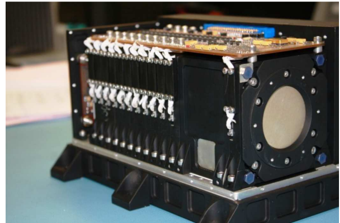
Fig. 1. Picture of the EPT FM instrument with cover removed.
