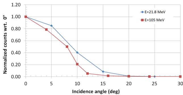
Fig. 10. Angular variation of EPT counts for 21.8 and 105 MeV protons.
