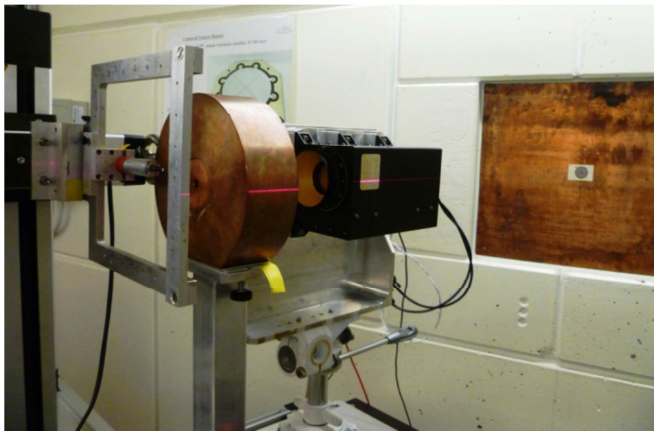
Fig. 3. Image of the experimental set-up showing the diode-based intensity monitor, the 7 cm thick collimator and the EPT.
