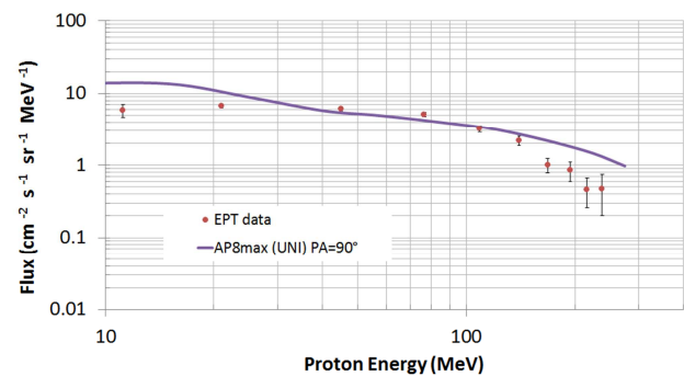
Fig. 20. Single proton spectrum measured by the EPT on 26 July 2013 with 91^\circ average pitch angle, as compared to prediction of AP8-MAX Unidirectional for position: -21.5^\circ LAT, -56.9^\circ LON, 831.3km ALT).
