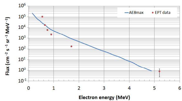
Fig. 16. Comparison between the differential flux as predicted by AE8MAX model and EPT results on 4th October 2013 (Geographic location: longitude= 46.9^\circ , latitude= -55.8^\circ ; altitude= 831.2 km).
