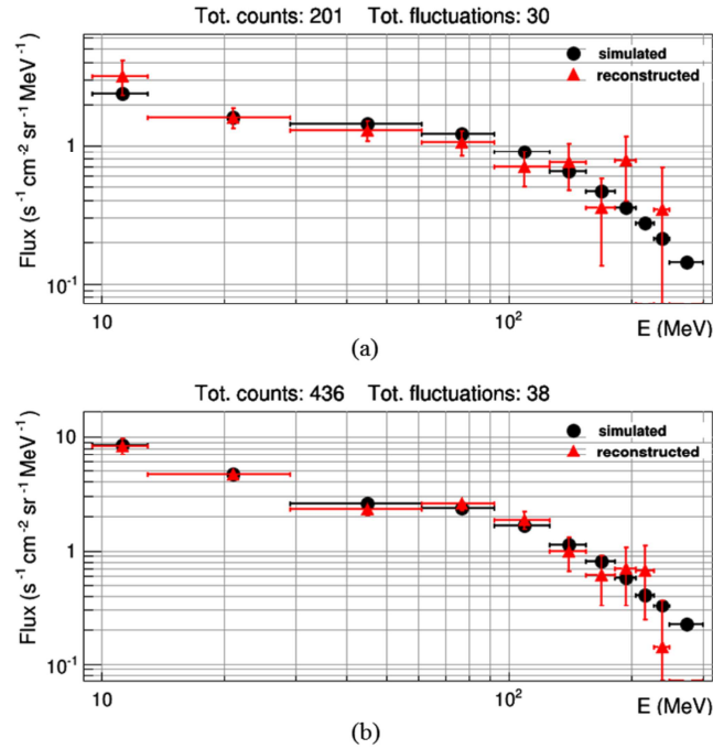
Fig. 14. Same as in Fig. 13 but in case of protons: comparison between original simulated proton spectra (black dots) and reconstructed spectra (red triangles).
