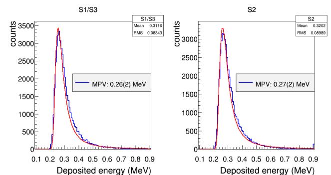
Fig. 5. Histograms of counts as a function of energy deposited in S1/S3 and S2 sensors (blue) with fits by a Landau distribution (red): The Most Probable Value (MPV) is shown in the insets along with their uncertainties.
