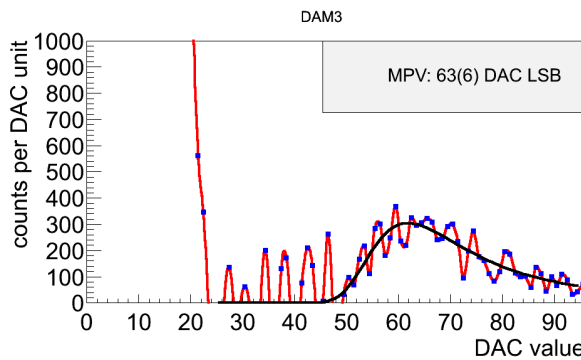
Fig. 7. Experimental spectrum (red line, blue dots) representing differential counts as a function of energy deposited by 203 MeV protons in the DAM-3 (expressed in DAC value) with Landau distribution fit (black).
