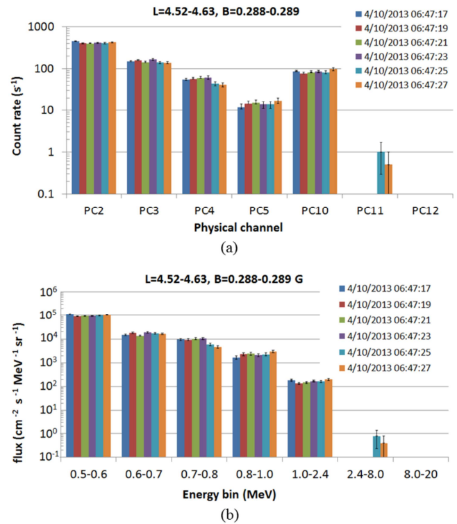
Fig. 15. a) Physical channel spectrum and b) energy differential spectrum (virtual channel spectra) as measured in the outer radiation belt (Geographic location: longitude= 47.0 \pm 0.2^\circ , latitude= -55.6 \pm 0.3^\circ ; altitude= 831.2 km).
