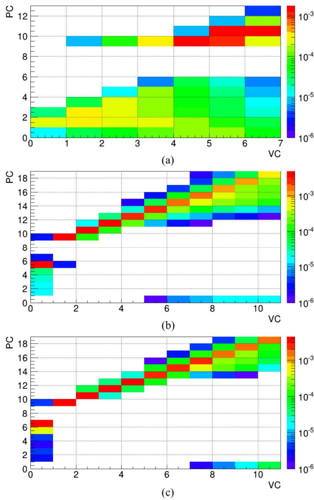
Fig. 8. Graphical representation of the particle efficiency matrices: a) electrons, b) protons, c) He-ions.
