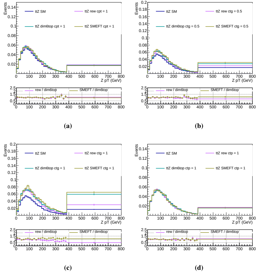
Figure 6.18: Comparison of the reweighted t\bar{t}Z MC distribution with the response of dim6top and SMEFT-LO for (a) c_{pt} = 1 , (b) ct_G = 0.5 , (c) ct_G = 1 and (d) ct_p = 1
