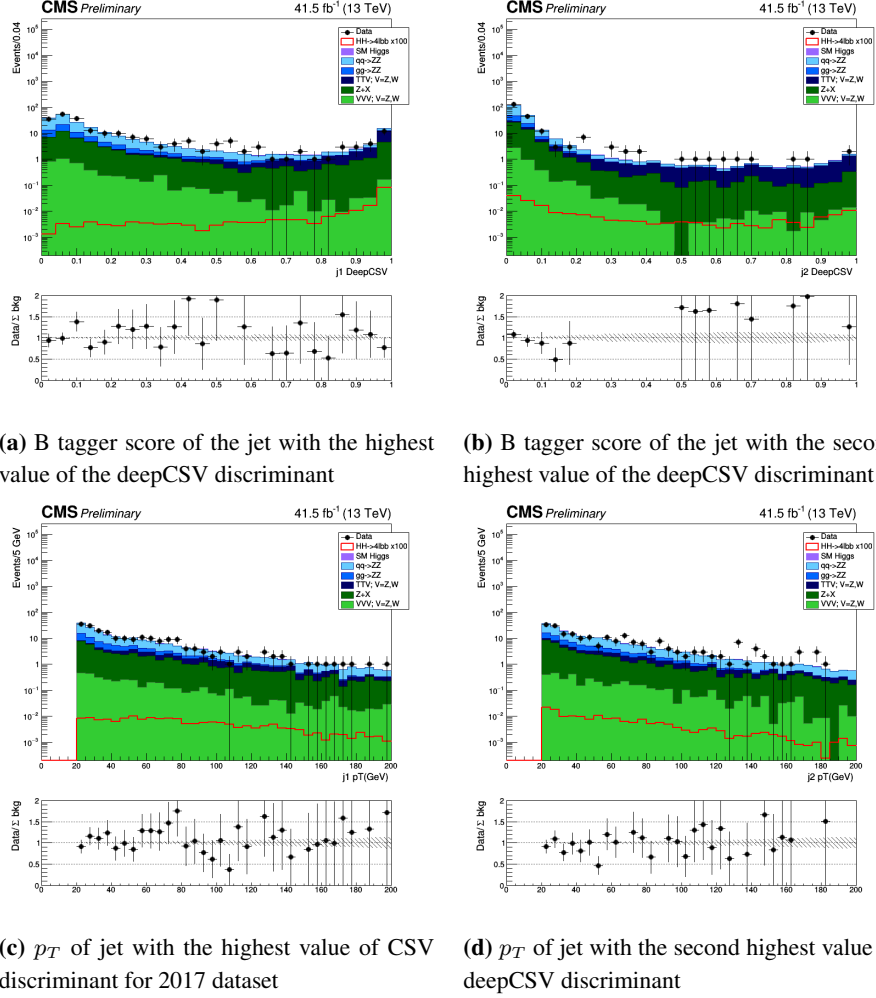
Figure A.3: Four-lepton + 2jets sideband plots for 2017 datasets.
