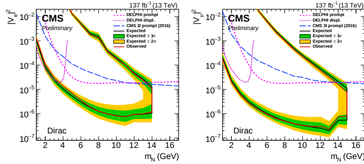
Figure 5.5: Exclusion region at 95% CL in the |V_{Ne}|^2 (left), |V_{N\mu}|^2 (right) as a function of m_N for a Dirac HNL. Results from the Delphi [89] and the CMS [90, 91] Collaborations are shown for reference.
