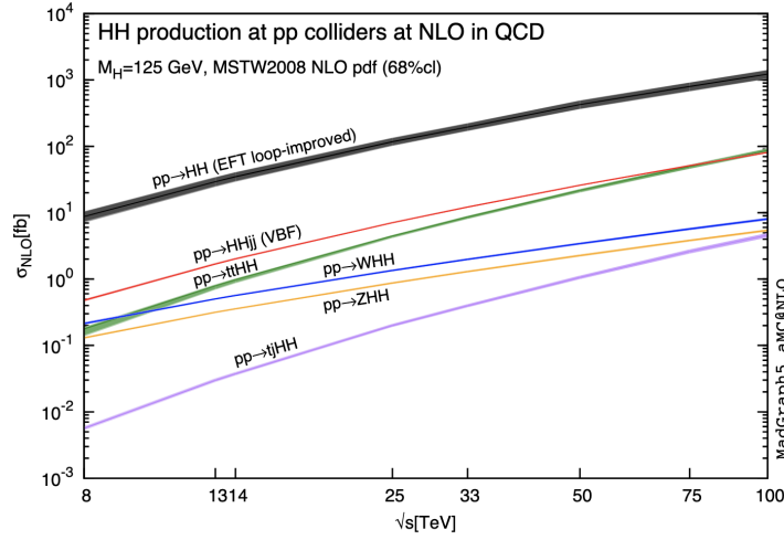
Figure 1.14: Di-Higgs production mechanism at LHC as a function of the center of mass energy [9]
