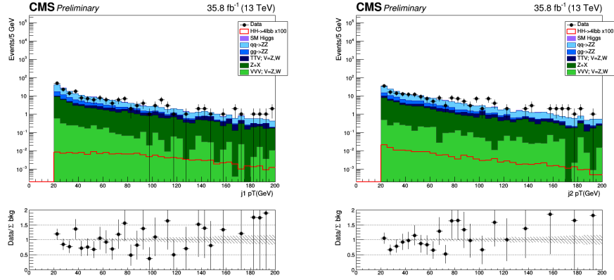
(c) p_T of jet with the highest value of CSV discriminant for 2016 dataset
