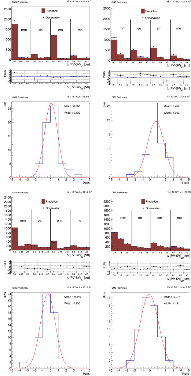
Figure 5.21: Pulls for CR1 as a function of displacement for each flavor. We show the prediction for 2016 separately (top) and for 2017+2018 (bottom), with plots for the low mass PFNs on the left and the high mass PFNs on the right, OS and SS categories are merged together.
