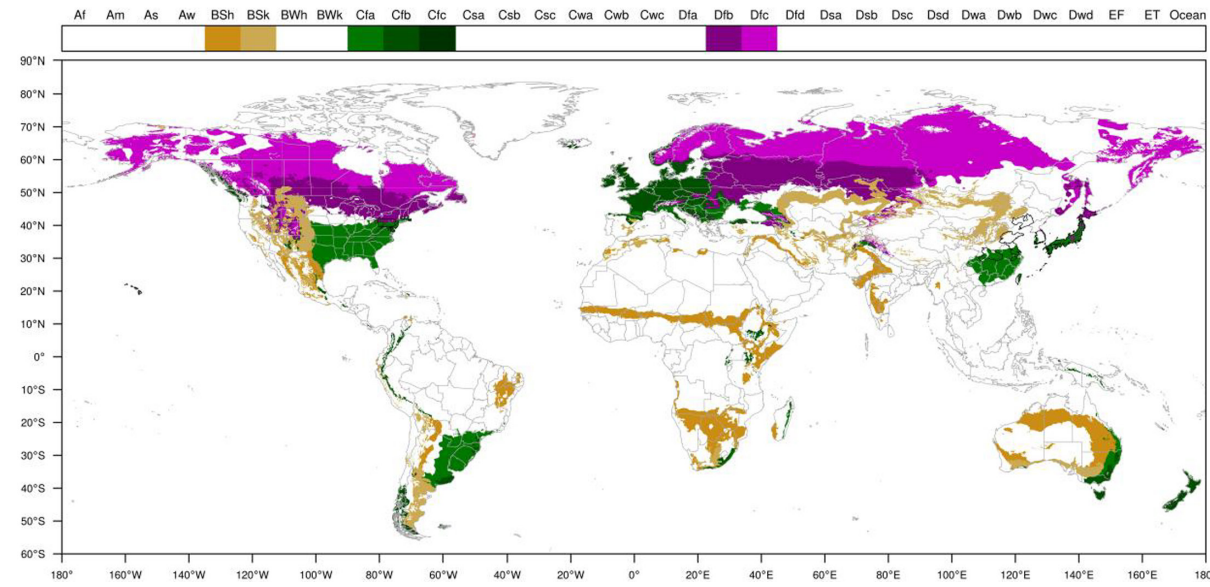
FIGURE 6 Distribution of Köppen–Geiger climate types that occur in the EU and in areas where Lepidosaphes pini has been reported.
