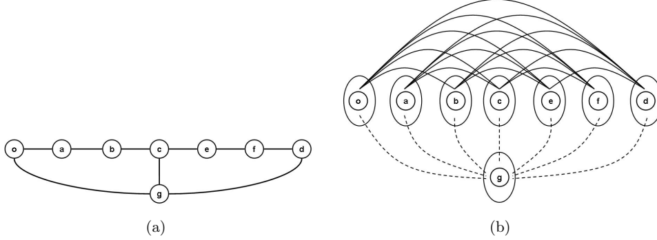
Figure 4: New inequality for L = 5 .
