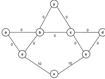
Figure 2: Graph obtained from \overline{Z}
