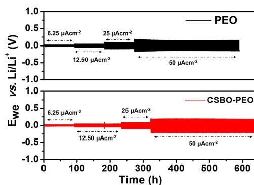
Figure 3. Galvanostatic charge–discharge voltage profiles for stripping–plating at various current densities at 60 °C with Li|SPE|Li symmetric cells. SPEs are PEO (top) and CSBO/PEO 50:50 wt/wt (bottom), both SPEs loaded with 20 wt % LiTFSI.
