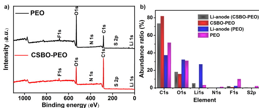
Figure 5. (a) Survey spectrum of the Li anode of PEO and the CSBO–PEO SPE-based Li–LFP cells after 100+ cycling and (b) abundance ratio percentage of surface elements constituting SEI for the Li anode and corresponding SPE membranes.
