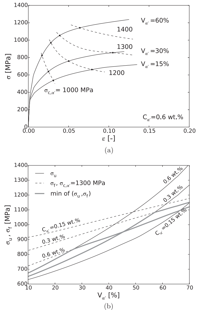
Fig. 9. (a) Locus of fracture, as predicted by a maximum principal stress criterion in the martensite, for varying values of the martensite critical stress \sigma_{c,\alpha'} . (b) Evolution of the tensile strength \sigma_u (black solid lines) and the fracture strength \sigma_f (dashed lines) with the volume fraction of martensite V_{\alpha'} . Grey lines indicate the maximum reachable stress.
