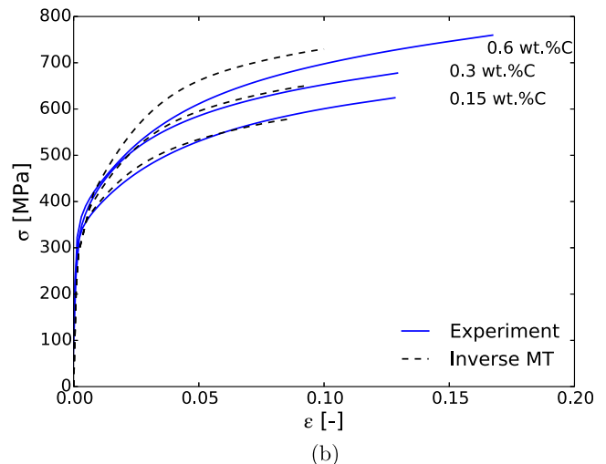
Fig. 11. Model predictions obtained with (a) the direct Mori–Tanaka scheme and (b) the inverse Mori–Tanaka scheme for V_{\alpha'} = 15\% . In each case the ferrite hardening parameters were fitted to obtain the best prediction in a least-squares sense.
