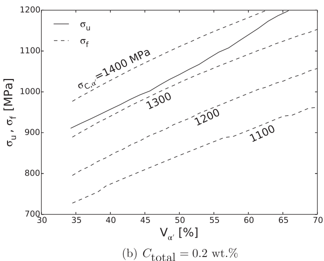
Fig. 10. Evolution of the tensile strength \sigma_u (black solid line) and fracture strengths \sigma_f (dashed lines) with the volume fraction of martensite V_{\alpha'} , for varying martensite critical stress \sigma_{c,\alpha'} .
