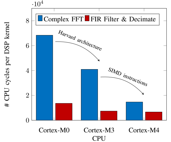
FIGURE 2. CPU cycles required for a Q16 complex 256-point FFT and a FIR filtering and decimation of 260 Q16 complex samples (63 taps, decimation factor of 52) for three low-power ARM Cortex-M CPUs.
