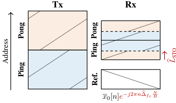
FIGURE 6. Organization of the buffers in DMEM for LoRa Tx ( f_s = 2B ) and Rx (Nyquist rate, after decimation by the DFE) chains. The gray lines in the buffers show the instantaneous frequency of the modulated chirps.
