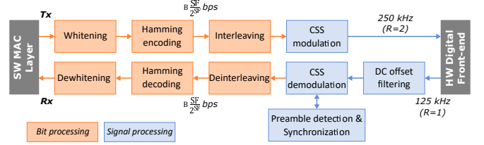
FIGURE 5. Block diagram of the LoRa DBB processing for B = 125 kHz.
