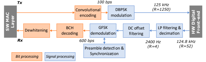
FIGURE 7. Block diagram of the Sigfox DBB processing.
