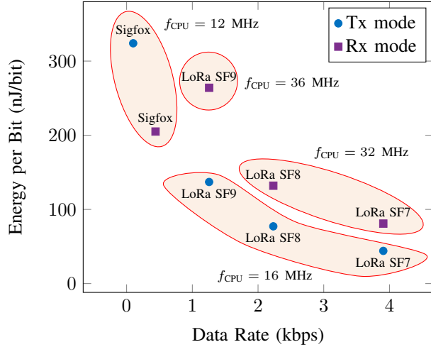
FIGURE 9. Minimum CPU frequency and average energy required by the LoRa and Sigfox SDRs for processing an information bit in the DFE and the DBB.
