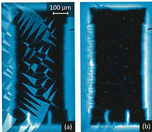
FIG. 2. Illustration of the correction of the indicator magnetic domains in a MO image. (a) Original raw image of a 800 \times 400 \mu\text{m}^2 Nb superconducting film at T = 3.6 \text{ K} and \mu_0 H = 2.1 \text{ mT} , 31 where the triangular artifacts pollute the intensity map. (b) Image after treatment with the correction algorithm, showing an enhanced contrast of the intensity map.
