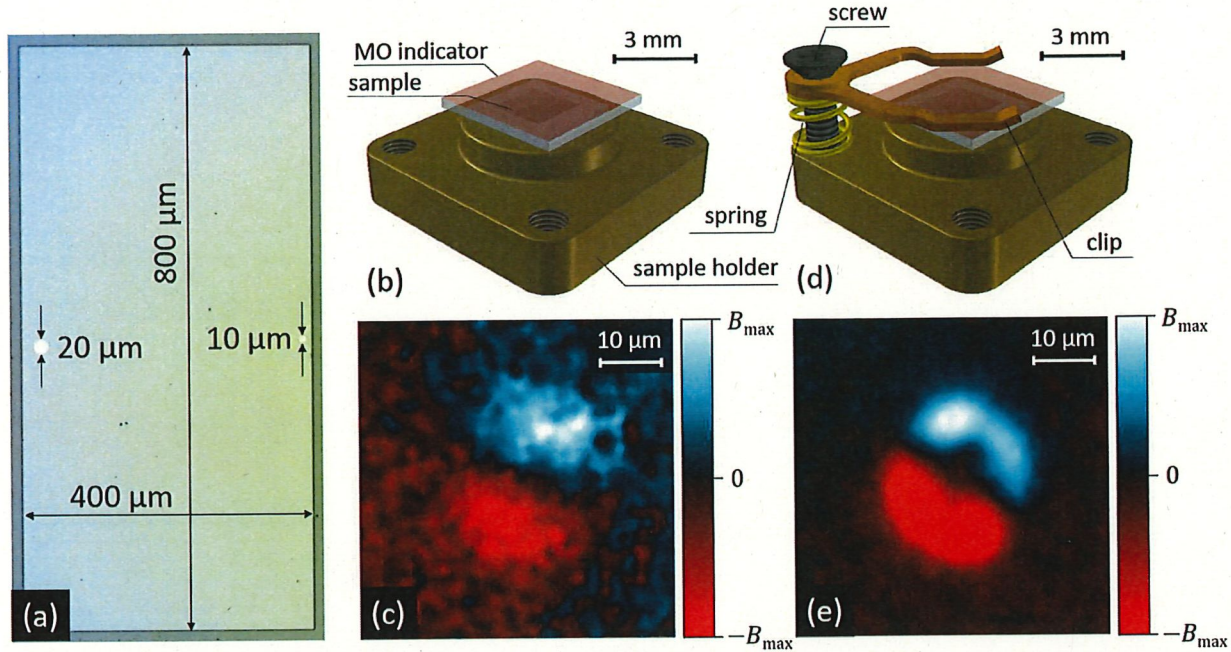
FIG. 4. Sample layout and mounting for the Nb film with Co disks. (a) Optical image of the 800 \times 400 \mu\text{m}^2 Nb film (100 nm thick), where the two 30 nm thick Co disks with a diameter of 20 \mu\text{m} and 10 \mu\text{m} are located at 20 \mu\text{m} and 10 \mu\text{m} , respectively, from the sample edge. (b) Classical configuration for the MOI measurements, with the sample mounted on top of the sample holder, and the indicator placed on top of it. (c) MO image of the 20 \mu\text{m} diameter Co disk after polarization with an in-plane field of 3 mT, in the configuration of panel (b). (d) Alternative configuration where the indicator is pressed closer to the sample surface with a purposely designed metallic clip. (e) MO image of the same disk as in panel (c) showing the enhanced MO signal using the alternative configuration presented in (d).
