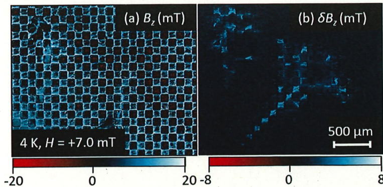
FIG. 9. Flux avalanches in Nb/NdFeB at 4 K. (a) Image of the B_z distribution converted from the MO image obtained at 7 mT, while increasing \mu_0 H from 0 mT after zero-field cooling the sample to 4 K. (b) Differential image showing the \delta B_z map in response to a 0.1 mT change in \mu_0 H at 7 mT.
