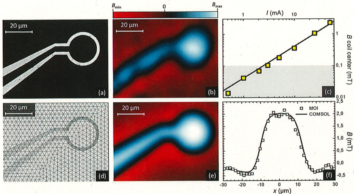
FIG. 6. Quantitative magneto-optical imaging on a planar coil. (a) Scanning electron microscope image of the 50 nm-thick coil made of Al. The coil has an inner and outer radius of 10 \mu\text{m} and 12 \mu\text{m} , respectively. (b) Magnetic field of the coil fed by a current I = 50 mA, obtained by MOI with the MO indicator pressed on the sample surface. (c) Magnetic field B_z at the center of the coil as a function of I . The error on the magnetic field value of a single pixel is around 0.1 mT, but for extended sources such as the coil, the correlation between pixels gives a lower detection threshold of 0.01 mT. (d) Mesh for the numerical simulations. (e) Magnetic field of the coil fed by a current I = 50 mA, obtained by numerical simulations, at a distance z = 6 \mu\text{m} of the sample surface. (f) Magnetic field profile through the center of the coil for I = 50 mA taken in the MO image of panel (b) and in the numerical simulation for z = 6 \mu\text{m} .
