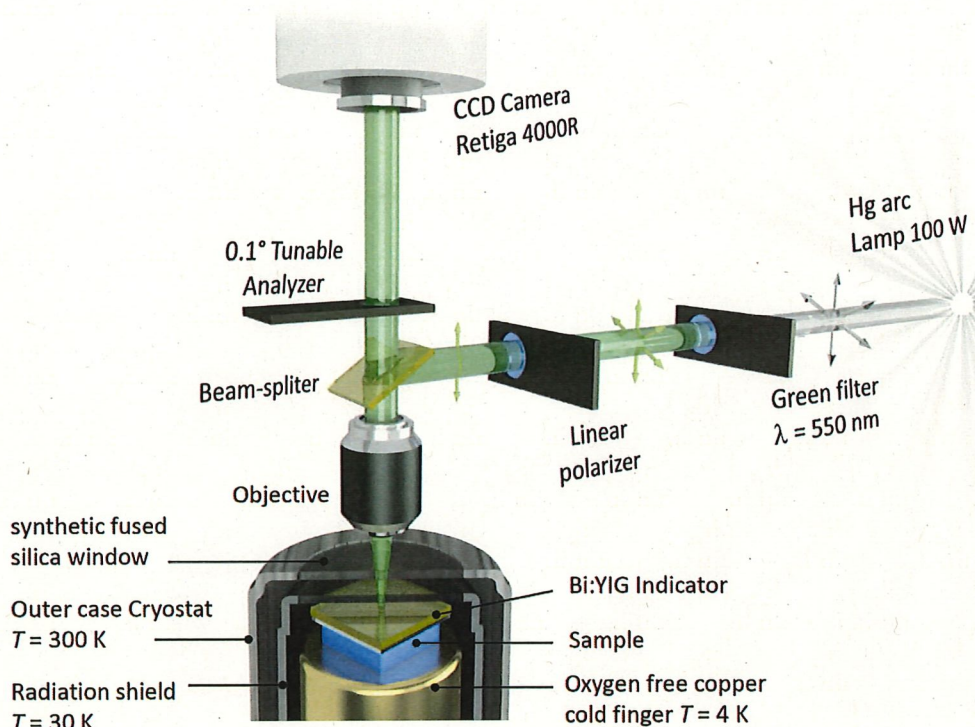
FIG. 1. Schematic of the MOI setup (cf. text for details).
