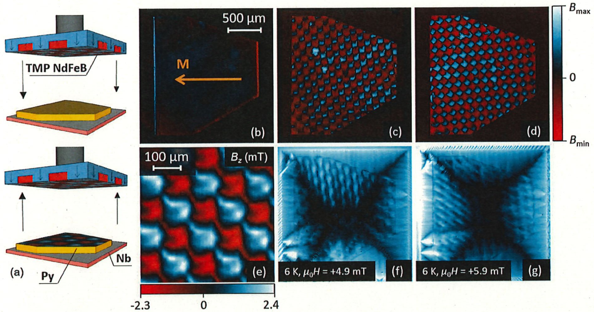
FIG. 10. Imprinting the micromagnetic pattern in the permalloy. (a) Schematic showing the imprinting process. (b) Py/Nb sample magnetized in-plane with the magnetization direction indicated by the arrow. [(c) and (d)] Py/Nb sample with the micromagnetic pattern imprinted in the Py layer. (c) Chessboard pattern aligned roughly along the long side of Py. (d) Chessboard pattern at \sim 45^\circ with respect to the long side. (e) SHPM image at room temperature showing a part of the chessboard pattern in the Py layer of panel (c), obtained at a scan height z \sim 4 \mu\text{m} . [(f) and (g)] MO Images showing smooth flux penetration at 6 K in the Py/Nb sample with the imprinted patterns shown in (c) and (d), respectively. These images are obtained by subtracting the image at \mu_0 H = 0 \text{ mT} in each set to remove the signal from the magnetic pattern. Images in (f) and (g) are at \mu_0 H = 4.9 \text{ mT} and 5.9 \text{ mT} , respectively. Both images were obtained while increasing \mu_0 H from 0 mT after zero-field cooling the sample to 6 K.
