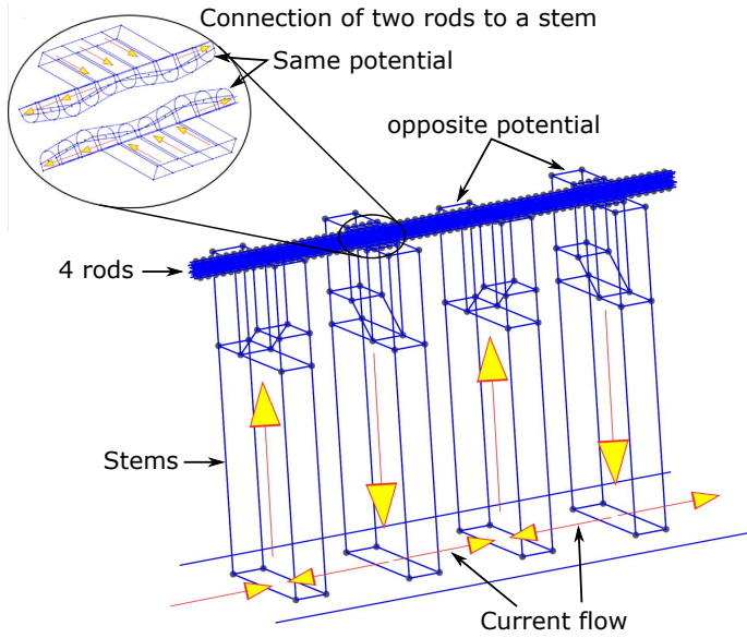
Figure 2.4: Four-rod RFQ supported by stems
