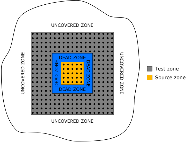
Figure 4.4: Definition of the different domains.
