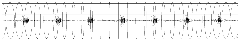
Figure 6.27: Transversal beam dynamics view.
