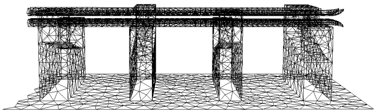
Figure 4.11: Accelerator mesh used for the low-frequency preconditioner test.
