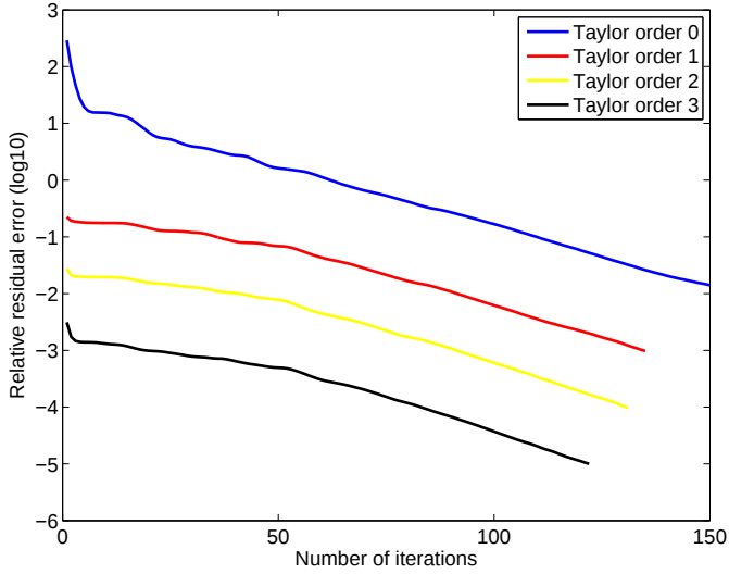
Figure 4.22: Convergence of GMRES with the low-frequency preconditioner - The accuracy for each Taylor order approximation is set according to the criterion defined by Eq. 4.167 and Eq. 4.168.
