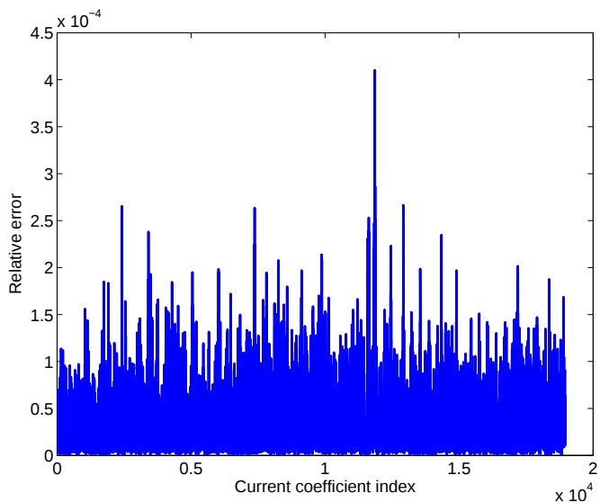
Figure 4.20: Relative current error between the brute force solution and the FNFMMs solver solution with the low-frequency preconditioner.
