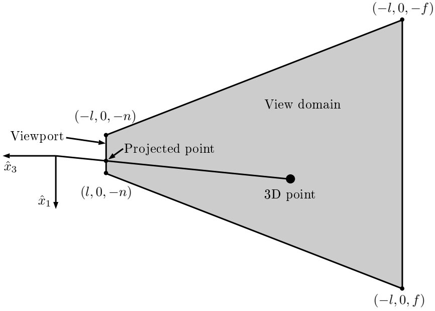
Figure 5.2: Projection principle.
