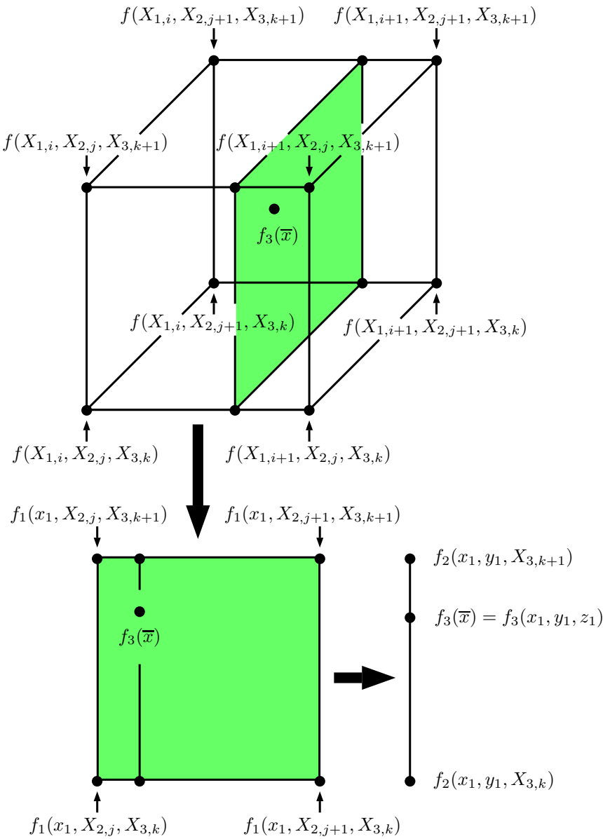
Figure 10.1: 3-linear Lagrangian interpolation for a 3 dimensional vector space.
