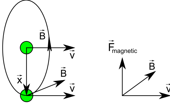
Figure 2.5: Magnetic field due to space charge.
