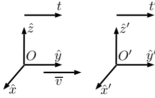
Figure 10.2: Example of two inertial frames
