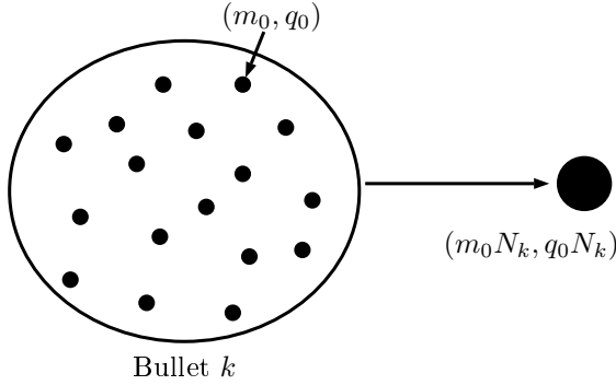
Figure 6.2: Macro-particle approximation.
