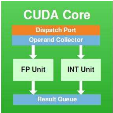
Figure 5.5: Cuda CORE hardware [69].
