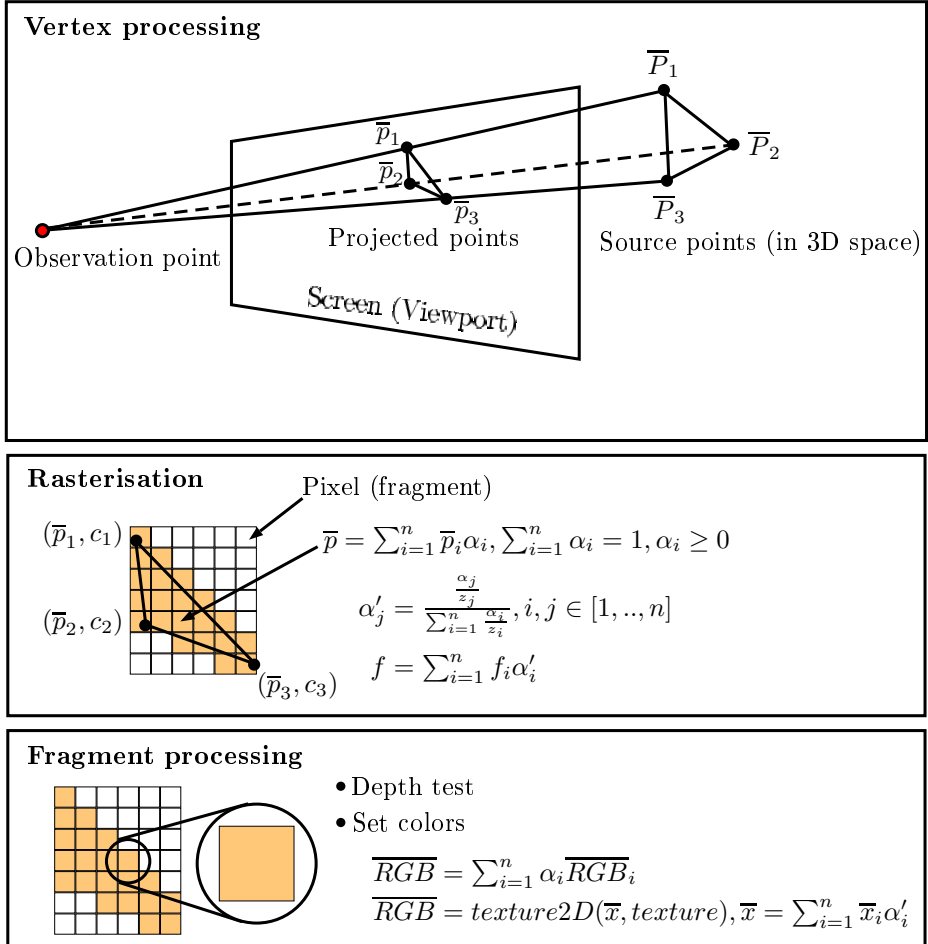
Figure 5.1: Rasterisation principle.
