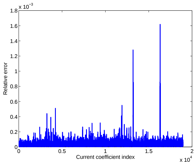
Figure 4.17: Relative current error between the brute force solution and the FNFMMs solver without any low-frequency preconditioner.
