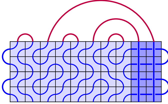
Figure 1: Typical configuration of a logarithmic minimal model. For the \mathcal{LM}(1, 2) model, \beta = 0 and closed loops are thus forbidden. Since the nonlocal degrees of freedom are connectivities, the transfer matrices act on link states which keep track of the planar connectivities. Here the (r, s) = (1, 3) boundary condition is applied so that there are s - 1 = 2 defects propagating in the bulk.
