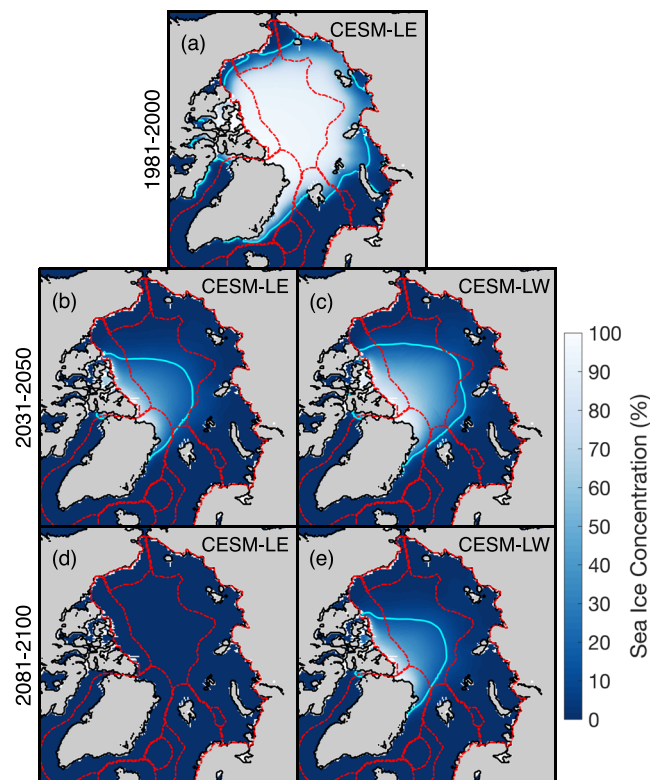
Figure 3. Average September sea ice concentration for the CESM-LE over the period of (a) 1981–2000 and for (b, d) the CESM-LE and (c, e) the CESM-LW over the periods of (b, c) 2031–2050 and (d, e) 2081–2100. The borders of the EEZs are indicated by red lines. The cyan line shows the 15% sea ice concentration contour.
