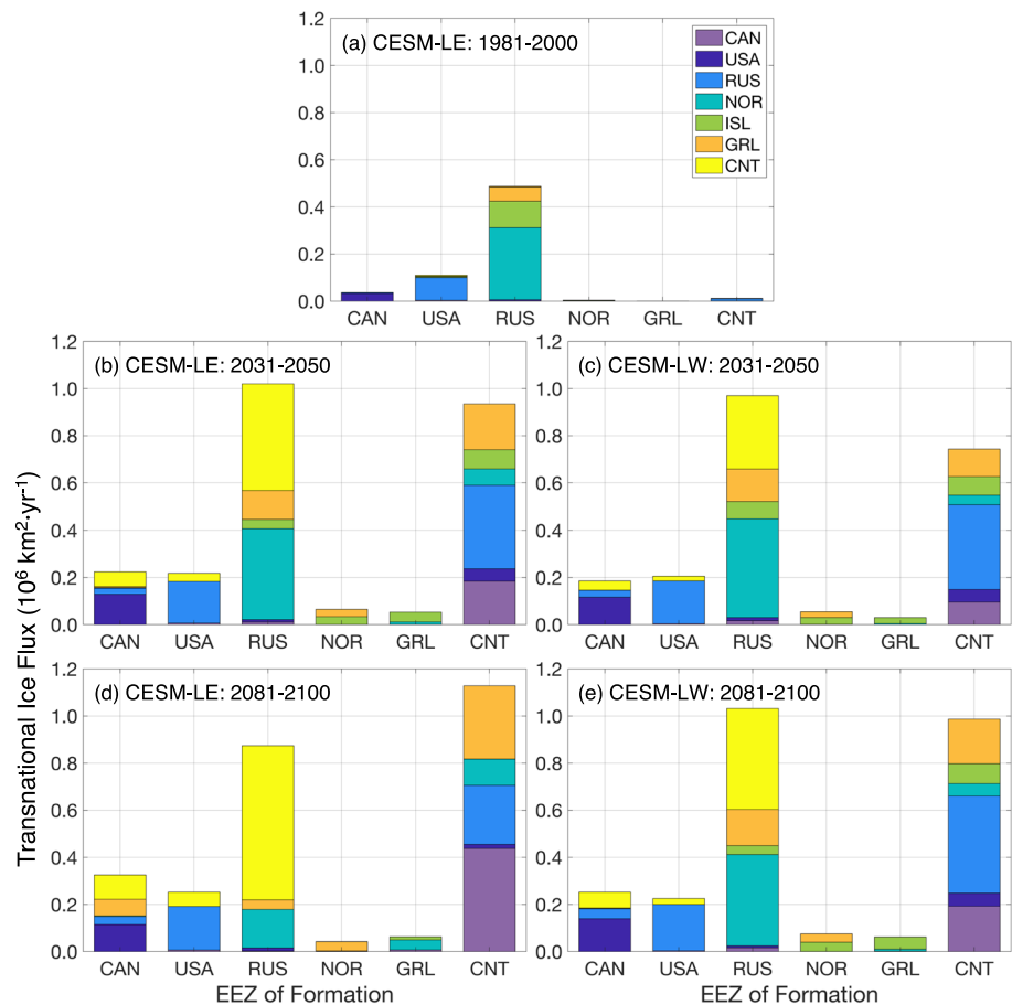
Figure 4. Annual mean average areal flux of transnational ice for the CESM-LE over the period of 1981–2000 (a) and for the CESM-LE (b, d) and the CESM-LW (c, e) over the periods of 2031–2050 (b, c) and 2081–2100 (d, e). The height of each colored portion within one bar represents the annual mean areal flux of ice between the EEZ of formation (x axis) and the EEZ of melt (color). Note that domestic ice is not included in this figure in order to focus on the features of transnational ice exchange. The average amount of ice area exchanged between all EEZs, including domestic ice, for both experiments and a statistical assessment of the pathways that are significantly different between the CESM-LE and the CESM-LW can be found in Tables S1 and S2 in the supporting information.
