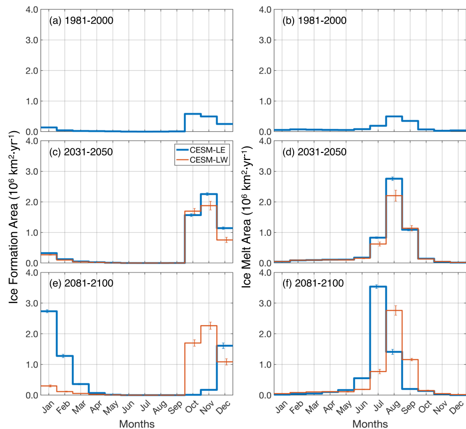
Figure 7. Annual cycle of areal ice formation (left) and melt (right) for the periods of 1981–2000 (a, b), 2031–2050 (c, d), and 2081–2100 (e, f) in the CESM-LE (blue) and the CESM-LW (orange). The error bars show the 95% confidence intervals of the 20-yr averaged ice formation/melt area for each month across the 40 ensemble members of the CESM-LE and the 11 ensemble members of the CESM-LW. Only ice floes that formed and melted between the specified time periods are considered.
