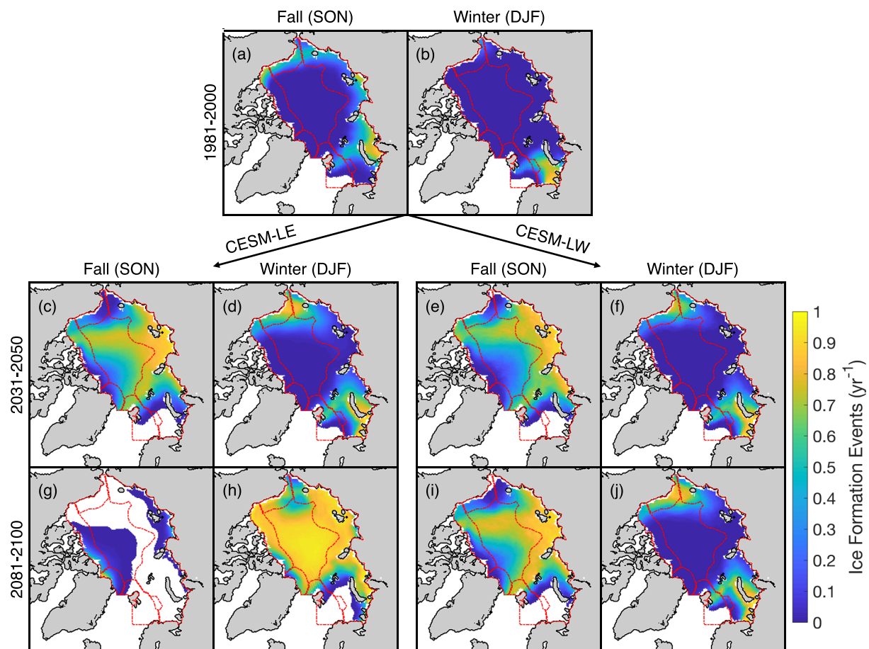
Figure 5. Average number of ice formation events per year in fall (SON) and winter (DJF) for the CESM-LE over the period of 1981–2000 (a, b) and for the CESM-LE (c, d, g, and h) and the CESM-LW (e, f, i, and j) over the periods of 2031–2050 (c–f) and 2081–2100 (g–j). Only grid cells that are ice covered for at least 1 month during the specified season and time period and for a least one ensemble member are colored. The borders of the EEZs are indicated by red lines. Only ice floes that formed and melted between the specified time periods are considered.
