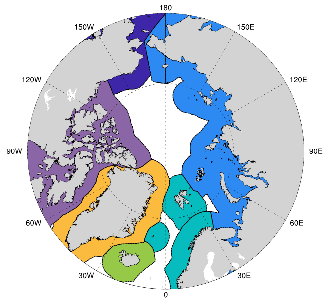
Figure 1. Map of the exclusive economic zones (EEZs) of the Arctic based on the definition from the United Nations Convention on the Law of the Sea (Nordquist, 2011): Canada (purple), the United States (dark blue), Russia (light blue), Norway (turquoise), Iceland (green), and Greenland (orange). The region in the middle of the Arctic Ocean that is not included within an EEZ is referred to as the Central Arctic (CNT) for the context of this study.
