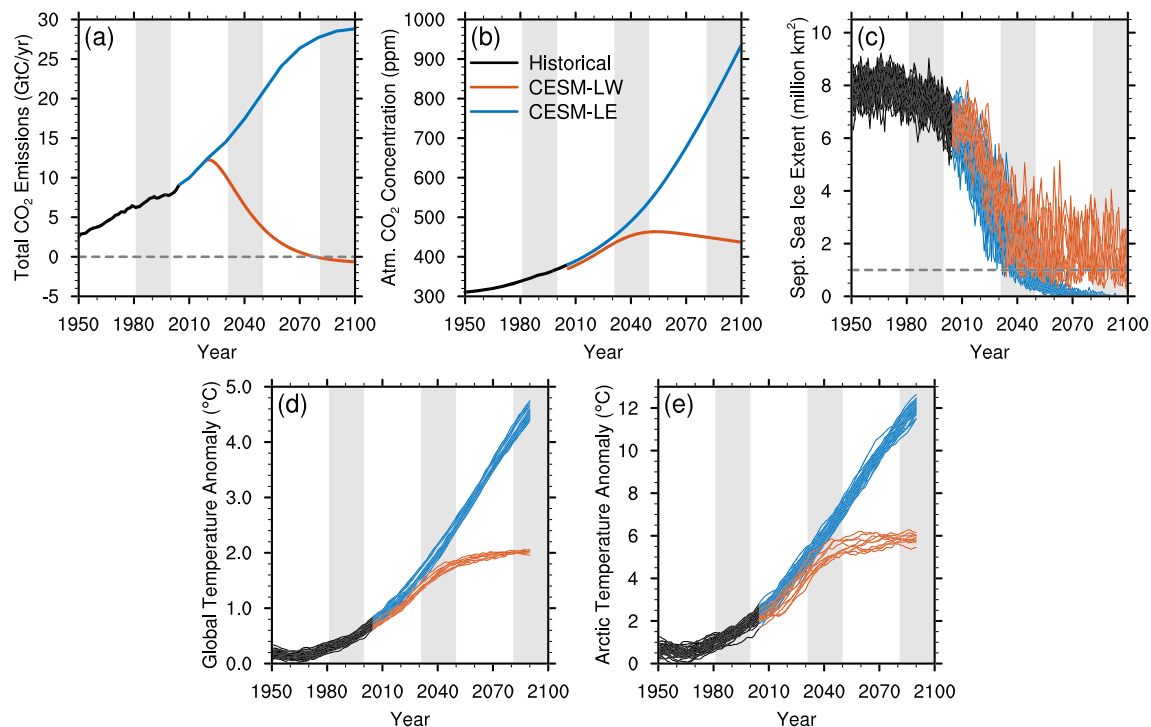
Figure 2. Time evolution of (a) the total CO 2 emissions in GtC/yr, (b) the atmospheric CO 2 concentration in ppm, (c) the September Arctic sea ice extent in million square kilometers for all ensemble members with the threshold for a nearly ice-free Arctic shown by the gray dashed line, (d) the 20-year running mean annual mean global temperature anomalies for all ensemble members (relative to preindustrial levels, taken as 1850–1920 here), and (e) the 20-year running mean annual mean Arctic temperature anomalies for all ensemble members. All panels cover the historical period of the CESM-LE (black), the future RCP8.5 scenario of the CESM-LE (blue), and the future low warming scenario of the CESM-LW (orange). Note the different range of the y axis for (d) the global temperature anomalies and (e) the Arctic temperature anomalies. The gray shaded areas highlight the three different time periods our analysis focuses on (adapted from Figure S1 of Jahn, 2018).
