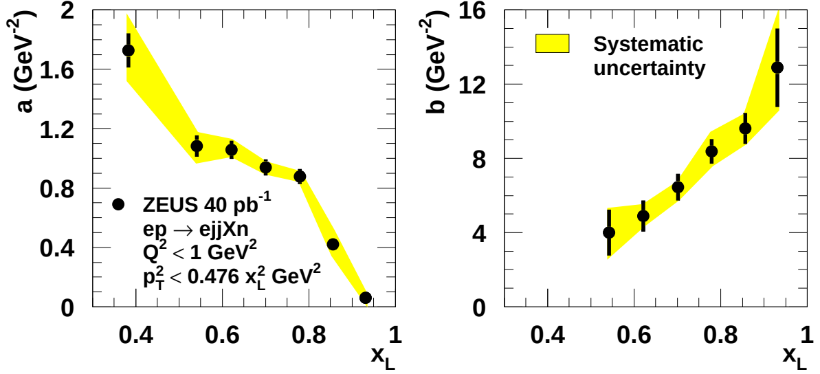
Figure 8: Intercepts a and exponential slopes b versus x_L from fits of the p_T^2 distributions to the form (1/\sigma_{ep \rightarrow ejjXn}) d^2\sigma_{ep \rightarrow ejjXn}/dx_L dp_T^2 = a \exp(-bp_T^2) over the range p_T^2 < 0.476x_L^2 \text{ GeV}^2 . The error bars show the statistical uncertainties; the shaded bands show the neutron-related systematic uncertainties. The band for the intercepts does not include the overall normalization uncertainty of \pm 2.1\% .
