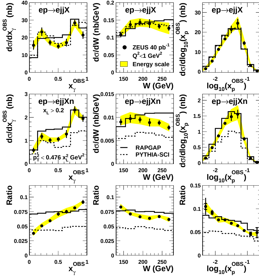
Figure 3: Differential neutron-tagged and untagged dijet photoproduction cross sections as functions of x_\gamma^{\text{OBS}} , W and \log_{10}(x_p^{\text{OBS}}) . The ratios between cross sections, the neutron yields, are also given. Details are as in Fig. 2.
