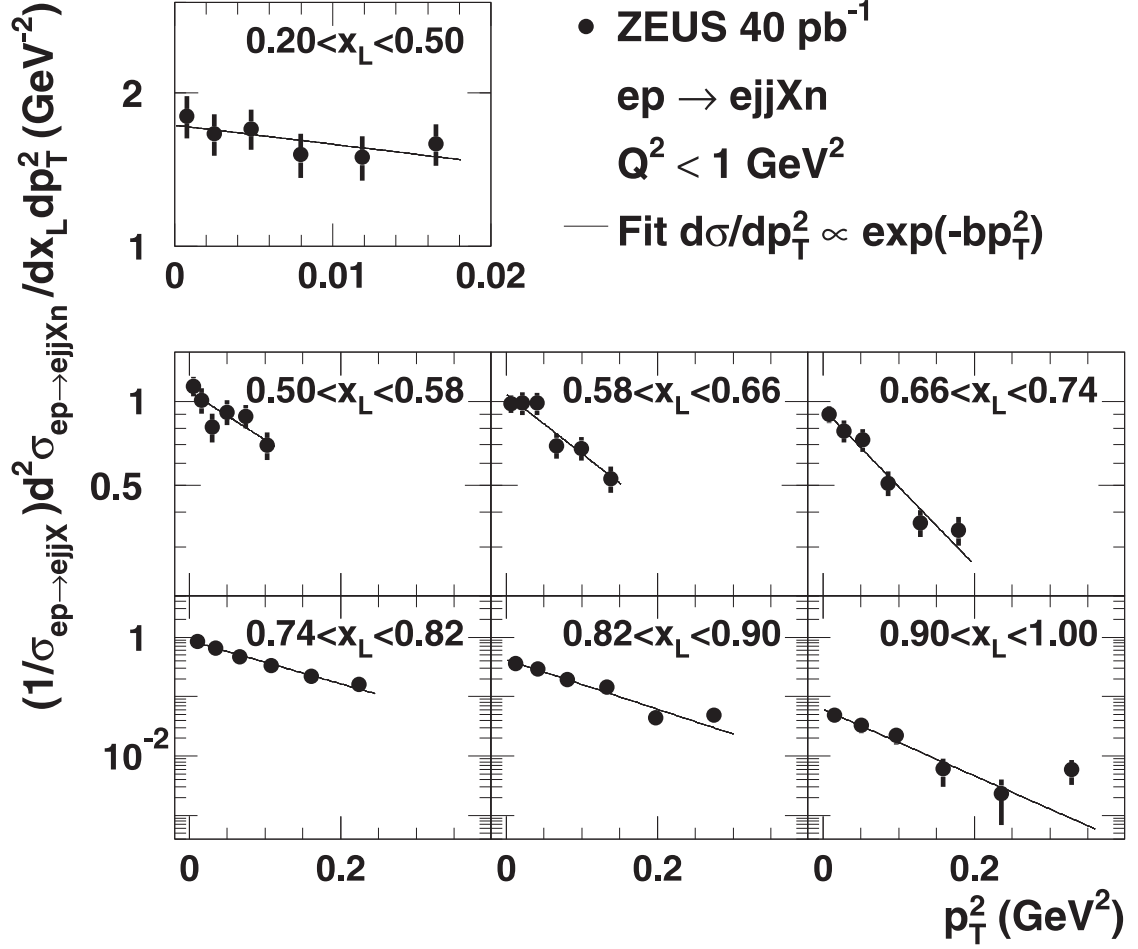
Figure 7: The p_T^2 distributions in bins of x_L . The statistical uncertainties are shown by vertical error bars; in some cases they are smaller than the plotted symbol. The systematic uncertainties are not shown. The line on each plot is the result of a fit to the form d\sigma_{ep \rightarrow ejjXn}/dp_T^2 \propto \exp(-bp_T^2) .
