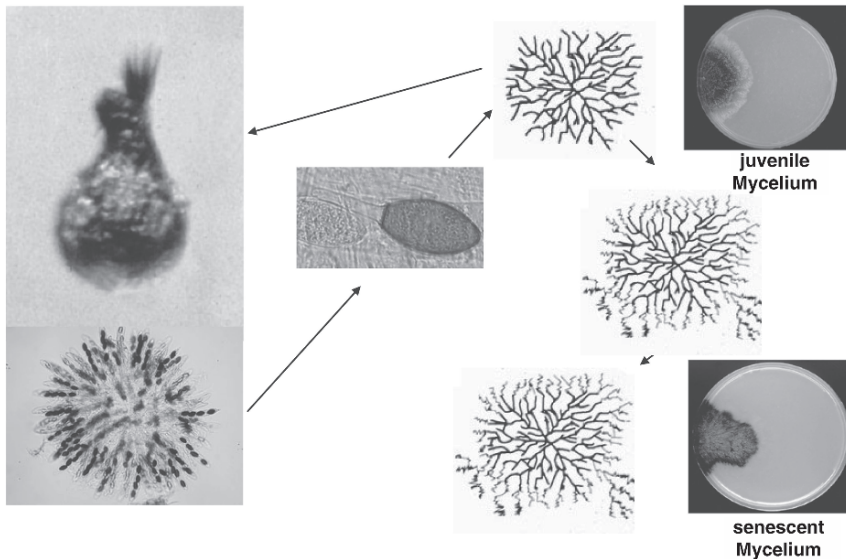
Fig. 4.1 Propagation and senescence of the filamentous ascomycete P. anserina . ( Left ) Fruiting bodies, termed perithecia, contain the products of sexual reproduction, the ascospores. After germination of an ascospore ( middle ) a mycelium is formed. Juvenile mycelia are characterized by aerial hyphae and regular growth. In the senescent stage, pigmentation increases and formation of aerial hyphae is strongly reduced. Mycelial tips swell and burst. Eventually, the mycelium stops growth completely and dies ( right )
