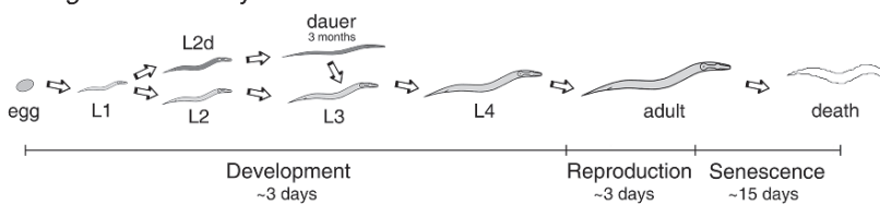
Fig. 6.2 C. elegans life history. This is broadly divisible into embryonic and larval development, reproduction, and senescence. Larval development has four stages of growth (e.g., L1, larval stage 1). Total life span is a mere 3 weeks at 20°C ( C. elegans life span is dependent on ambient temperature). Typically, life span measurements represent adult life span only, the mean being approximately 18 days. In contrast, at the L2 stage, larvae can enter an alternative, dormant state known as dauer. Dauer larvae can survive for at least 3 months without food, essentially a fourfold increase in longevity. After exposure to a food source, dauer larvae resume development and subsequently reproduce and senesce as normal
