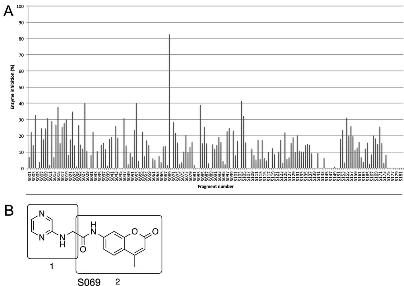
Fig. 2. Fragment library screening. Screening of 182 fragment-sized N -7-amino-4-methylcoumarines as potential Atg4B inhibitors. Compounds were screened using the earlier described SDS-PAGE-based inhibitor screening. A, overview of screening results. Enzyme inhibition was expressed per fragment (see Table S1 in supporting information for exact values). B, fragment structure of S069, identified as a weak Atg4B inhibitor. 1, active fragment residue, a 2-methylaminopyrazine substituent. 2, N -acyl 7-amino-4-methylcoumarin fragment, core structure shared by all fragments.
