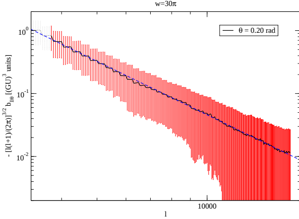
FIG. 7: Mean value and standard deviation of the squeezed bispectrum [\ell(\ell+1)/(2\pi)]^{3/2} b_{\ell\ell\theta} for \theta = 0.2 radians. The window function width has been increased to w = 30\pi to reduce the variance pushing up the lower multipole cutoff to \ell_{\min} = w/(\theta_{\text{fov}}\theta) \simeq 3750 . The dashed line is the best power law fit whose power has been set to the one obtained from the equilateral configuration [see Eq. (84)].
