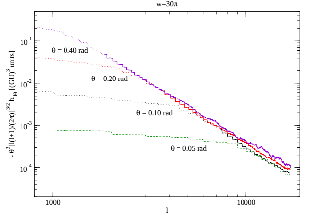
FIG. 8: Rescaled mean squeezed bispectrum \theta^3[\ell(\ell+1)/(2\pi)]^{3/2} b_{\ell\ell\theta} showing the 1/\theta^3 dependency. Notice the large window function width w = 30\pi chosen to reduce the statistical errors and pushing up the numerical multipole cutoff \ell_{\min} .
