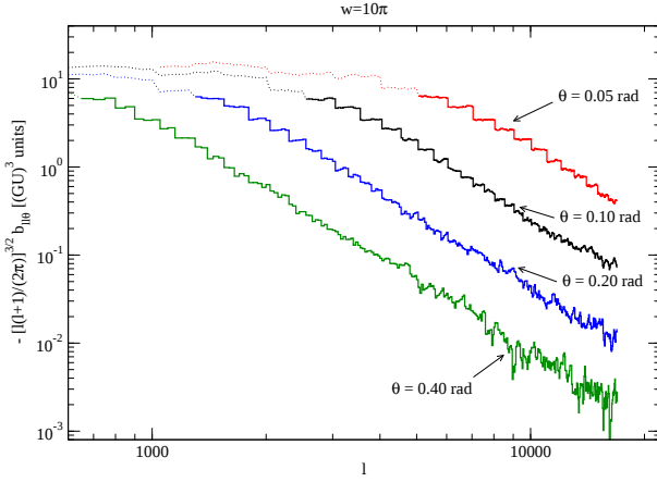
FIG. 6: Squeezed angle dependency of the mean squeezed bispectrum [\ell(\ell+1)/(2\pi)]^{3/2} b_{\ell\ell\theta} . The spurious plateau (dotted lines) for the lower multipoles comes from the cutoff associated with a given squeezed angle \theta together with the window function width w and occurs at \ell_{\min} = w/(\theta_{\text{fov}}\theta) .
