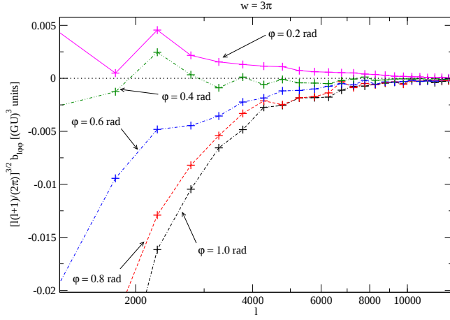
FIG. 9: Mean collapsed bispectrum [\ell(\ell+1)/(2\pi)]^{3/2} b_{\ell\varphi\varphi} . This configuration is extremely sensitive to the window function properties and statistical errors dominate. The change of sign for small values of \varphi is nevertheless observable.
