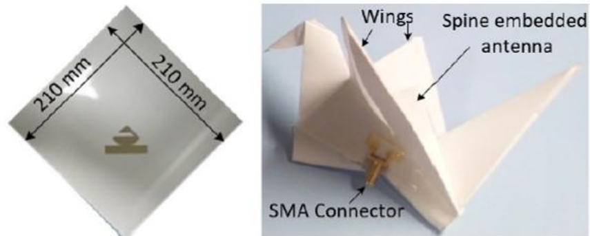
Figure 12. Left: unfolded structure showing at the center the antenna printed on photo paper using silver ink. Right: folded origami bird-like structure, fed by a coaxial connector on the spine. Reproduced from [88] under a Creative Commons Attribution 4.0 License by IEEE. For more information, see https://creativecommons.org/licenses/by/4.0/ .
