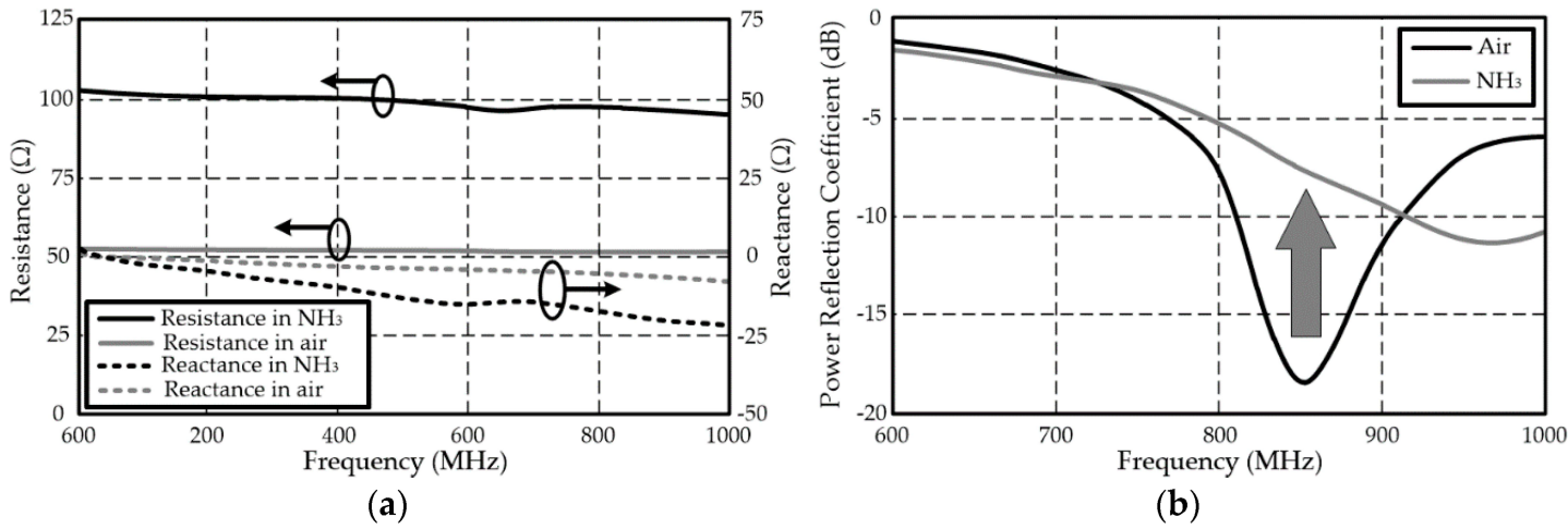
Figure 10. (a) measured impedance of the RFID tag including an inkjet-printed CNT film in the presence of air and \text{NH}_3 gas (b) reflection coefficient in the presence of air and \text{NH}_3 , Reprinted from [10] under CC BY 4.0 license by MDPI.
