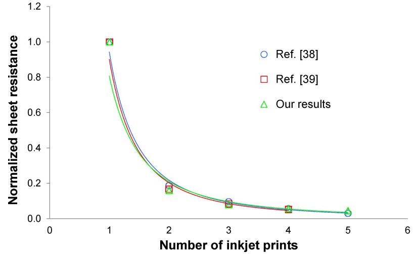
Figure 2. Normalised sheet resistance according to [26]. Reproduced under the Creative Commons Attribution Non-Commercial License by MDPI.
