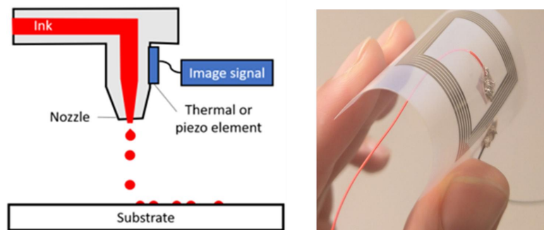
Figure 3. Left: Schematic representation of IJP process. Right: printed RFID coil. Reprinted from [62] under the terms and conditions of the Creative Commons Attribution (CC BY) license ( https://creativecommons.org/licenses/by/4.0/ ).
