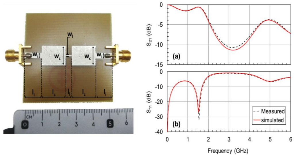
Figure 4. Stepped impedance low-pass filter having 5 sections. Left: photo and dimensions of the filter. Right: measured and simulated performance. (a) transmission (b) reflection. Reprinted from [4] under the terms and conditions of the Creative Commons Attribution (CC BY) license ( https://creativecommons.org/licenses/by/4.0/ ).
