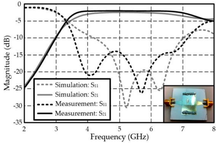
Figure 9. Microstrip-to-SIW transition inkjet printed on a paper substrate using silver ink. The transition consists of two triangular tapered strips connecting the coaxial connectors to the input and output of the rectangular SIW. Reprinted from [10] under CC BY 4.0 license by MDPI.
