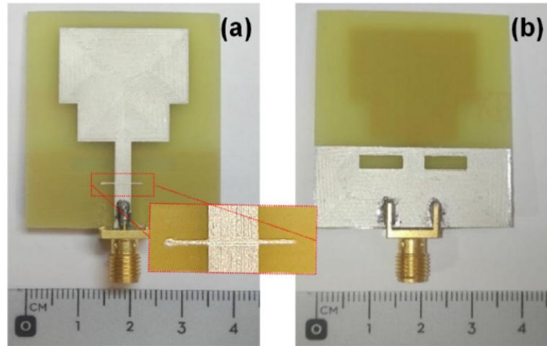
Figure 6. Stepped-type monopole antenna (a) top view (b) bottom view. Reprinted from [4] under the terms and conditions of the Creative Commons Attribution (CC BY) license ( https://creativecommons.org/licenses/by/4.0/ ).
