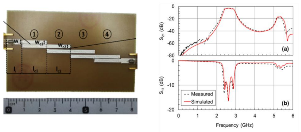
Figure 5. Left: Coupled line bandpass filter. Left: photo and dimensions of the filter containing 4 coupled sections. Right: measured and simulated performance (a) transmission (b) reflection. Reprinted from [4] under the terms and conditions of the Creative Commons Attribution (CC BY) license ( https://creativecommons.org/licenses/by/4.0/ ).
