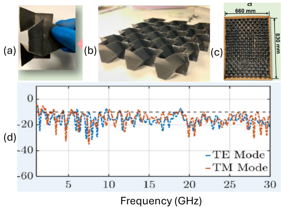
Figure 13. Origami-based absorber structure (a) hand-folding of the structure (b) perspective view of the folded structure (c) top view of the absorber prototype (d) reflectivity measurement. Reproduced and adapted from [90] under a Creative Commons Attribution 4.0 International License by Springer. For more information, see https://creativecommons.org/licenses/by/4.0/ .
