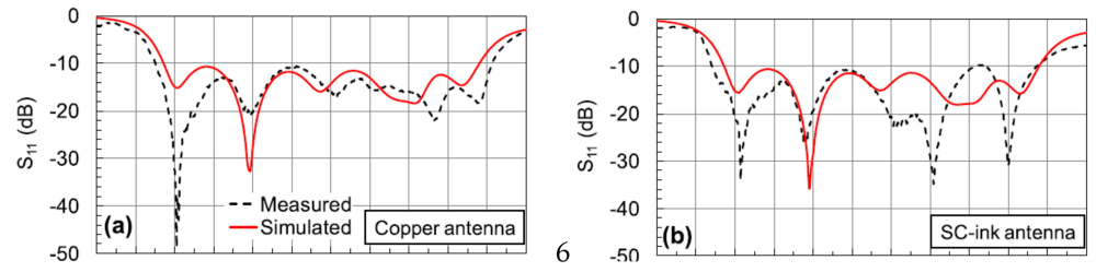
Figure 7. Simulated and measured performance of stepped-type monopole antenna (a) copper prototype (b) Silver conducting (SC) ink prototype. Reprinted from [4] under the terms and conditions of the Creative Commons Attribution (CC BY) license ( https://creativecommons.org/licenses/by/4.0/ ).
