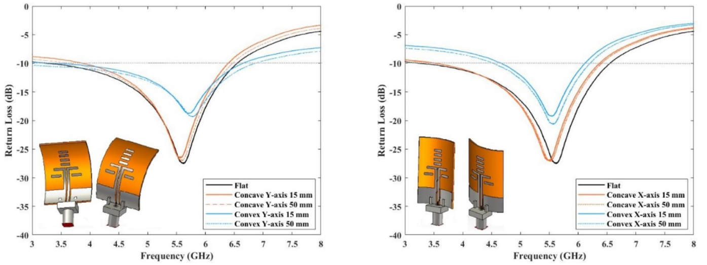
Figure 8. Left: return loss of the Yagi antenna under longitudinal bending. Right: return loss of the Yagi antenna under lateral bending. Reprinted from [72] under the terms of the Creative Commons Attribution 4.0 licence..
