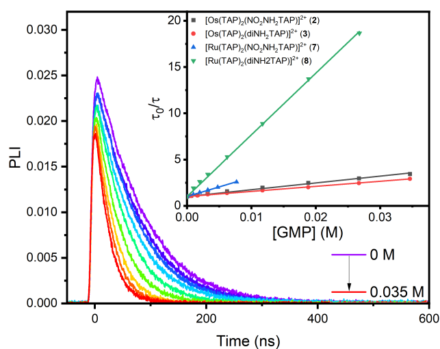
Figure 4. Time-resolved excited-state quenching of [\text{Os}(\text{TAP})_2(\text{NO}_2\text{NH}_2\text{TAP})]^{2+} and the corresponding Stern-Volmer plots of all photosensitizers undergoing excited-state quenching (inset). Experiments were performed in air-equilibrated tris HCl buffer (50 mM, pH = 7.4) at room temperature using 440 nm light excitation.
