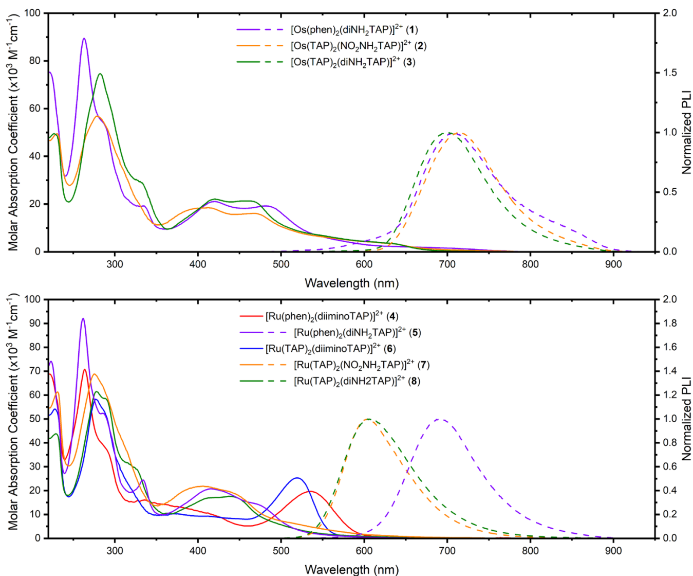
Figure 2. Absorption (solid) and photoluminescence (dashed) spectra of Os(II) (top) and Ru(II) (bottom) photosensitizers recorded in acetonitrile at room temperature under argon.
