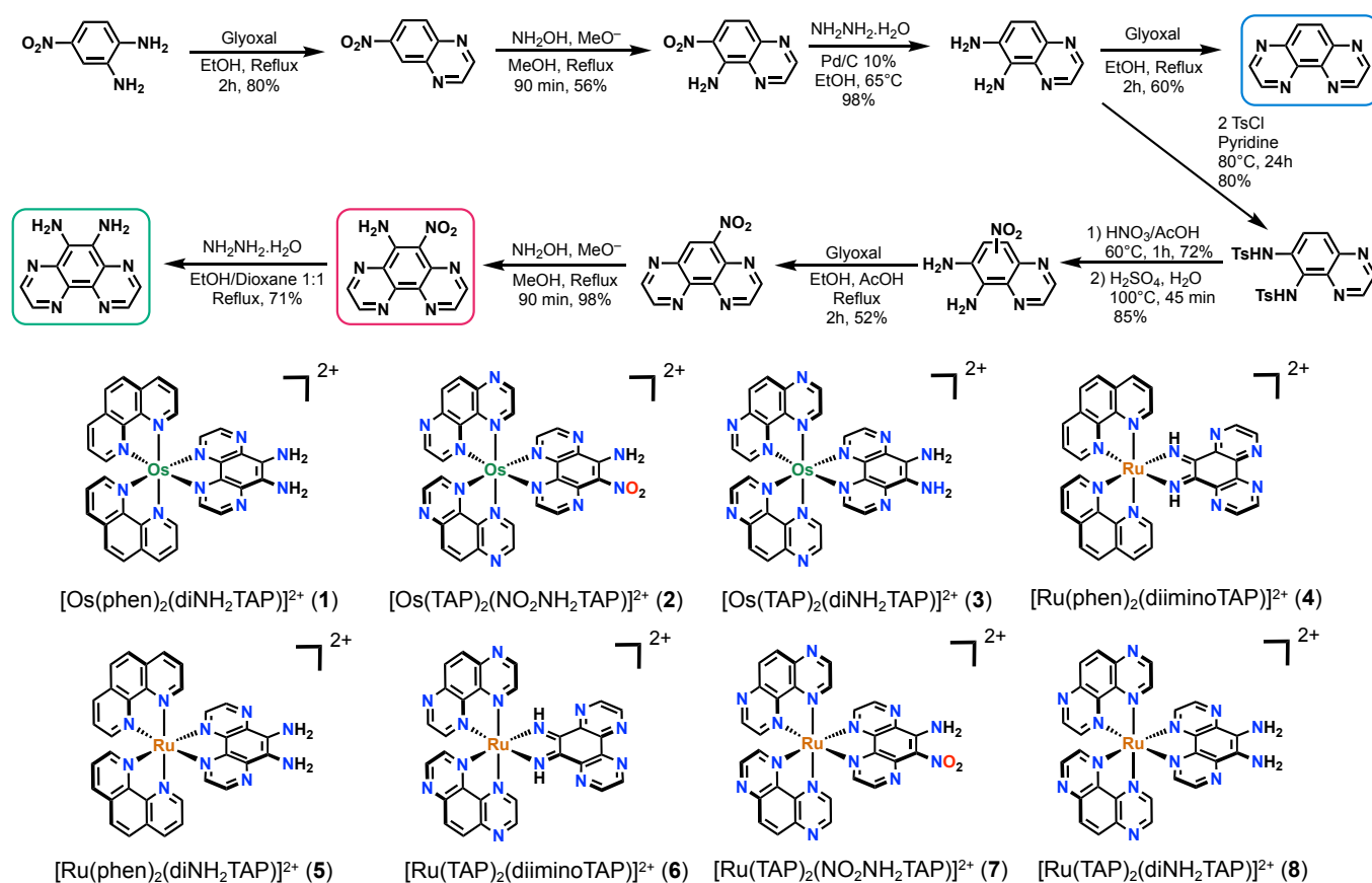
Figure 1. Synthesis scheme of 1,4,5,8-tetraazaphenanthrene (TAP), 9-amino-10-nitro-1,4,5,8-tetraazaphenanthrene (NO 2 NH 2 TAP) and 9,10-diamino-1,4,5,8-tetraazaphenanthrene (diNH 2 TAP) alongside the structures of the eight photosensitizers reported in the present study: [Os(phen) 2 (diNH 2 TAP)] 2+ (1), [Os(TAP) 2 (NO 2 NH 2 TAP)] 2+ (2), [Os(TAP) 2 (diNH 2 TAP)] 2+ (3), [Ru(phen) 2 (diiminoTAP)] 2+ (4), [Ru(phen) 2 (diNH 2 TAP)] 2+ (5), [Ru(TAP) 2 (diiminoTAP)] 2+ (6), [Ru(TAP) 2 (NO 2 NH 2 TAP)] 2+ (7), and [Ru(TAP) 2 (diNH 2 TAP)] 2+ (8).
