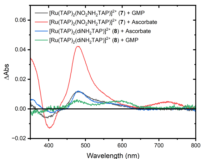
Figure 5. Transient absorption spectra of [\text{Ru}(\text{TAP})_2(\text{diNH}_2\text{TAP})]^{2+} and [\text{Ru}(\text{TAP})_2(\text{NO}_2\text{NH}_2\text{TAP})]^{2+} recorded in the presence of 20 mM of sodium ascorbate or with 10 mM of GMP. Spectra were recorded in argon purged tris-HCl buffer (50 mM, pH = 7.4) 1 \mu\text{s} after the laser pulse and integrated for 50 ns. Samples were excited at 440 nm with a laser fluence of 10 mJ/pulse.
