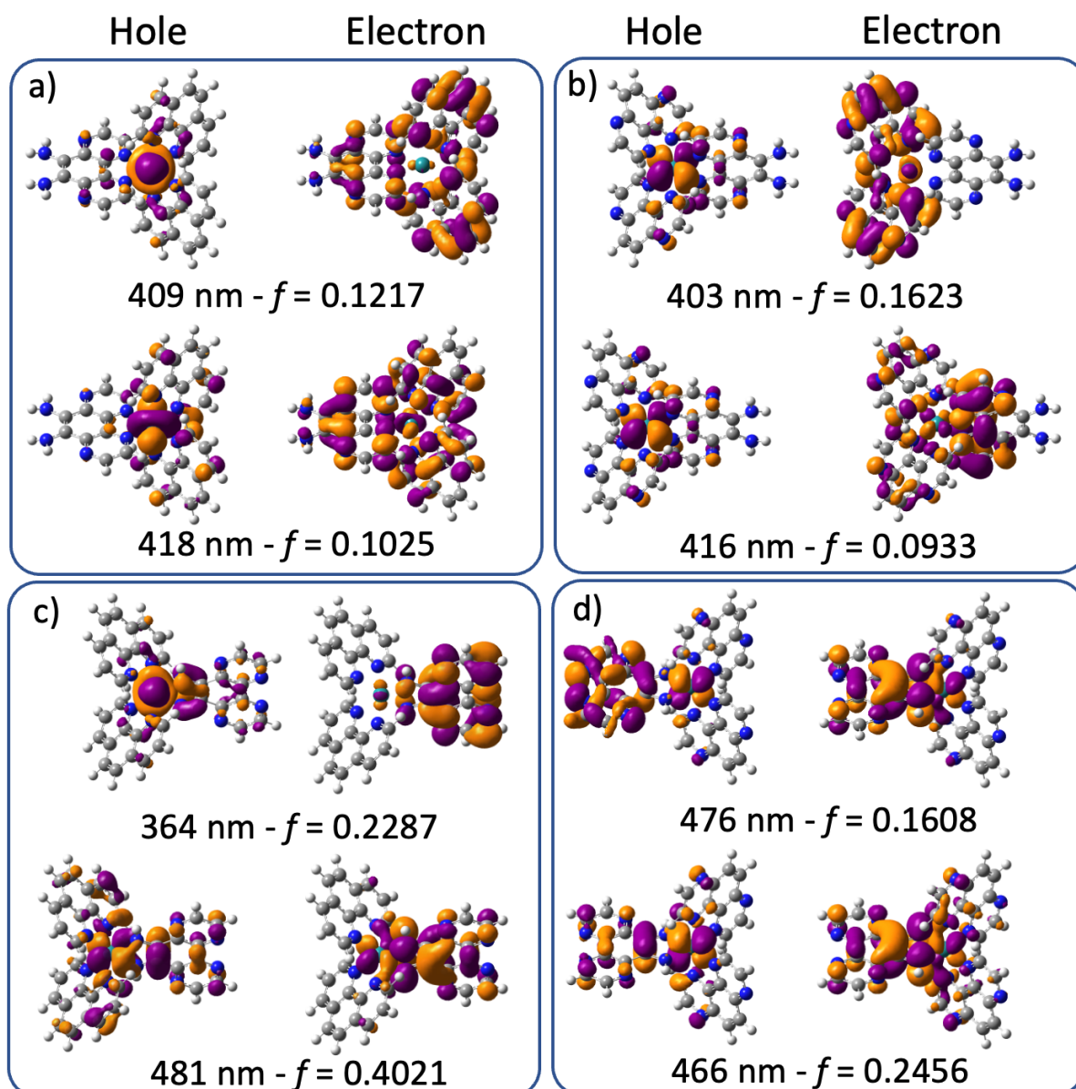
Figure 3. Natural Transition Orbitals (NTOs) for [\text{Ru}(\text{phen})_2(\text{diNH}_2\text{TAP})]^{2+} (a), [\text{Ru}(\text{TAP})_2(\text{diNH}_2\text{TAP})]^{2+} (b), [\text{Ru}(\text{phen})_2(\text{diiminoTAP})]^{2+} (c) and [\text{Ru}(\text{TAP})_2(\text{diiminoTAP})]^{2+} (d) involved in each excited state according to the TD-DFT calculations. For each excited state, absorption wavelengths (in nm) and calculated oscillator strengths ( f ) are listed. See supporting information for additional details on the theoretical calculations.
